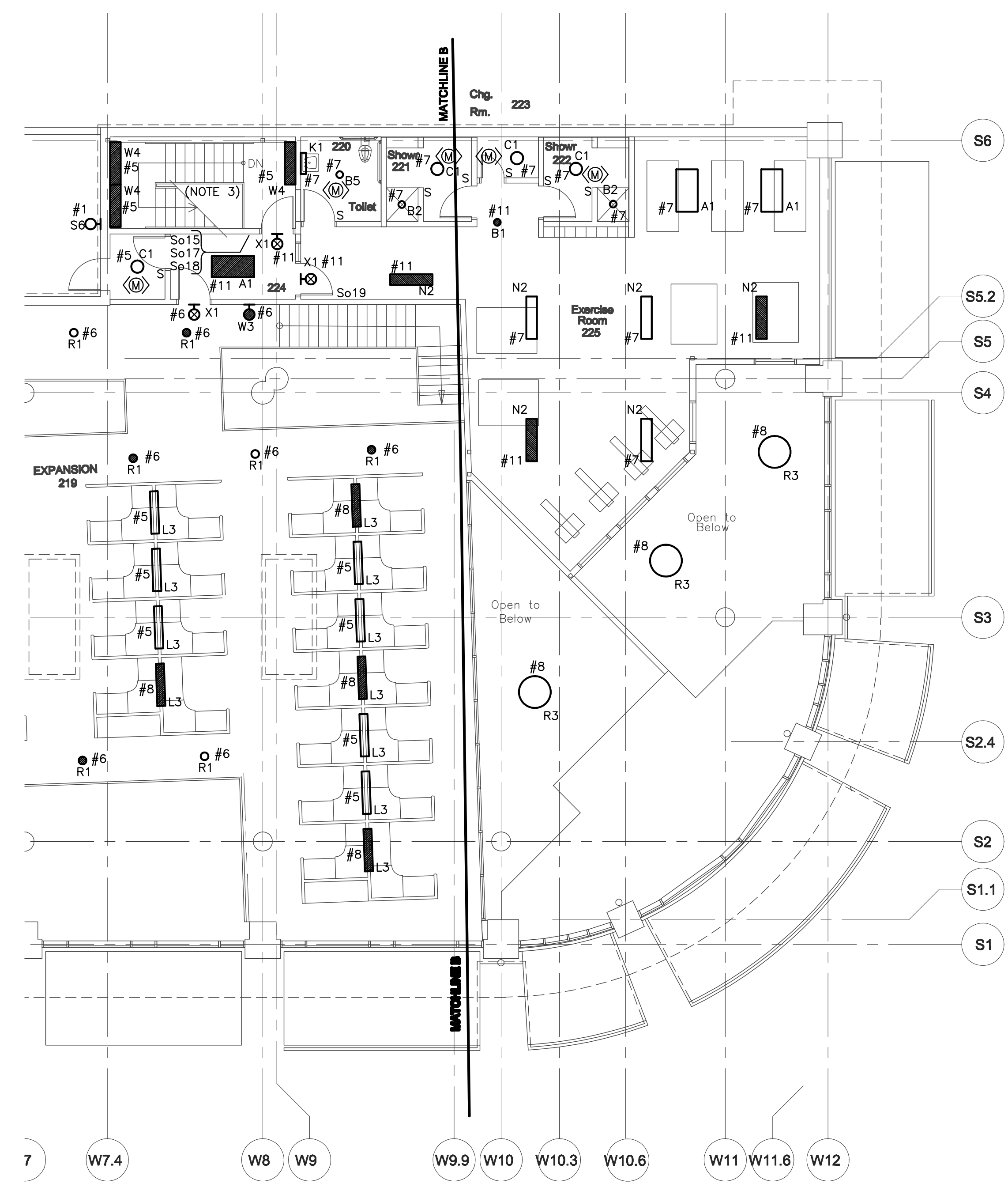
1 SECOND FLOOR LIGHTING PLAN - PART C E2.6 1/8" = 1'-0"
