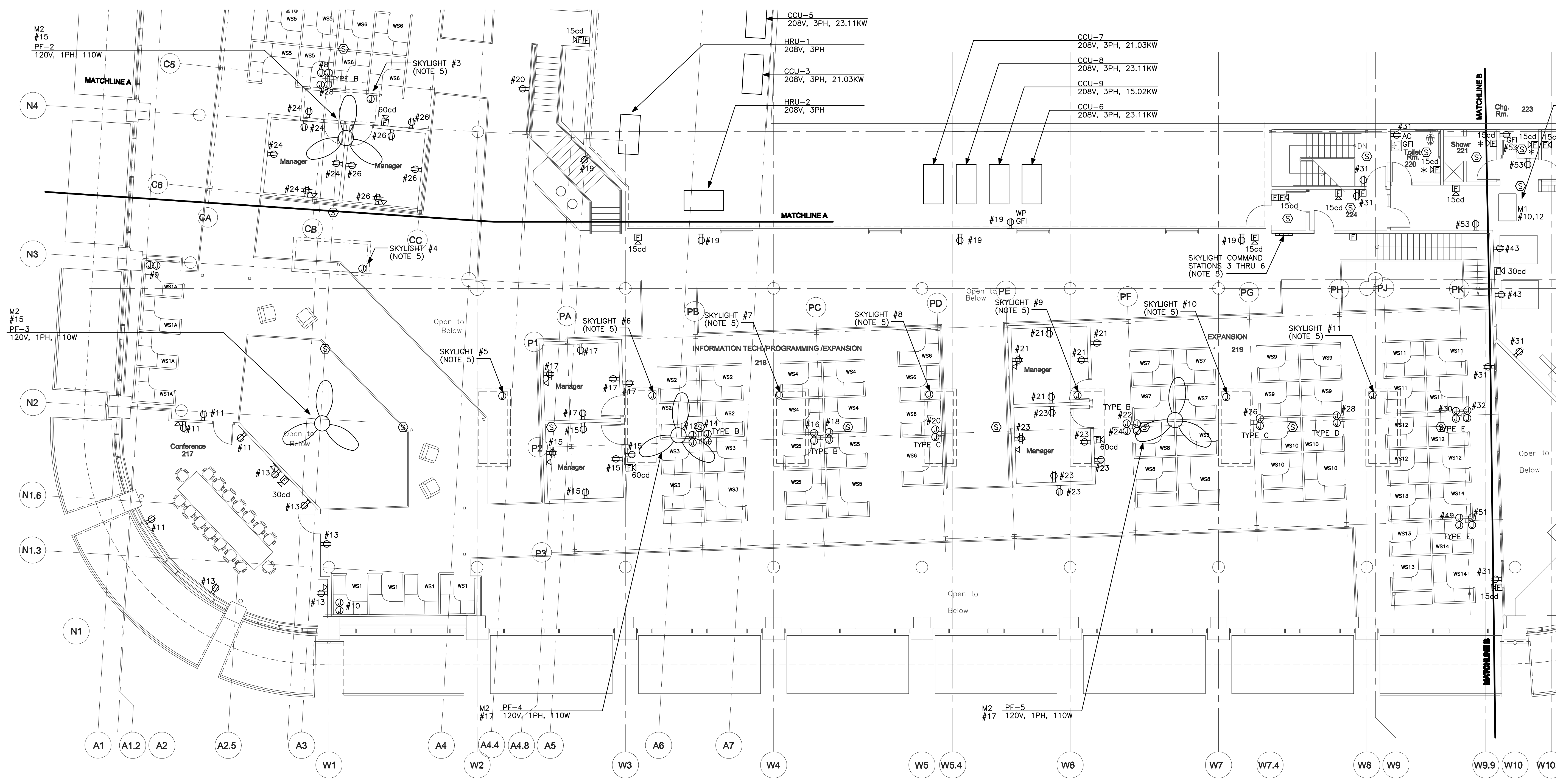
2 E1.5 SECOND FLOOR POWER PLAN - PART B 1/8" = 1'-0"
