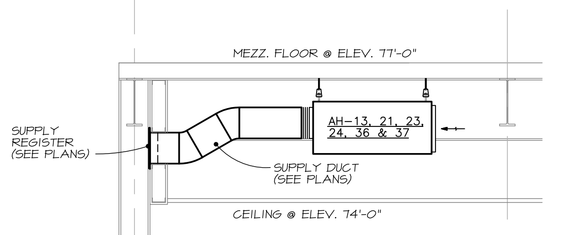
I SECTION AT AIR HANDLERS 13, 21, 23, 24, 36 & 37 SCALE: 1/2" = 1'-0"
