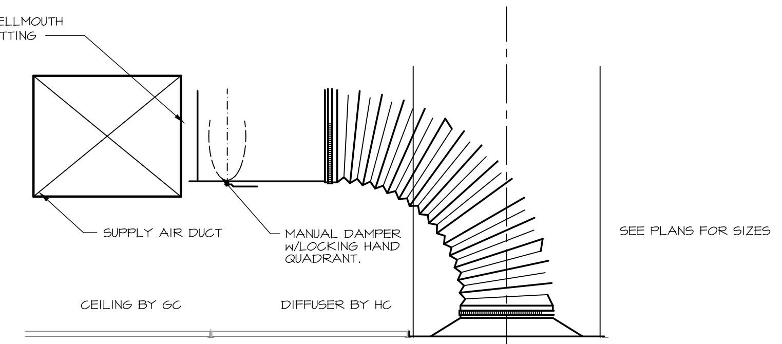
3 CONNECTION DETAIL NO SCALE
