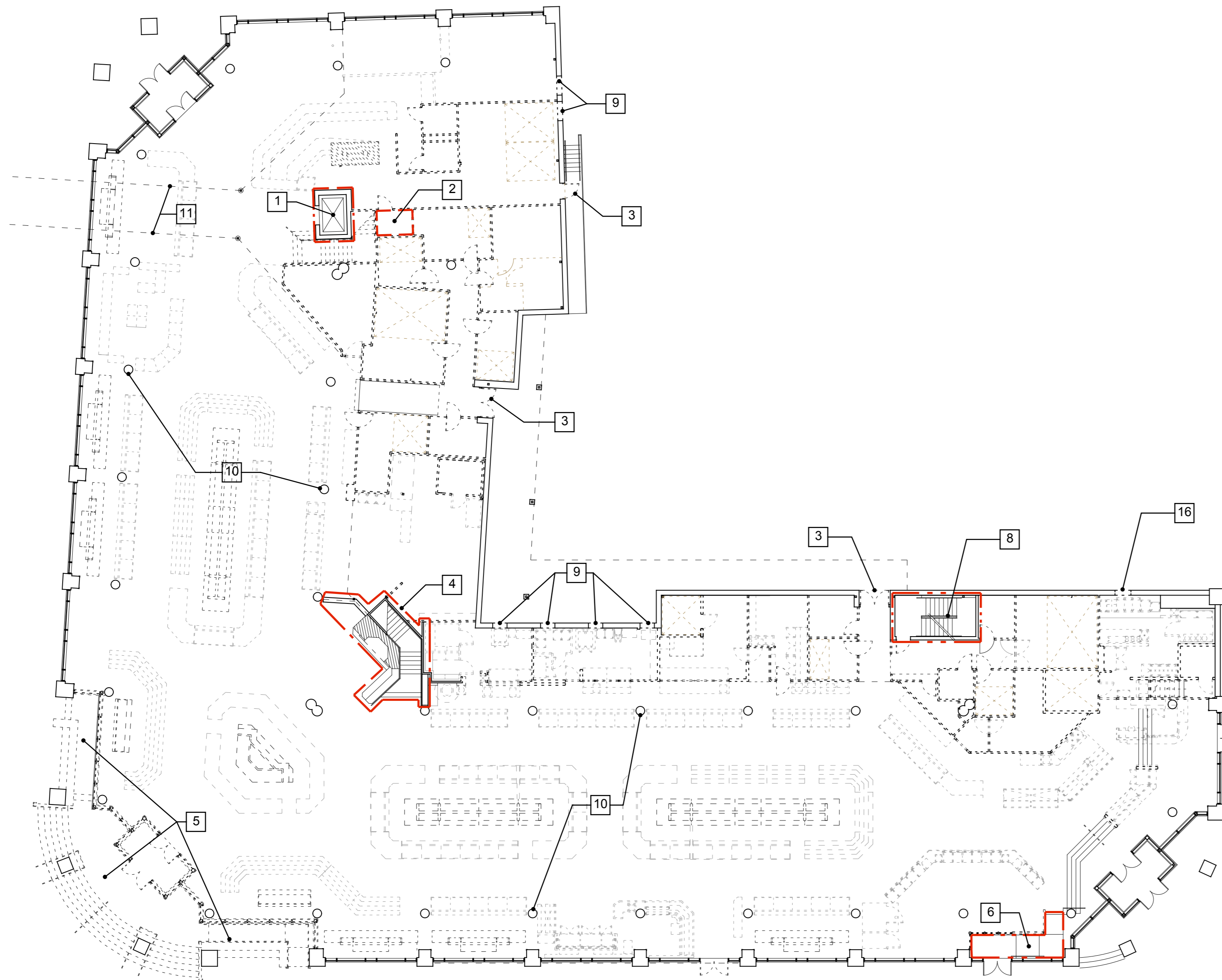
FIRST FLOOR DEMOLITION PLAN
