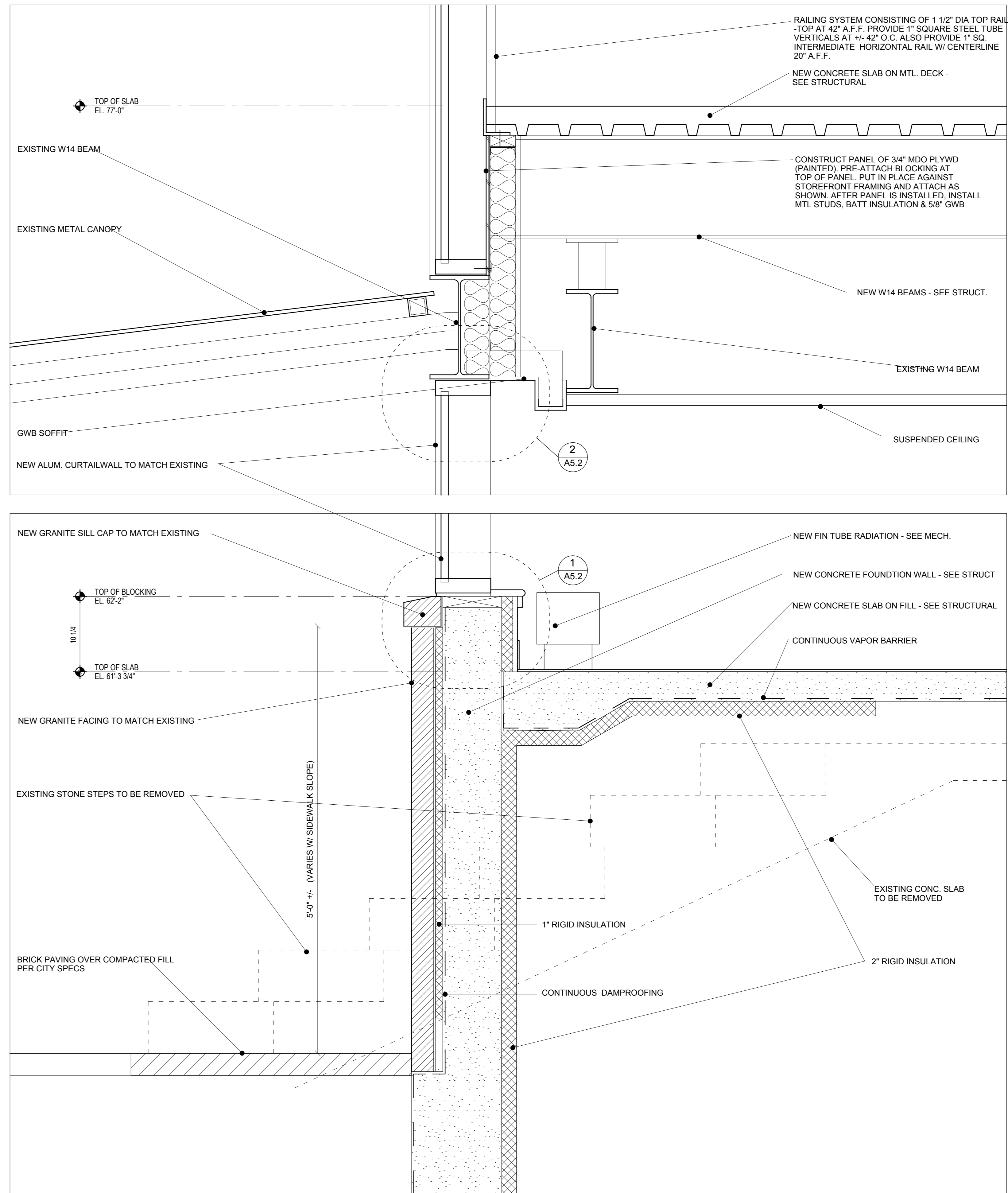
1 WALL SECTION DETAIL - at Corner Reconstruction 1 1/2" = 1'-0"
