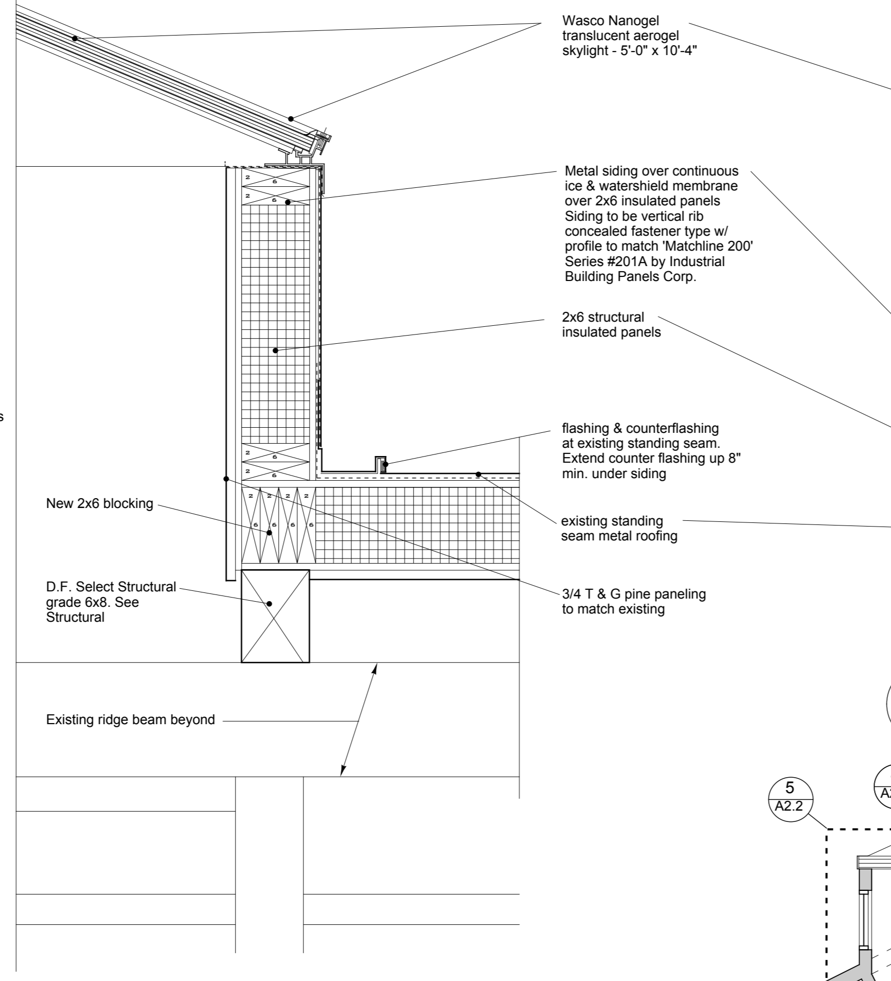
3 Skylight Curb Detail 1/2" Full Size
