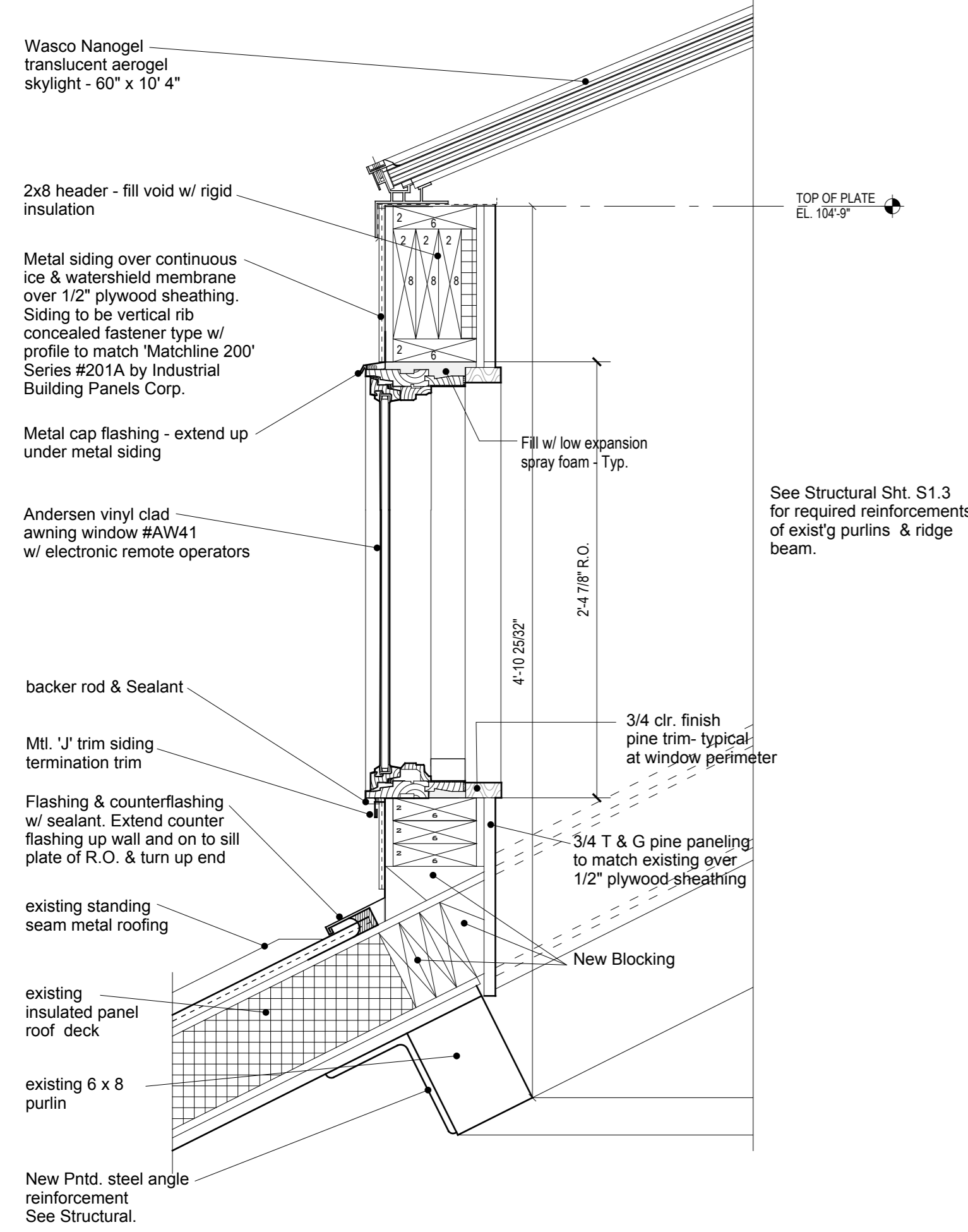
5 Skylight Curb Detail 1/2"=1'-0"
