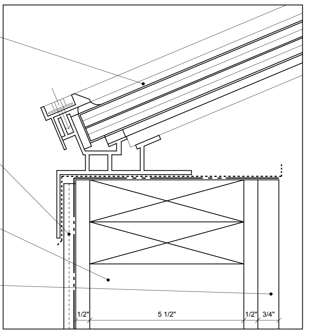
3 Skylight Curb Detail 1/2" Full Size
