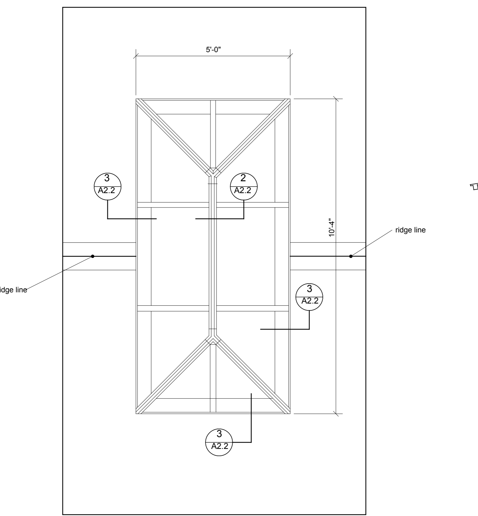
6 Skylight Roof Plan 1/2"=1'-0"
