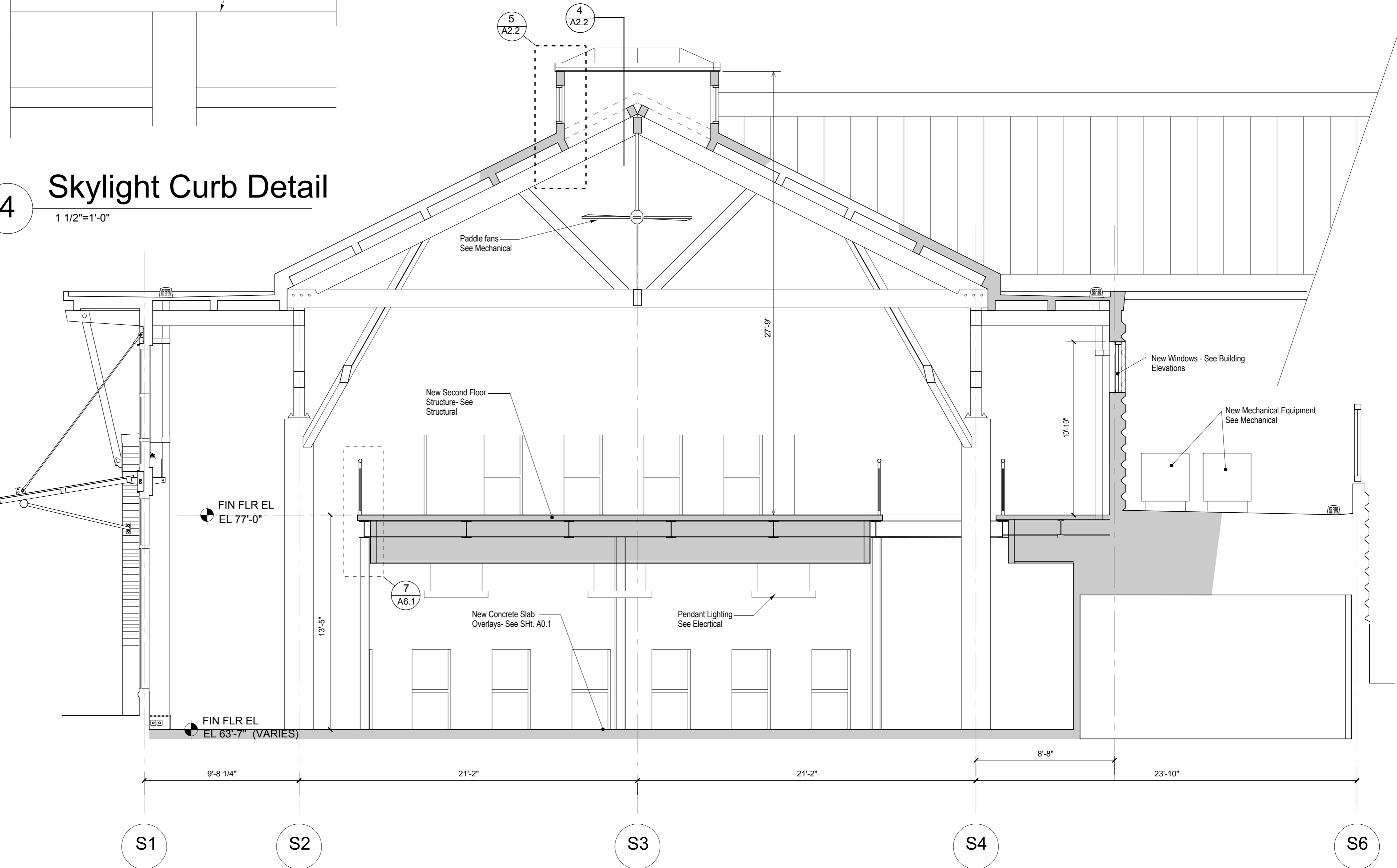
1 Building Section thru Skylight 1/4"=1'-0"
