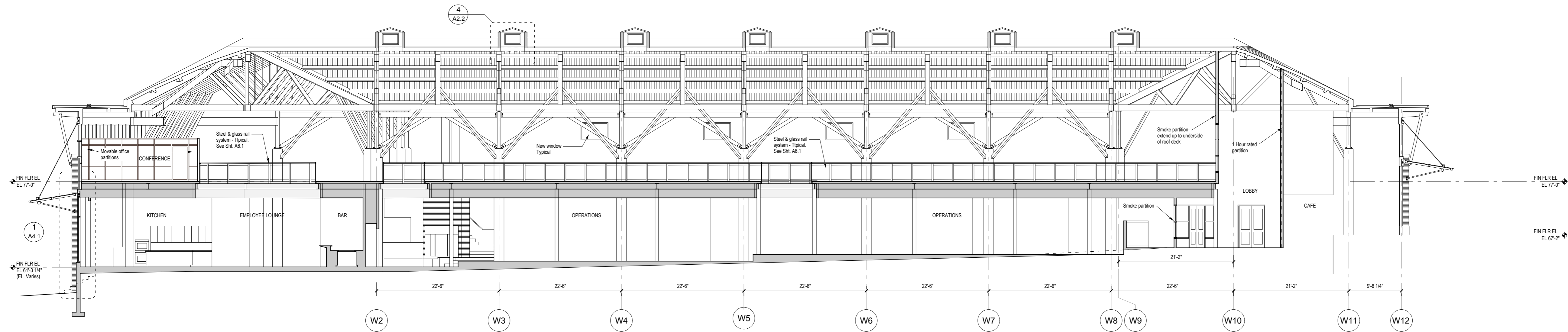
2 Building Section
