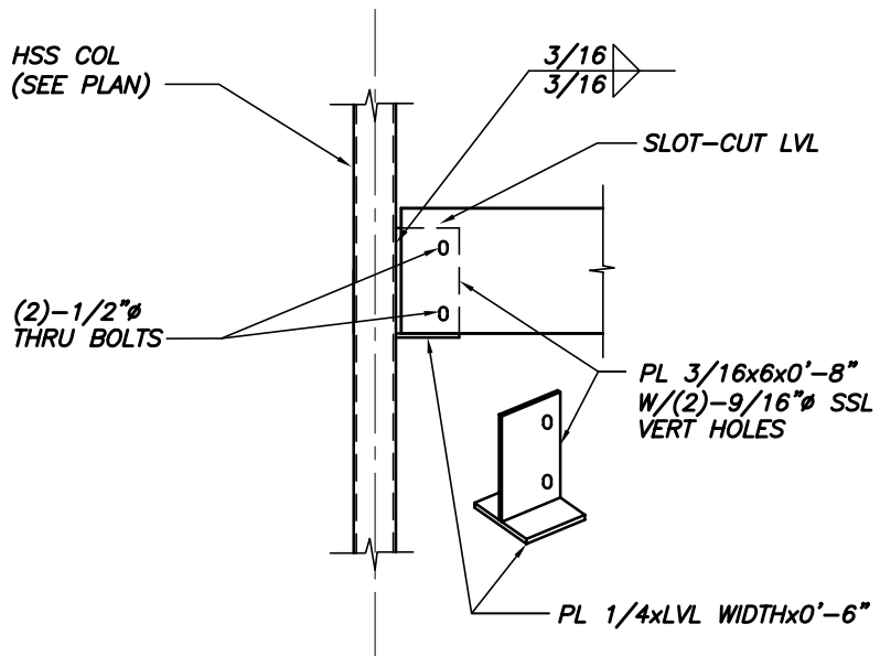
TYP HSS TO LVL DETAIL N.T.S.
