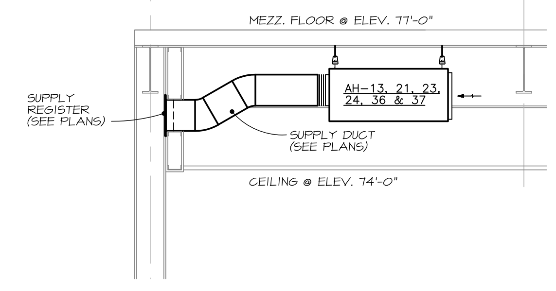
SECTION AT AIR HANDLERS 13, 21, 23, 24, 36 & 37 SCALE: 1/2" = 1'-0"
