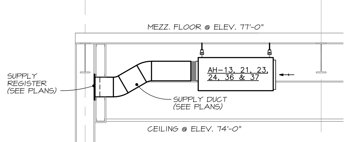
SECTION AT AIR HANDLERS 13, 21, 23, 24, 36 & 37 SCALE: 1/2" = 1'-0"
