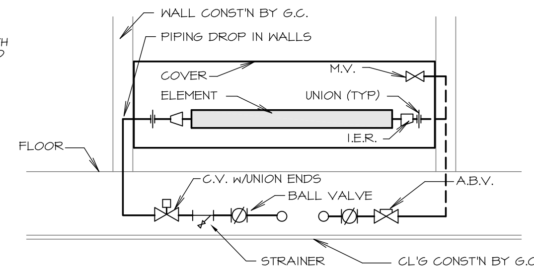
2 UPFEED FINNED PIPE OPPOSITE END FEED NO SCALE
