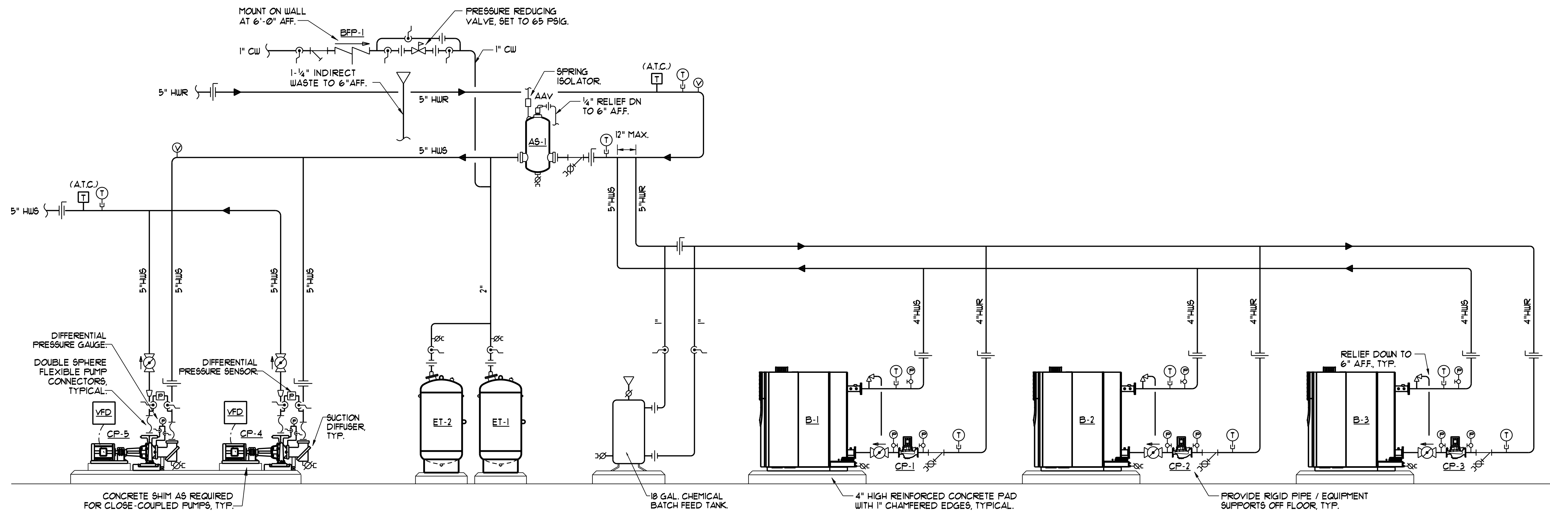
BOILER PIPING SCHEMATIC NTS
