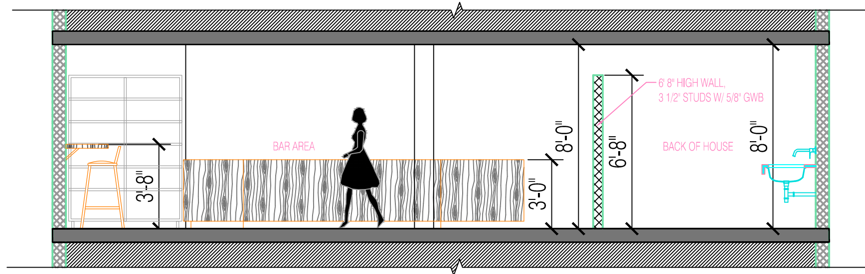
COFFEE BAR CROSS SECTION #####
