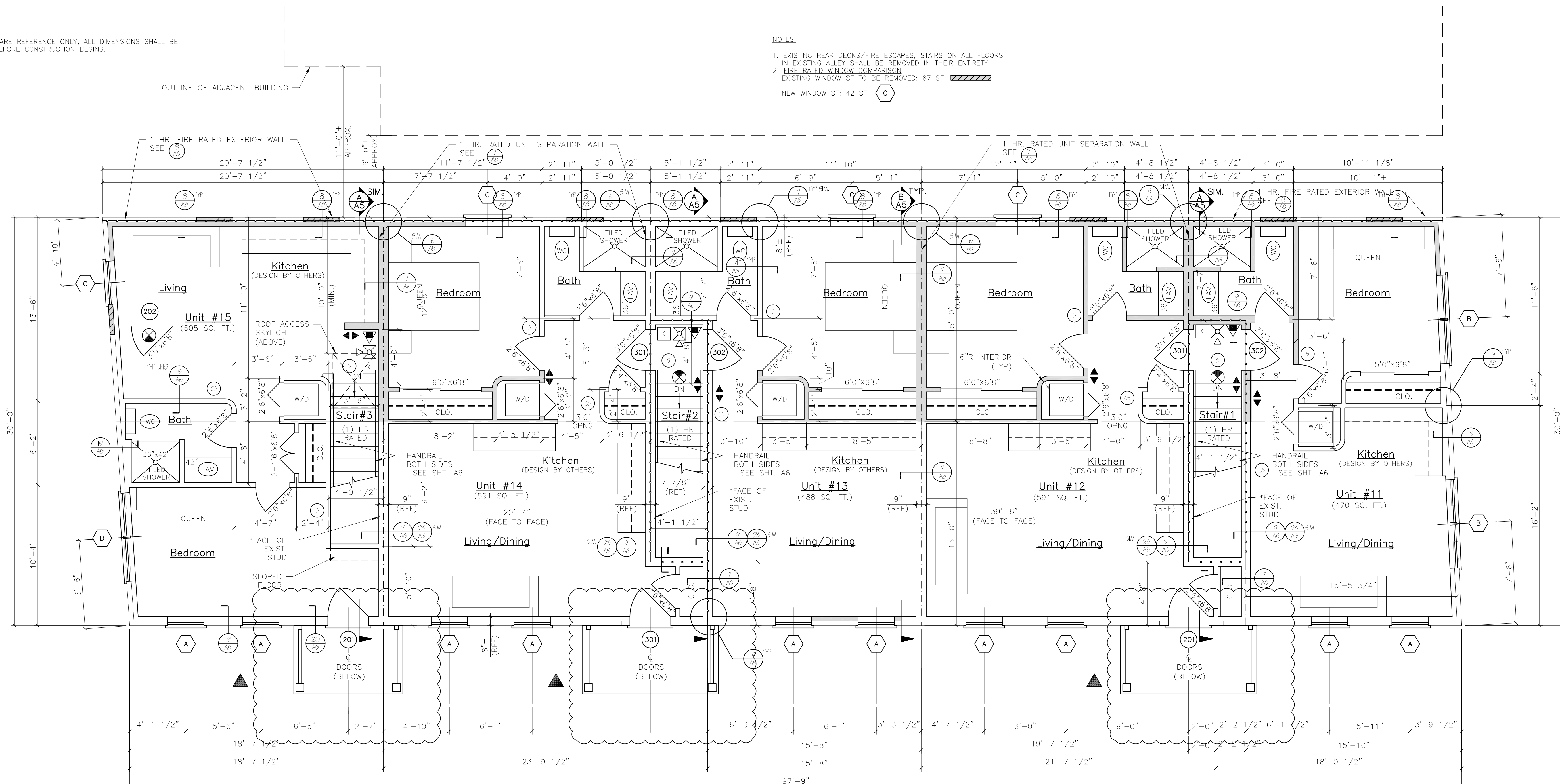
PROPOSED 3RD FLOOR PLAN
