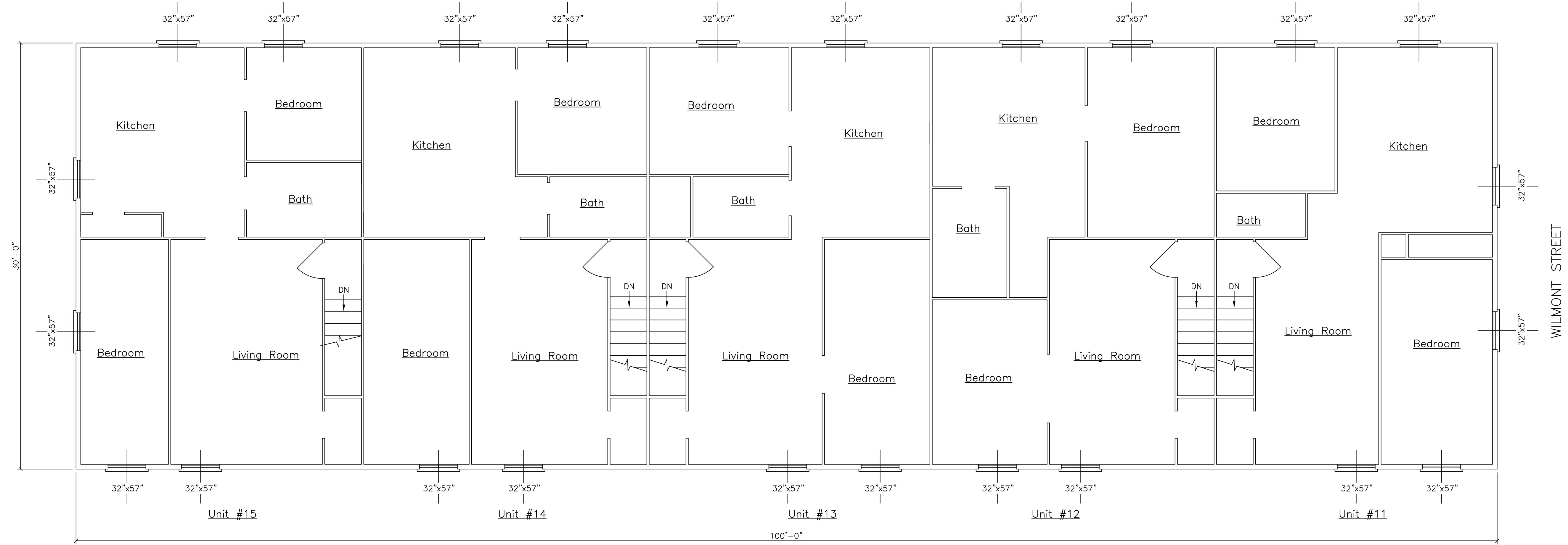
EXISTING 3RD FLOOR PLAN
