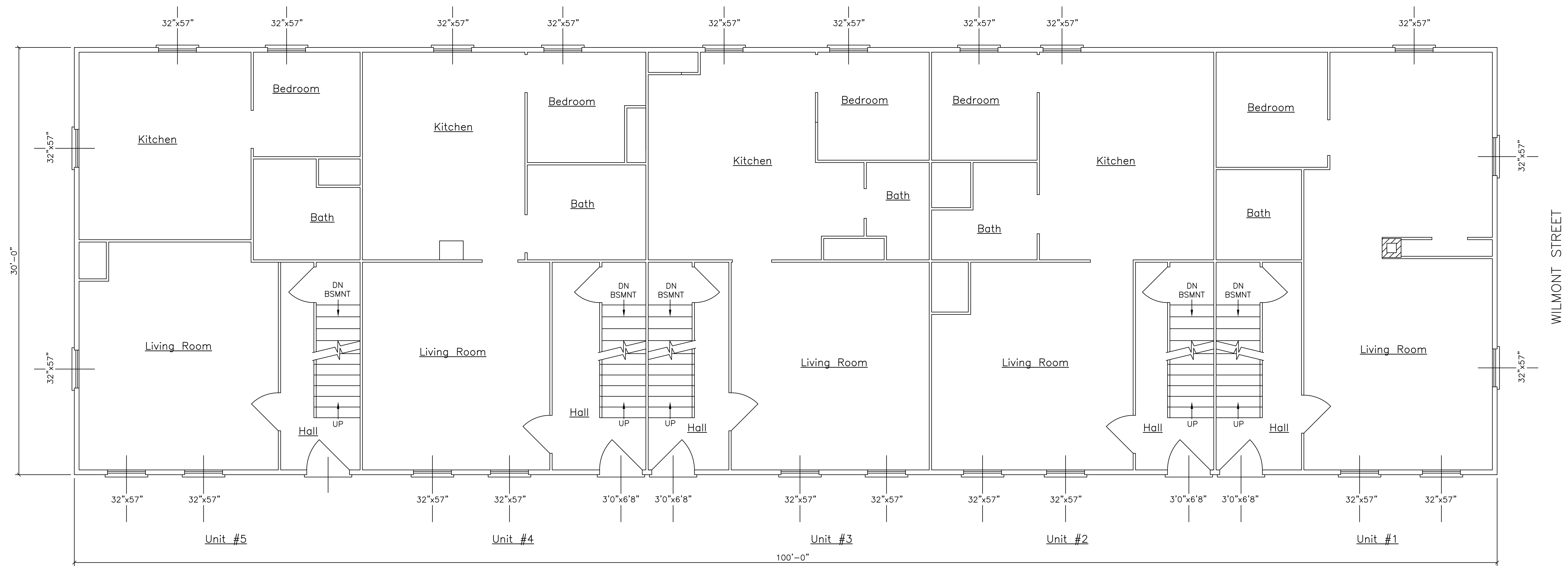
EXISTING 1ST FLOOR PLAN
