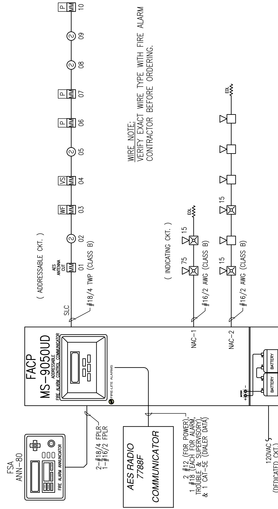
FIRE ALARM RISER DIAGRAM SCHEMATIC: NO SCALE
