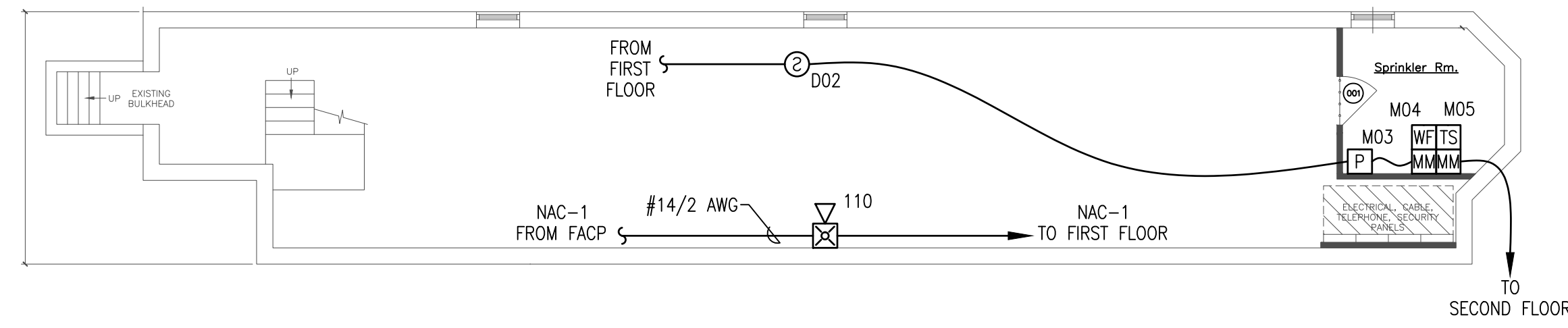
FIRE ALARM PLAN – BASEMENT PLAN SCALE: 1/8"=1'-0"
