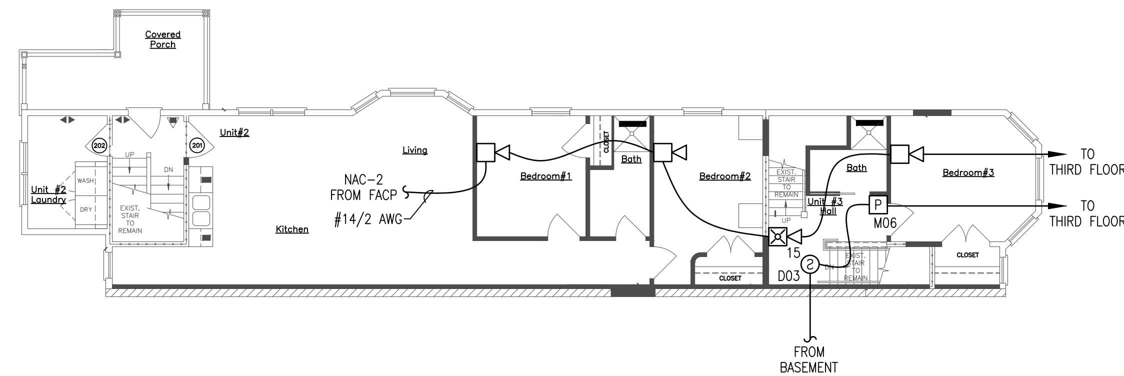
FIRE ALARM PLAN – SECOND FLOOR – UNIT 2 & 3 SCALE: 1/8"=1'-0"
