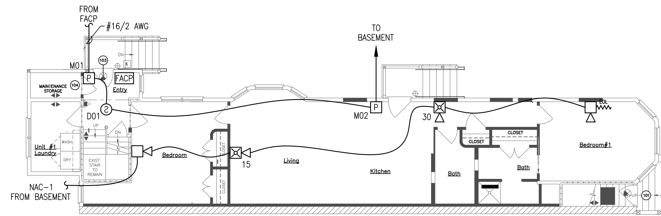
FIRE ALARM PLAN – FIRST FLOOR – UNIT 1 SCALE: 1/8"=1'-0"
