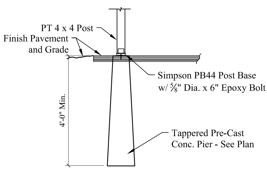
3 POST CONN. @ CONC. PIER Scale: 1/2" = 1'-0"
