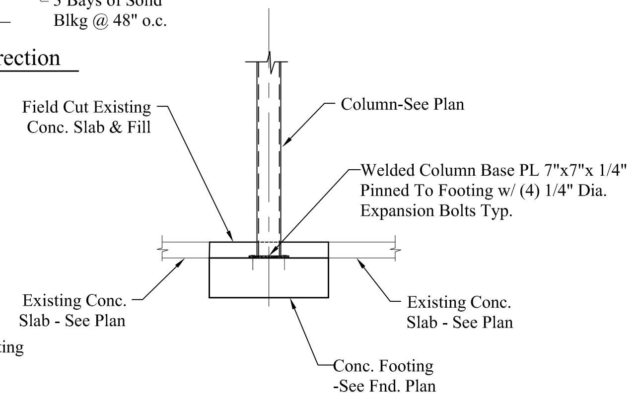
2 INTERIOR COLUMN FOOTING Scale: 1/2" = 1'-0"
