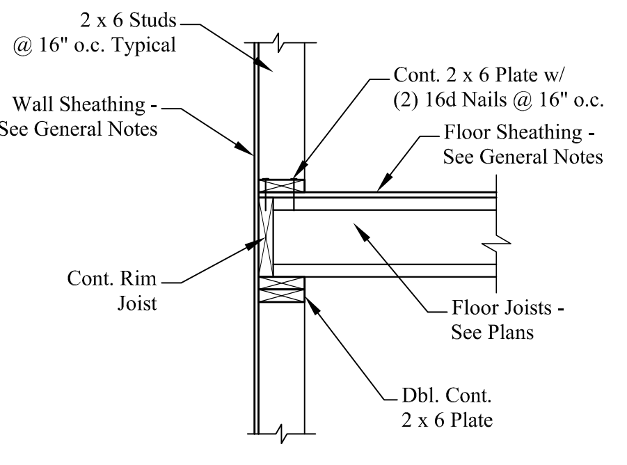
9 FLOOR JOIST @ BRG. WALL Scale: 3/4" = 1'-0"
