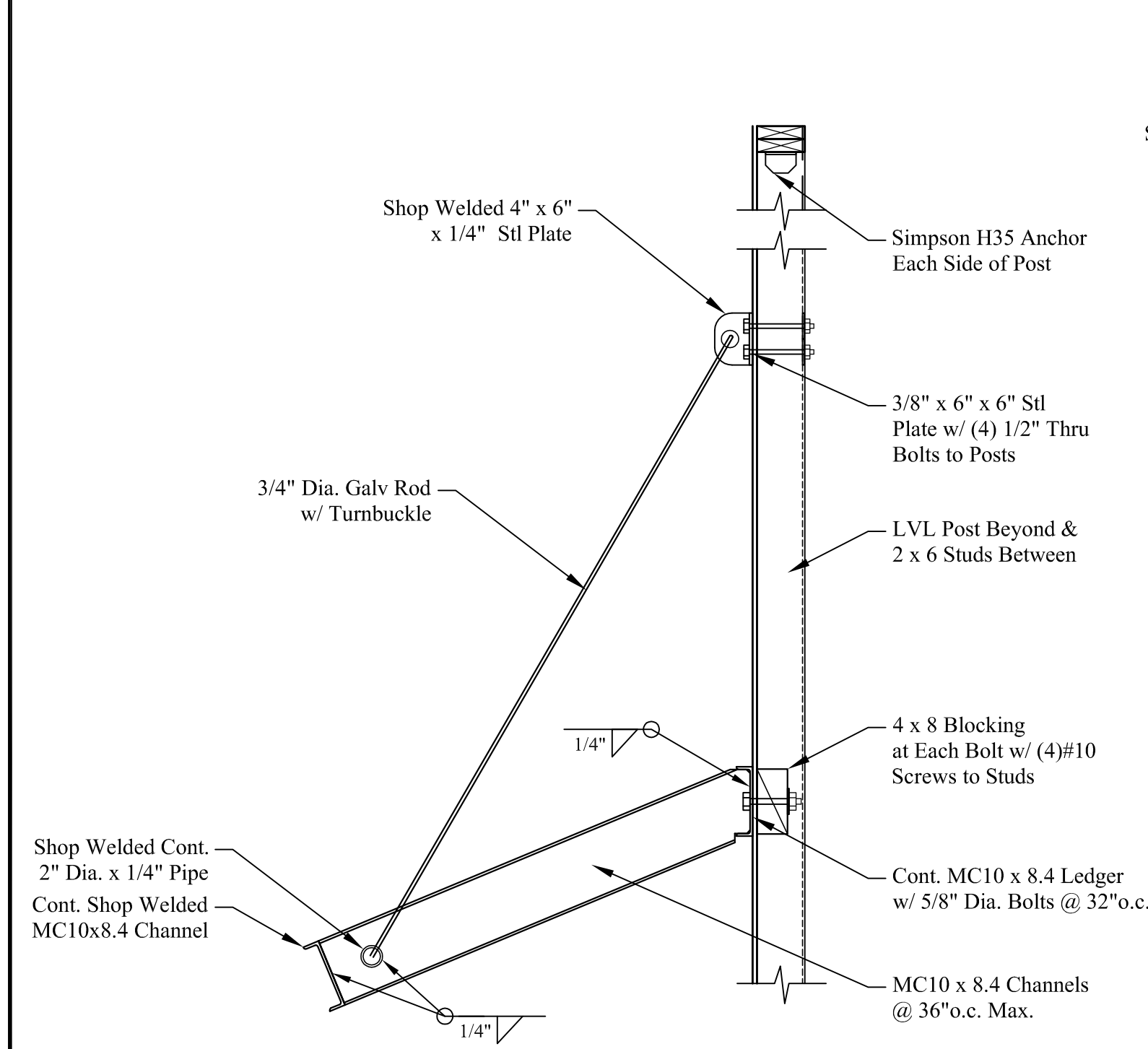
13 HANGING CANOPY ROOF Scale: 3/4" = 1'-0"
