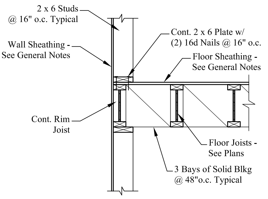
10 FLOOR JOIST @ NON-BRG. WALL Scale: 3/4" = 1'-0"
