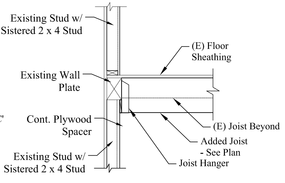
15 FLOOR JOIST @ BRG. WALL Scale: 3/4" = 1'-0"
