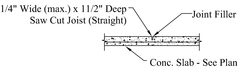
5 TYP. FLOOR & WALL JOINTS Scale: 1/2" = 1'-0"
