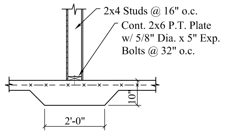
6 TYP. THICKENED SLAB FTG. Scale: 1/2" = 1'-0"
