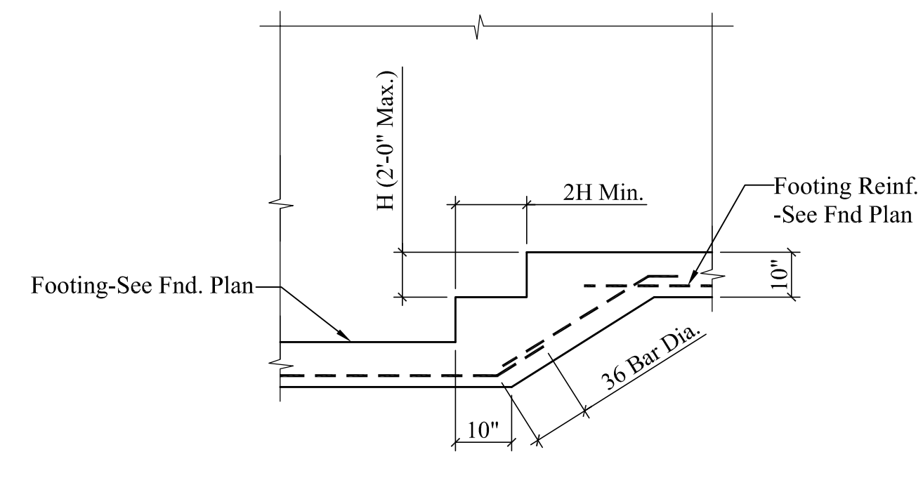
4 TYP STEP FOOTING DETAIL Scale: 1/2" = 1'-0"
