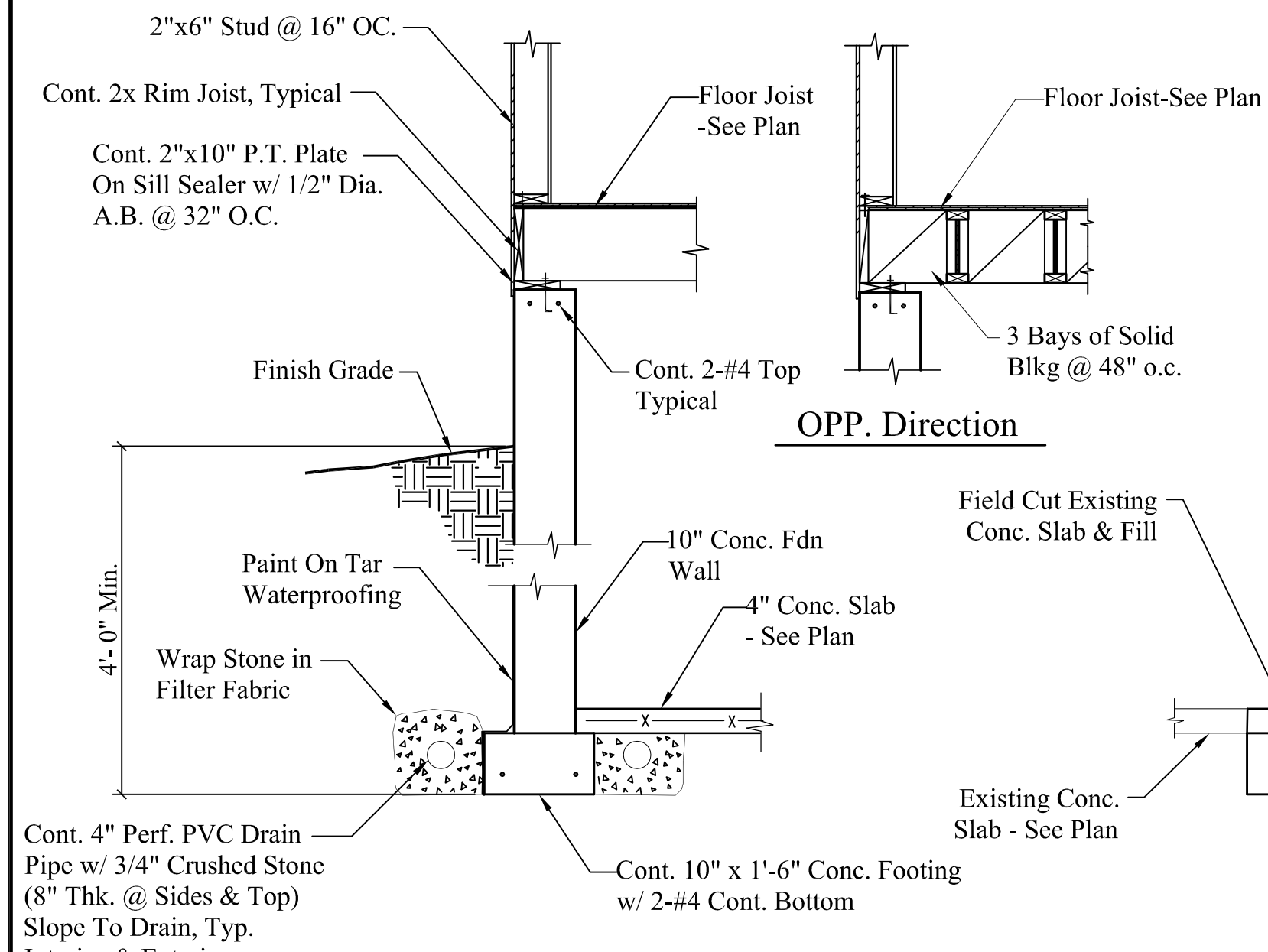
1 FOUNDATION @ STUD WALL Scale: 1/2" = 1'-0"
