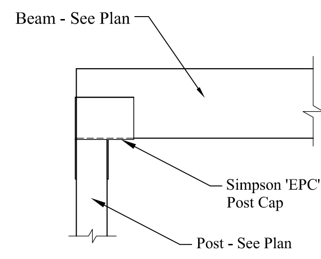
11 WOOD BM. to WOOD POST CONN. Scale: 3/4" = 1'-0"
