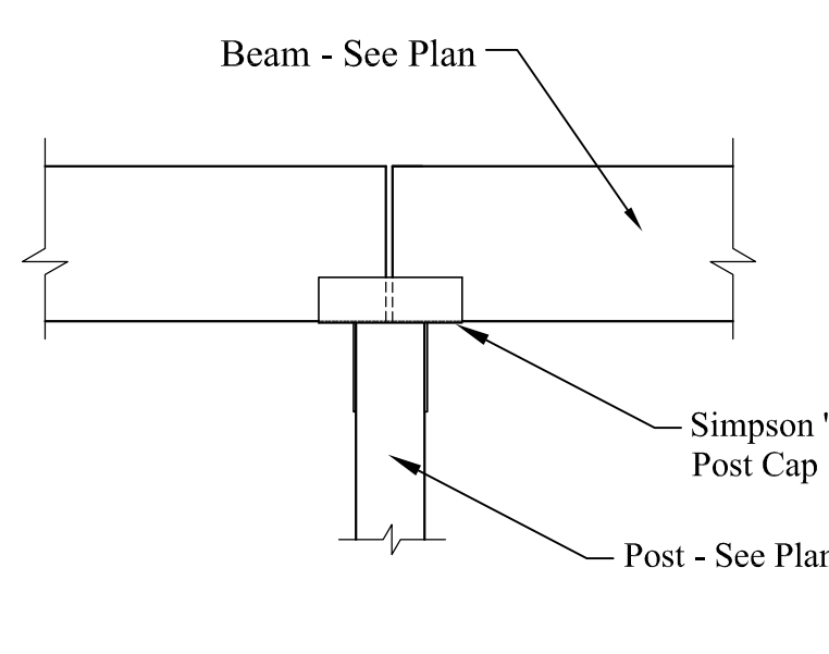
14 WOOD BM. to WOOD POST CONN. Scale: 3/4" = 1'-0"
