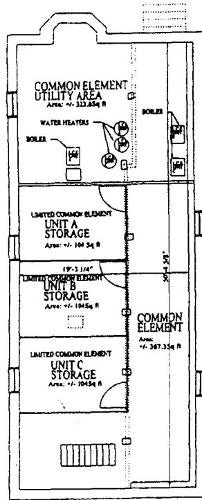
BASEMENT
