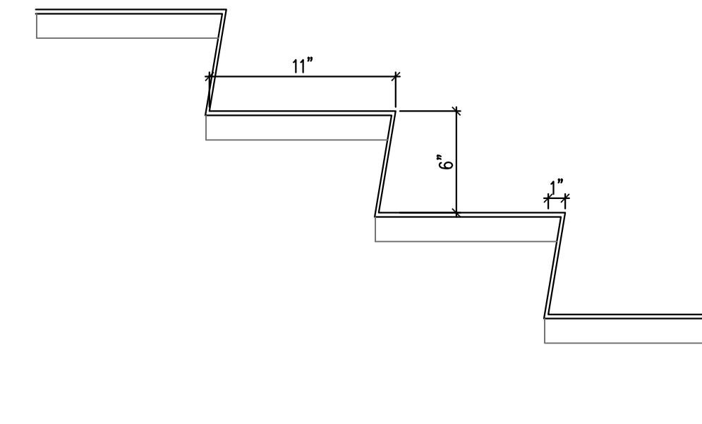
4 PROPOSED RISER & RUN A1.01 1 1/2" = 1'-0"
