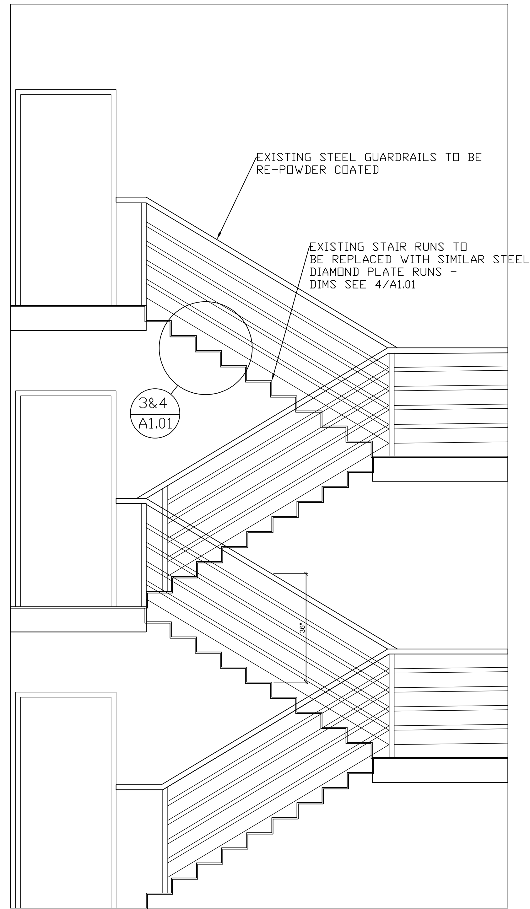
2 EXISTING STAIR SECTION A A1.01 1/2" = 1'-0"
