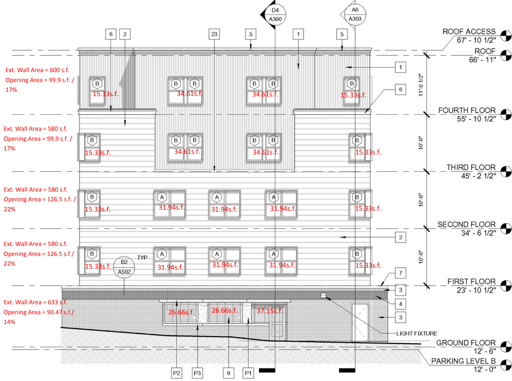
D2 EXTERIOR ELEVATION EAST - A WING 1/8" = 1'-0"
