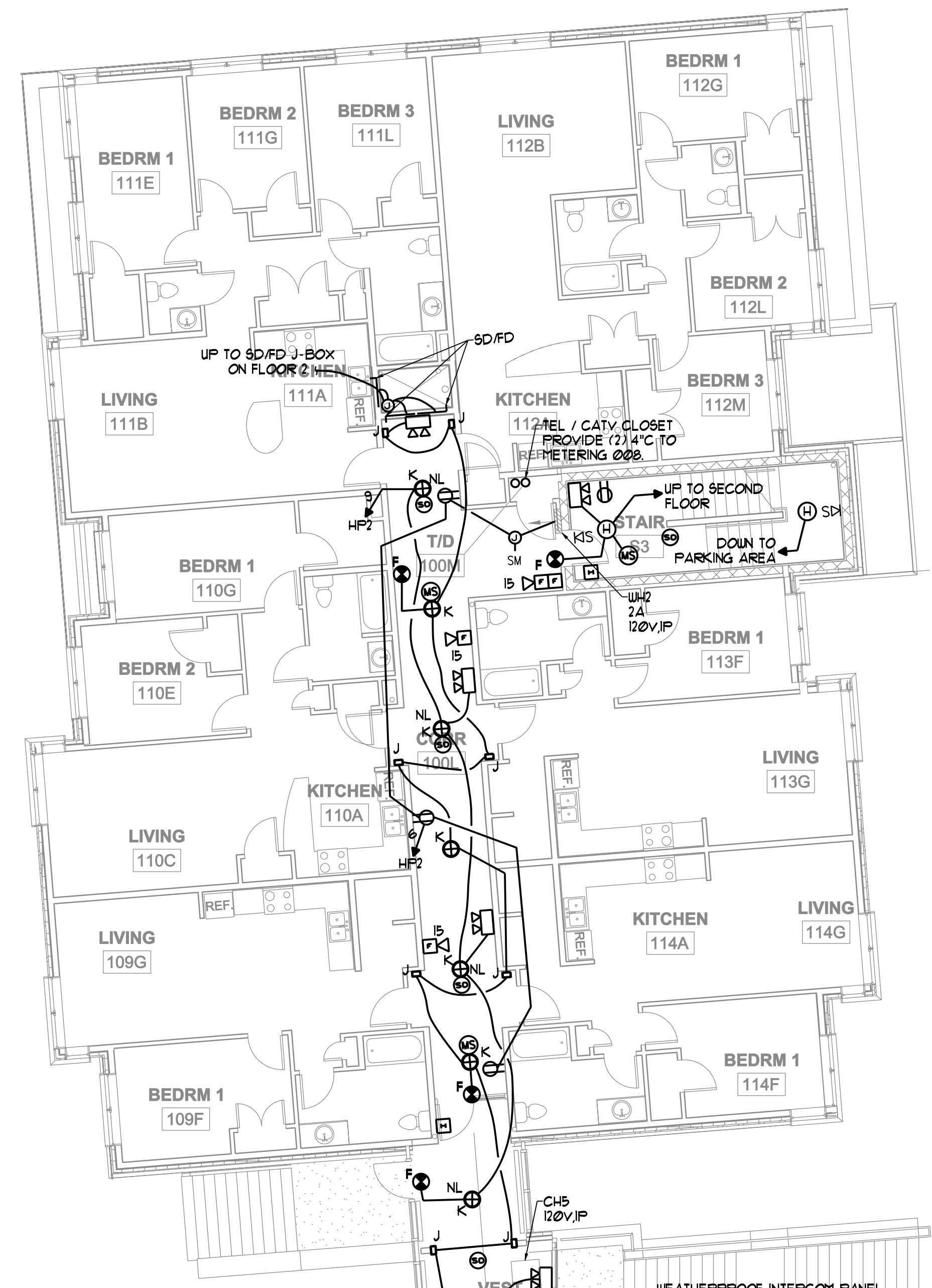
FIRST FLOOR ELECTRICAL PLAN SCALE: 1/8" = 1'-0"
