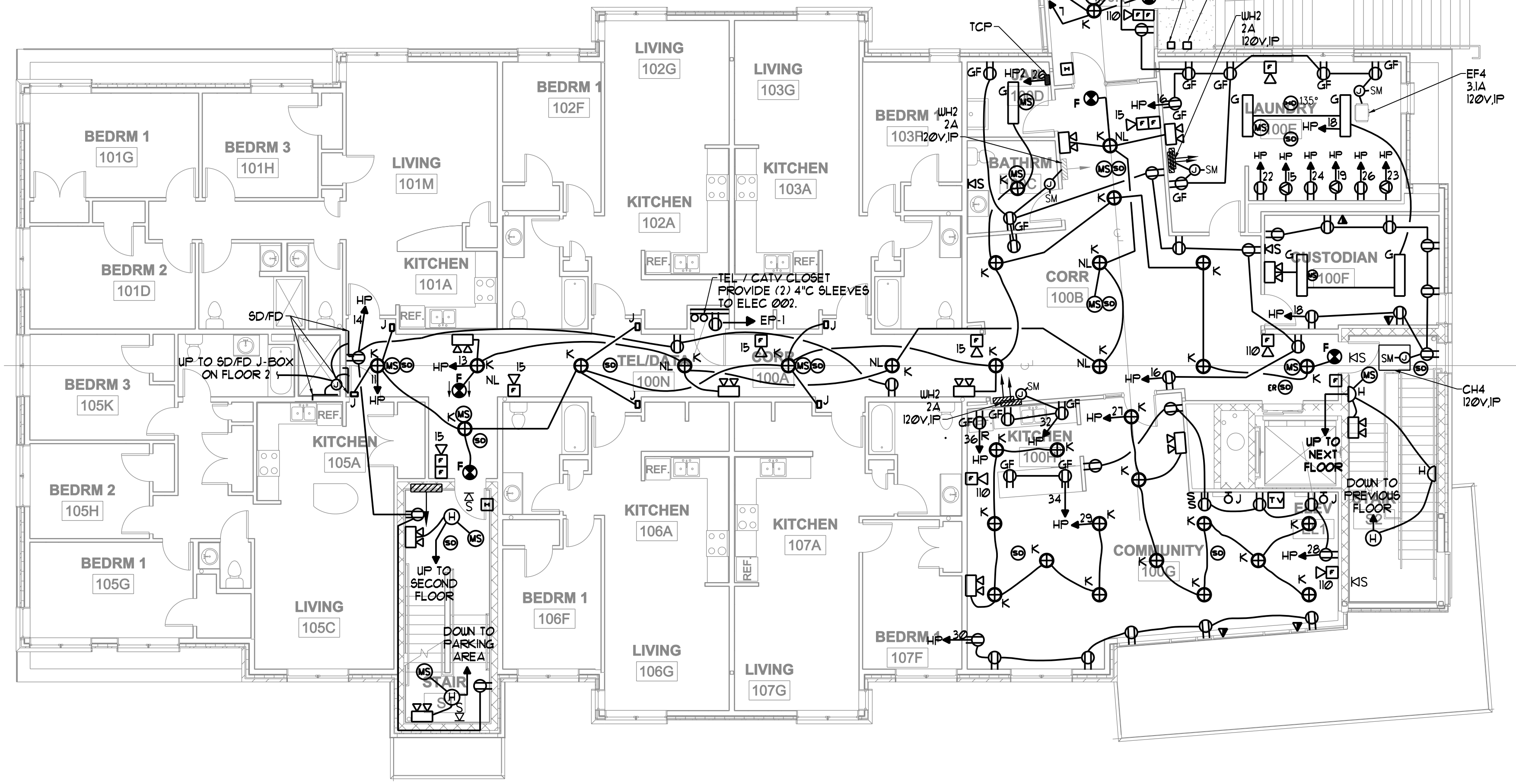
FIRST FLOOR ELECTRICAL PLAN SCALE: 1/8" = 1'-0"
