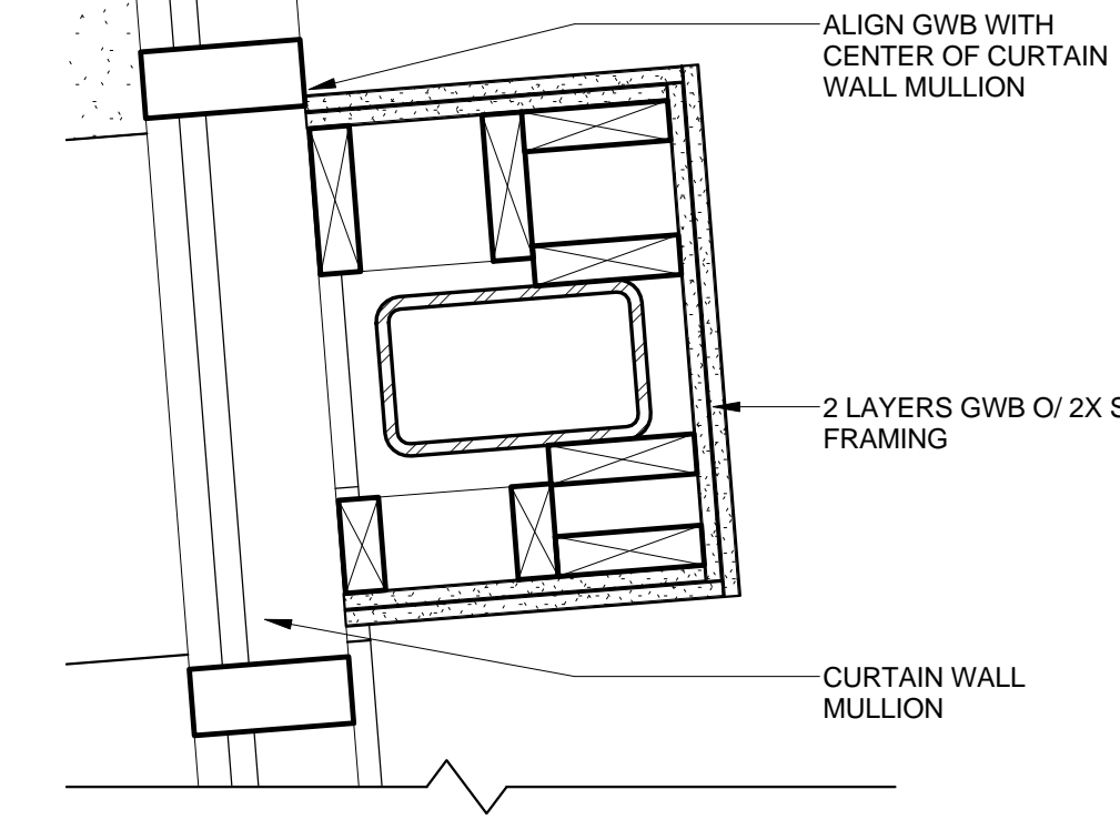
E4 TYPICAL COLUMN ENCLOSE AT LINK 1 1/2" = 1'-0"
