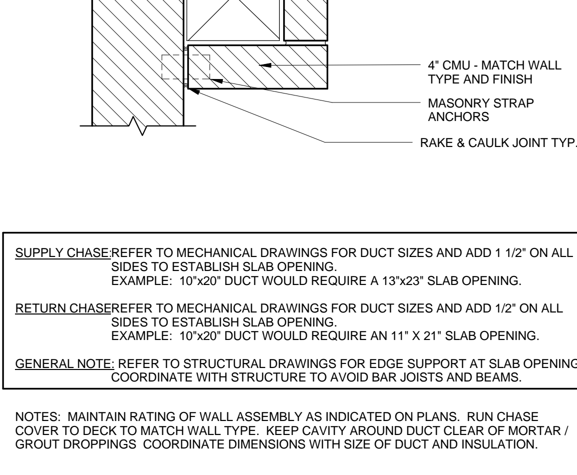
A2 CHASE AT INTERIOR PARTITION 1 1/2" = 1'-0"
