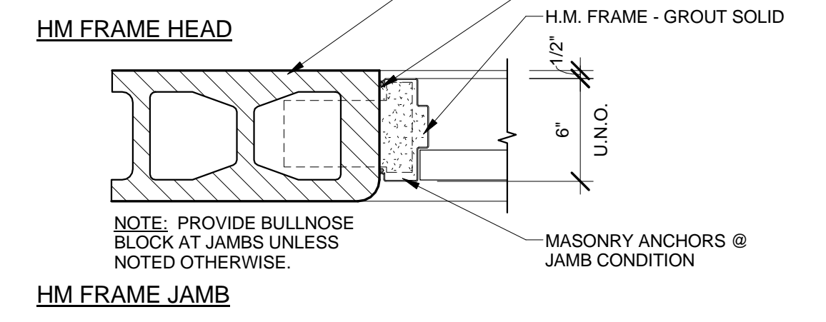
E1 HM FRAME DETAILS @ CMU 1 1/2" = 1'-0"
