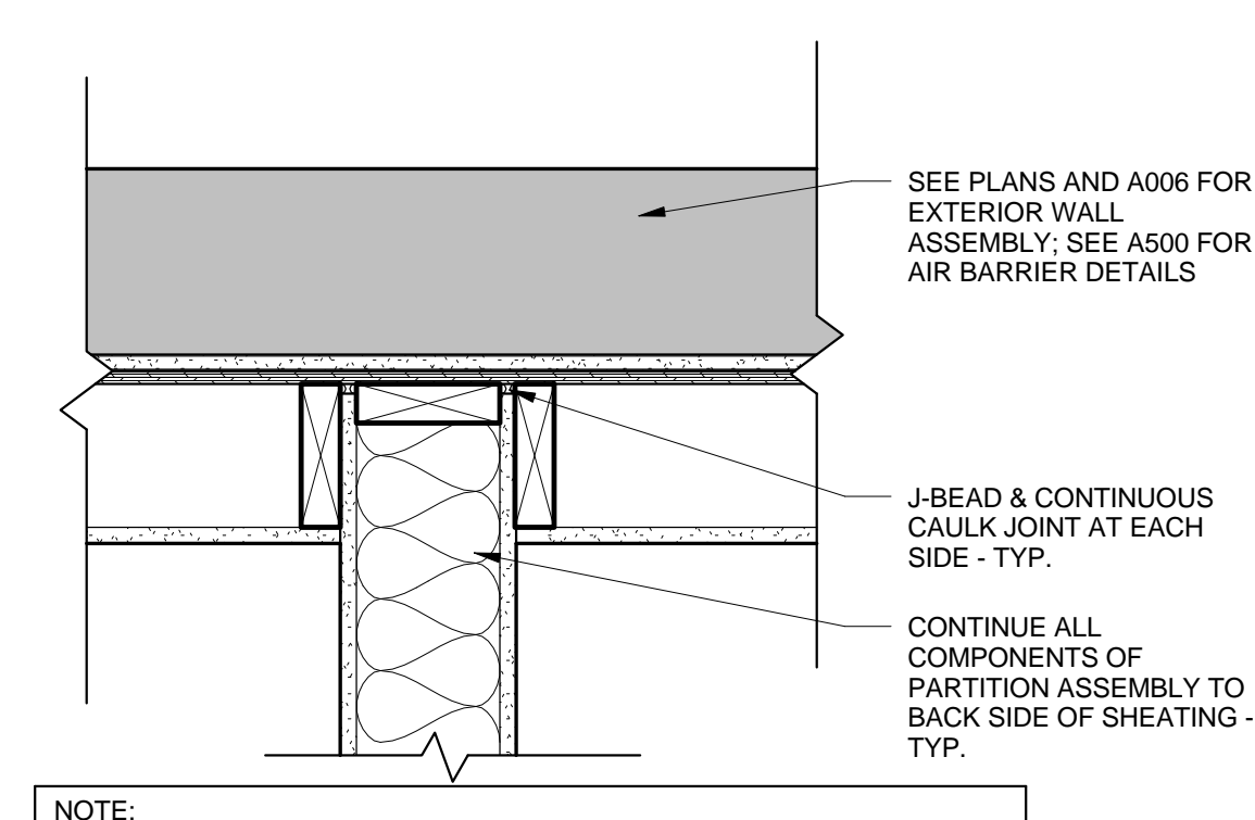
D2 TYPICAL WALL INTERSECTIONS 1 1/2" = 1'-0"
