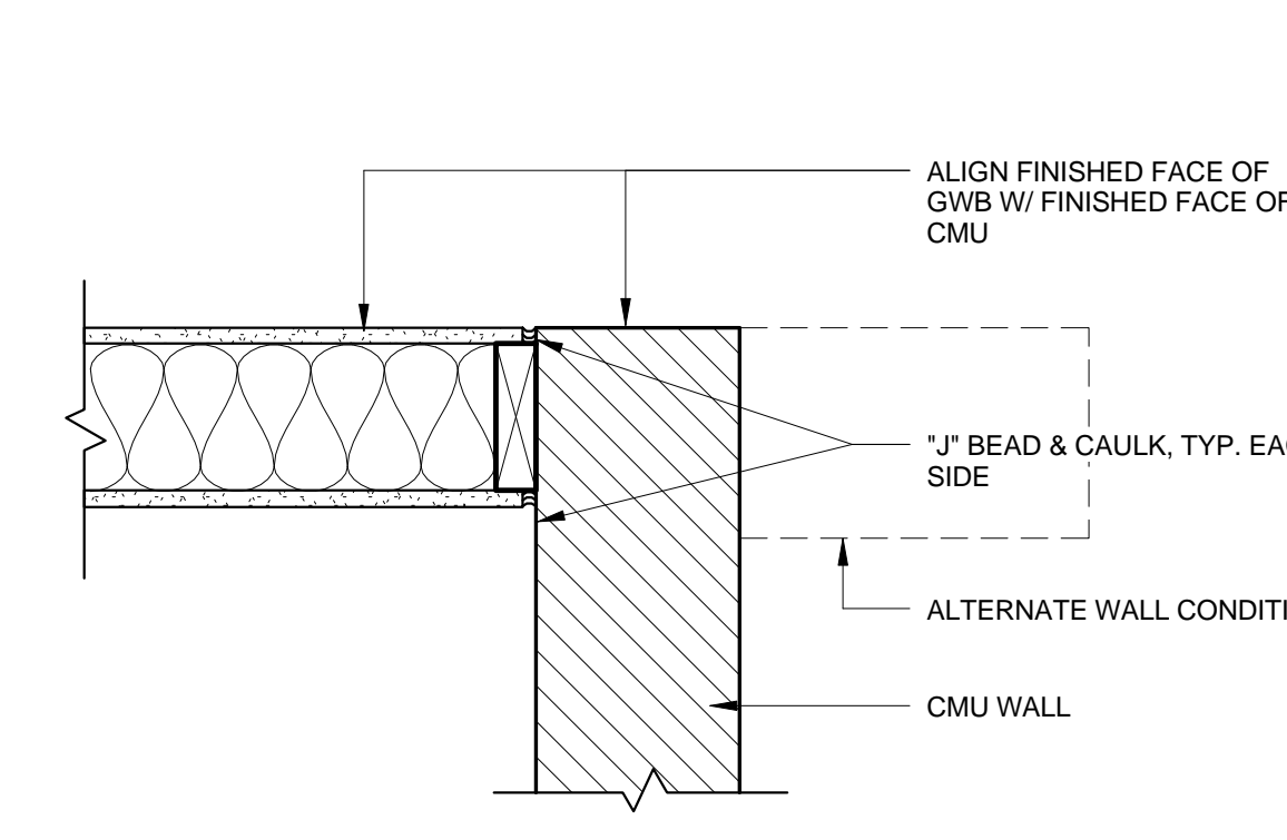
D1 PARTITION STANDARDS 1 1/2" = 1'-0"
