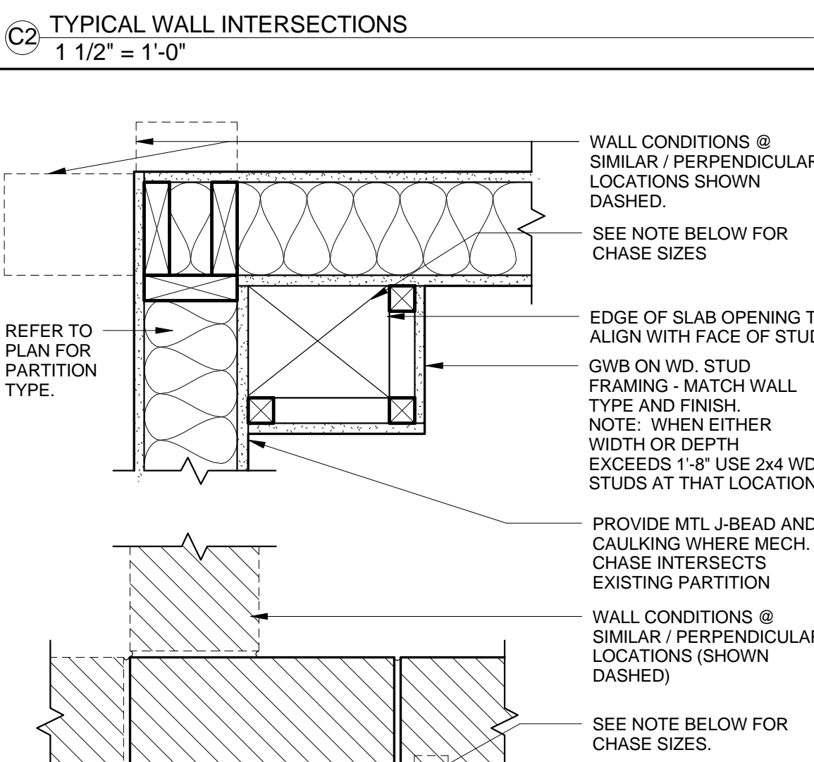
A2 CHASE AT INTERIOR PARTITION 1 1/2" = 1'-0"
