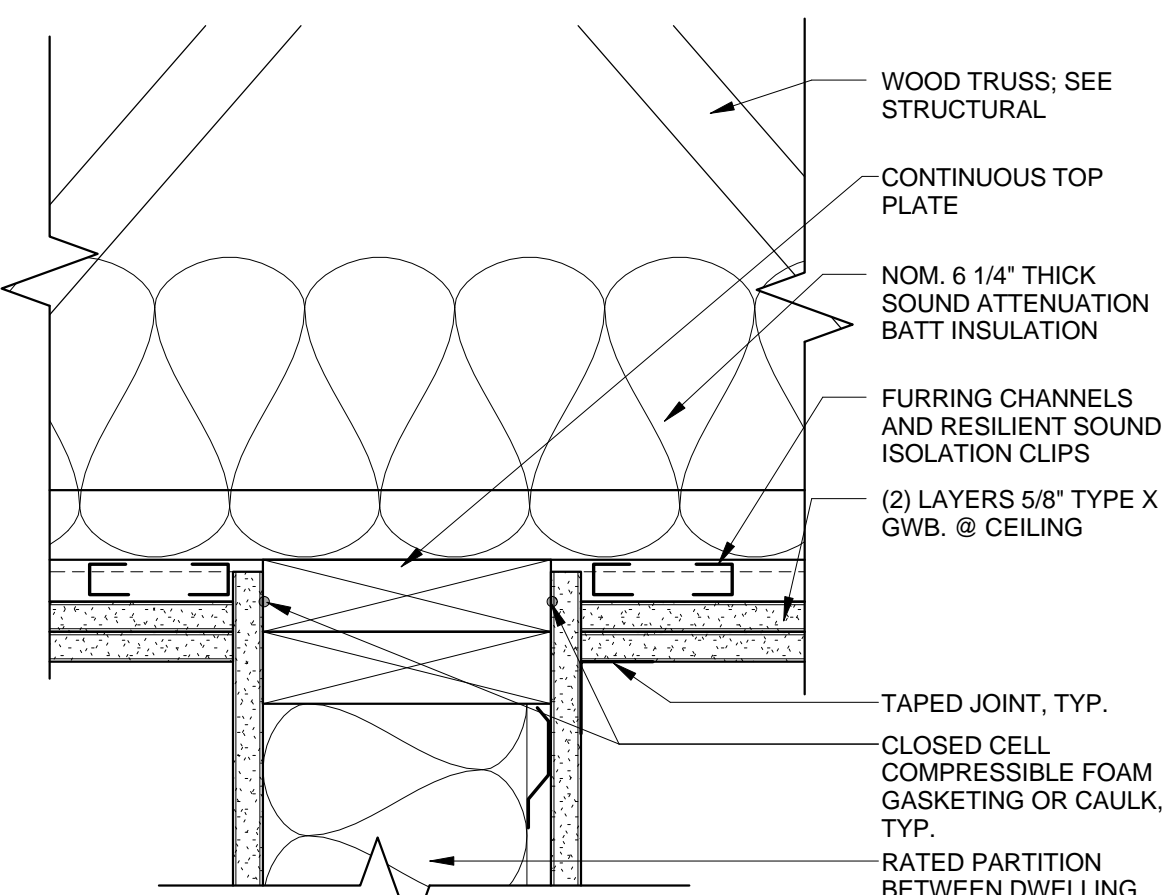
D5 RATED FLOOR AT 2HR RATED ENCLOSURE 1 1/2" = 1'-0"
