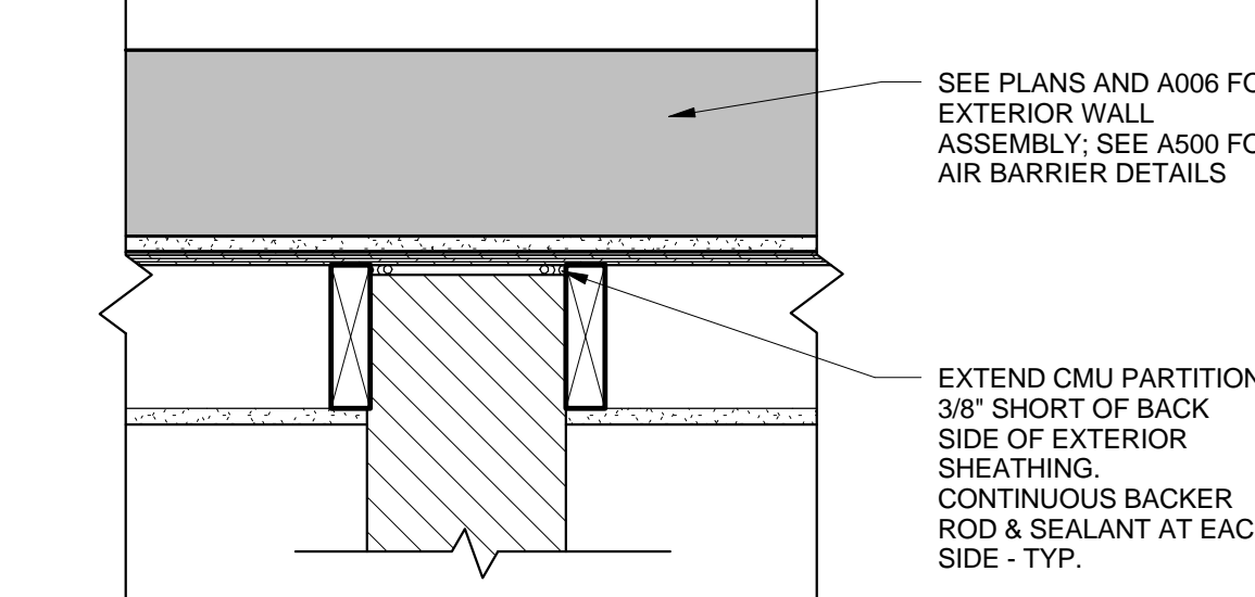
D2 TYPICAL WALL INTERSECTIONS 1 1/2" = 1'-0"
