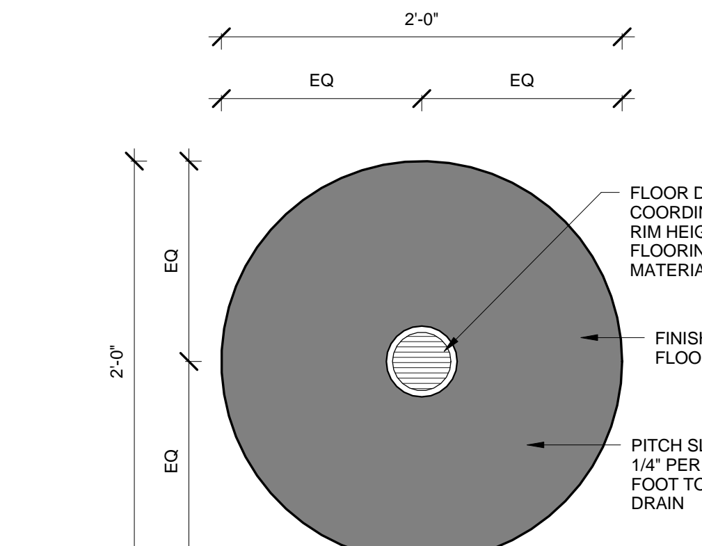
D4 FLOOR DRAIN - CIRCULAR 1 1/2" = 1'-0"
