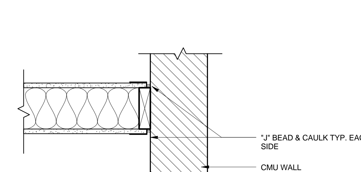
D1 PARTITION STANDARDS 1 1/2" = 1'-0"
