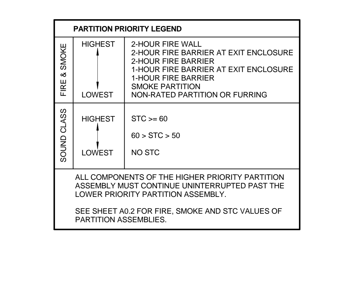
A3 PARTITION PRIORITY 1 1/2" = 1'-0"
