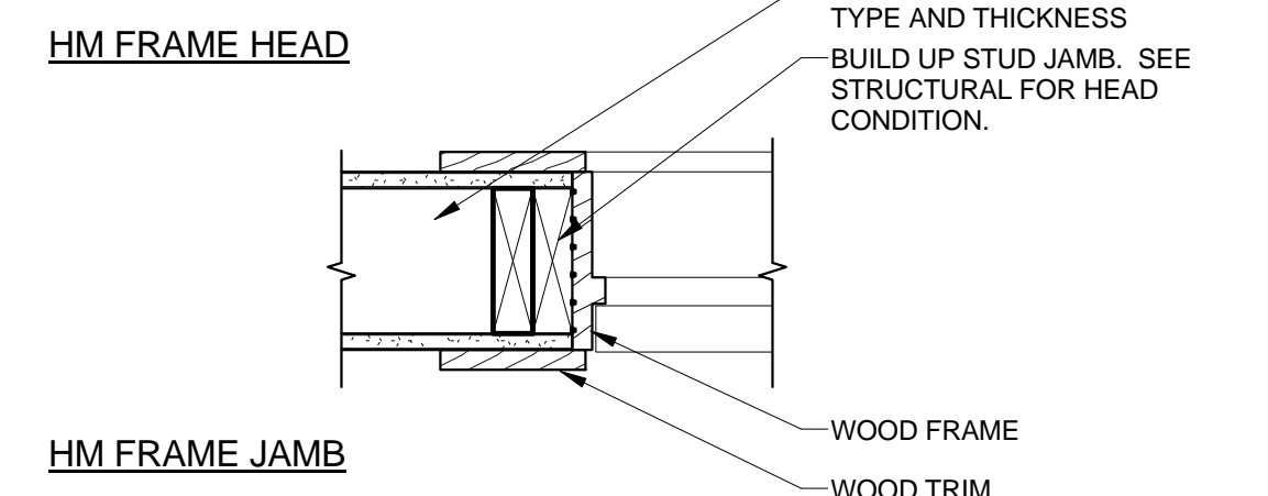
E3 WOOD FRAME DETAILS @ GWB 1 1/2" = 1'-0"
