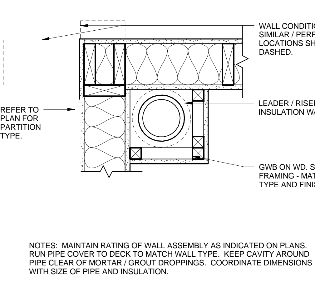
A4 LEADER / RISER ENCLOSURE 1 1/2" = 1'-0"
