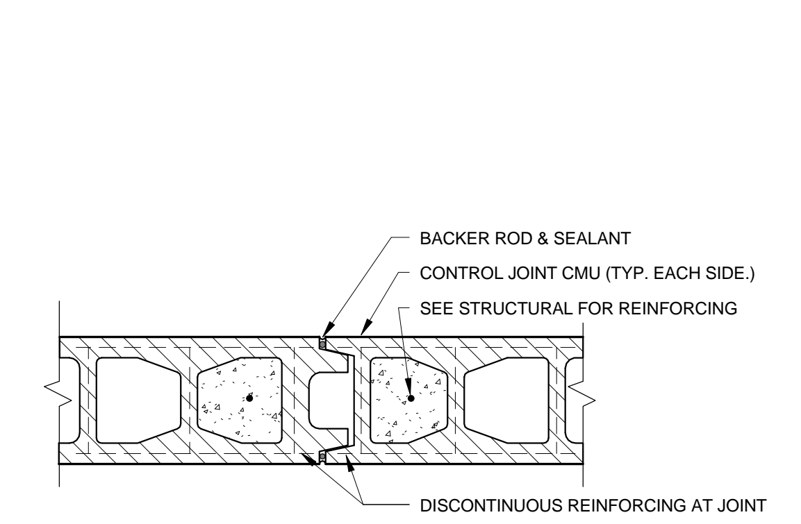
D3 CONTROL JOINT AT EXTERIOR CMU WALL 1 1/2" = 1'-0"
