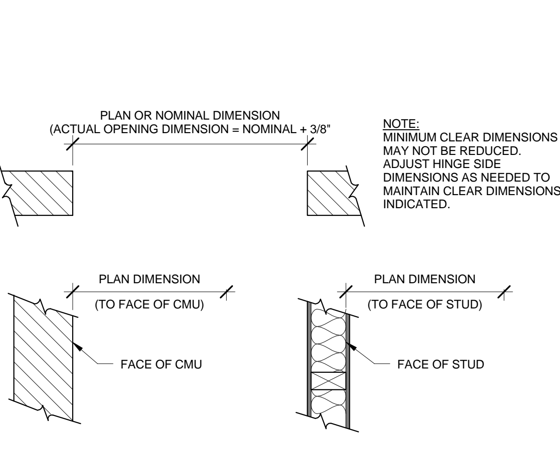
A1 DIMENSIONAL STANDARDS 1 1/2" = 1'-0"
