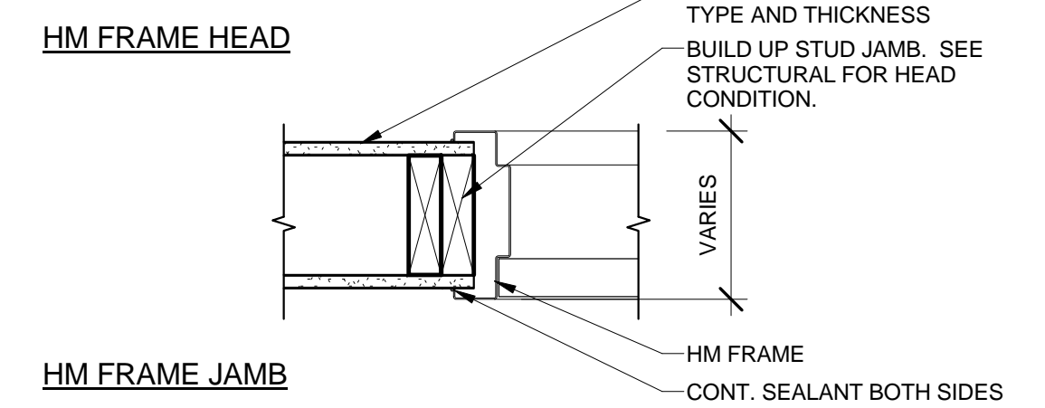
E2 HM FRAME DETAILS @ GWB 1 1/2" = 1'-0"
