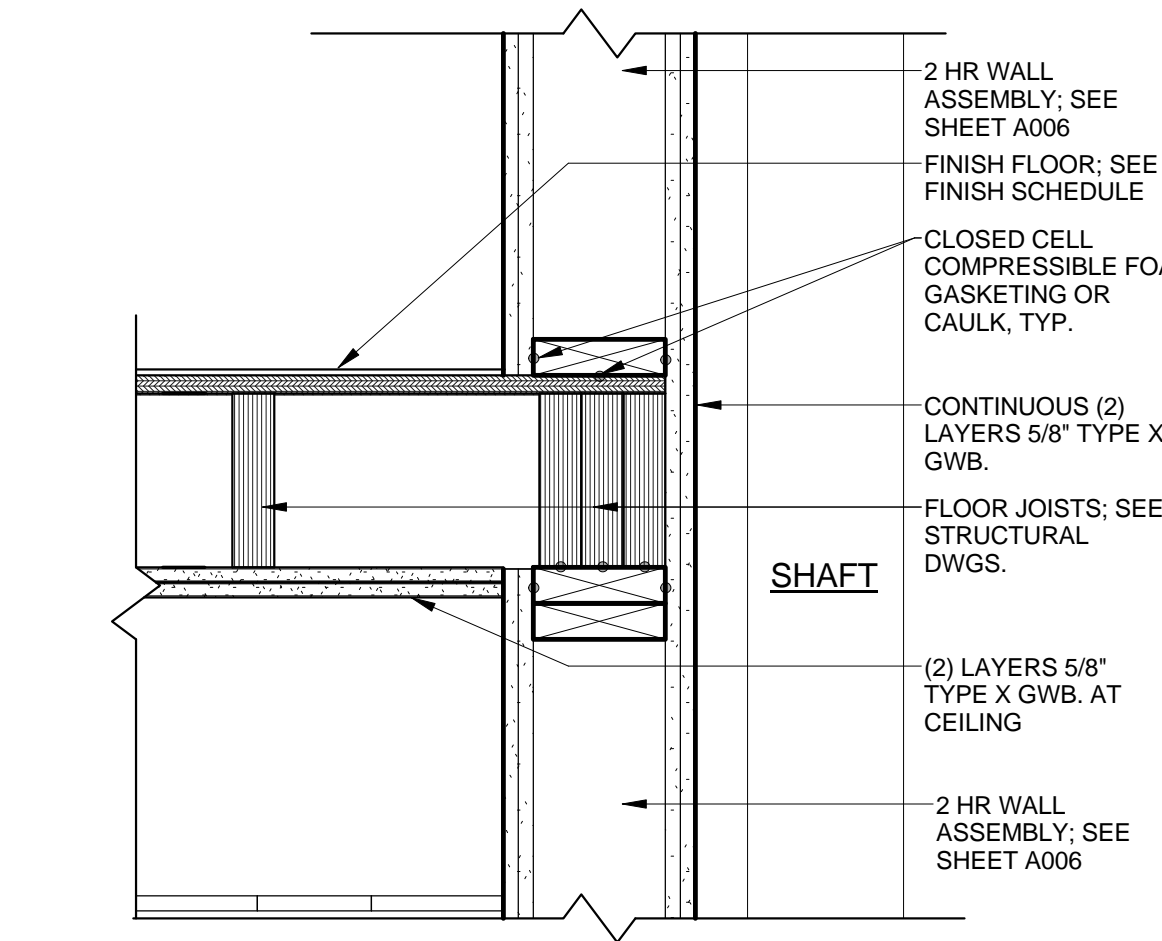
D5 RATED FLOOR AT 2HR RATED ENCLOSURE 1 1/2" = 1'-0"
