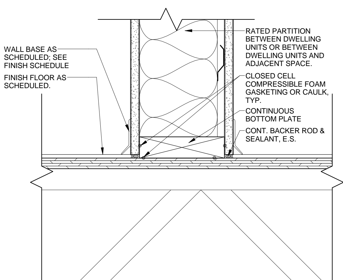
A5 COMPARTMENTALIZATION - PARTITION TO FLOOR 3" = 1'-0"
