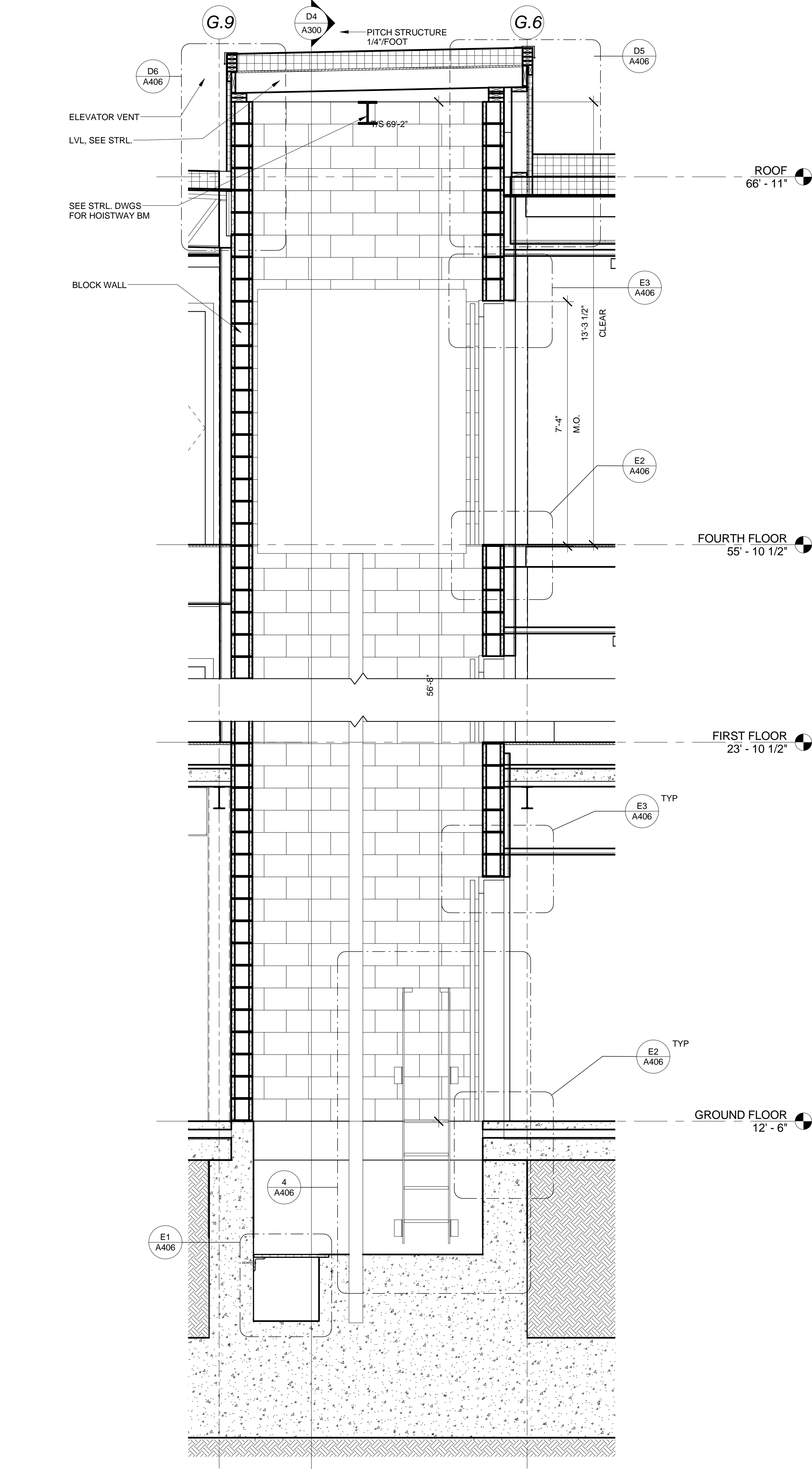
A2 ELEVATOR SECTION 1/2" = 1'-0"
