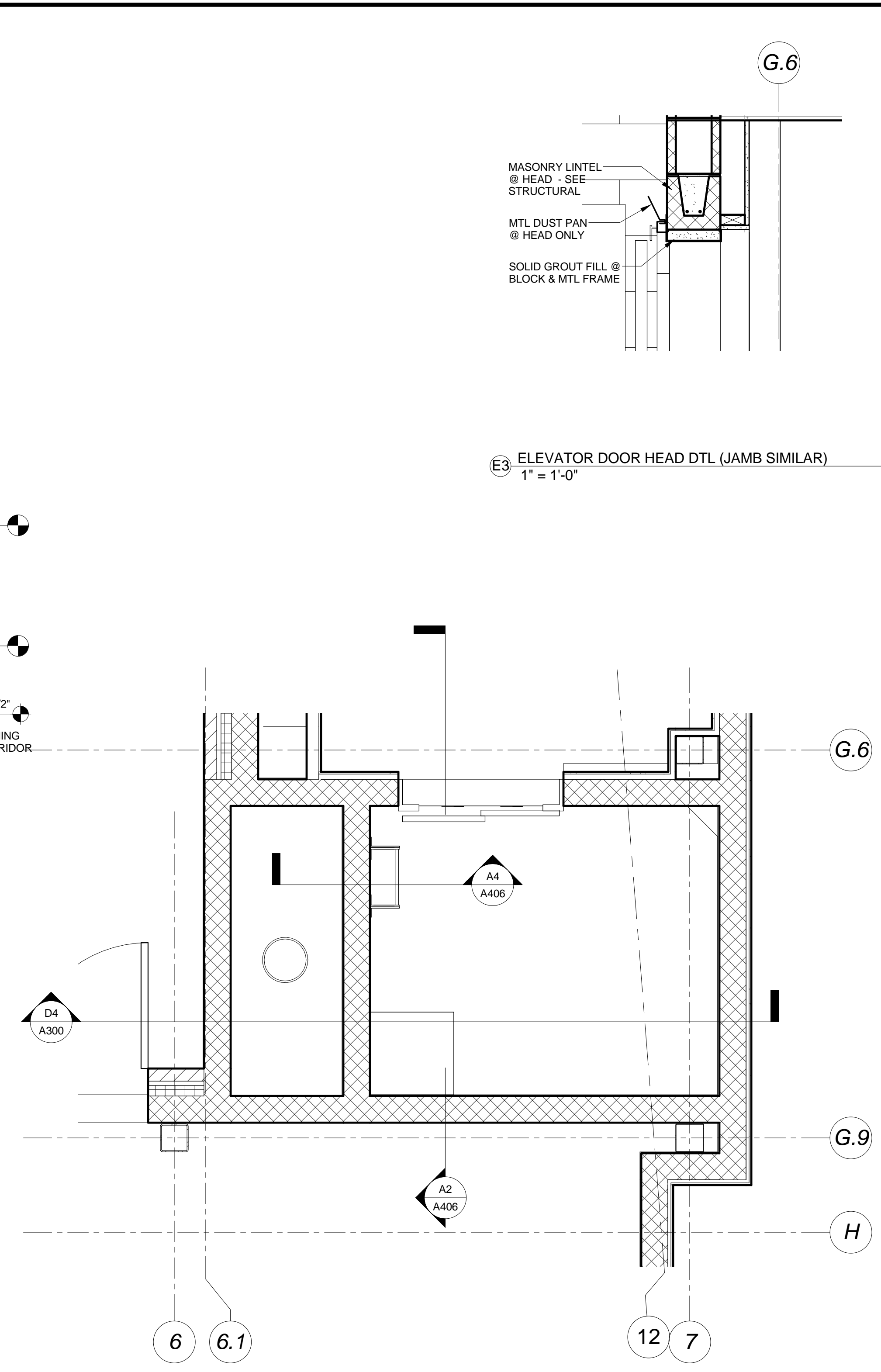
C4 ENLARGED ELEVATOR PLAN 1/2" = 1'-0"
