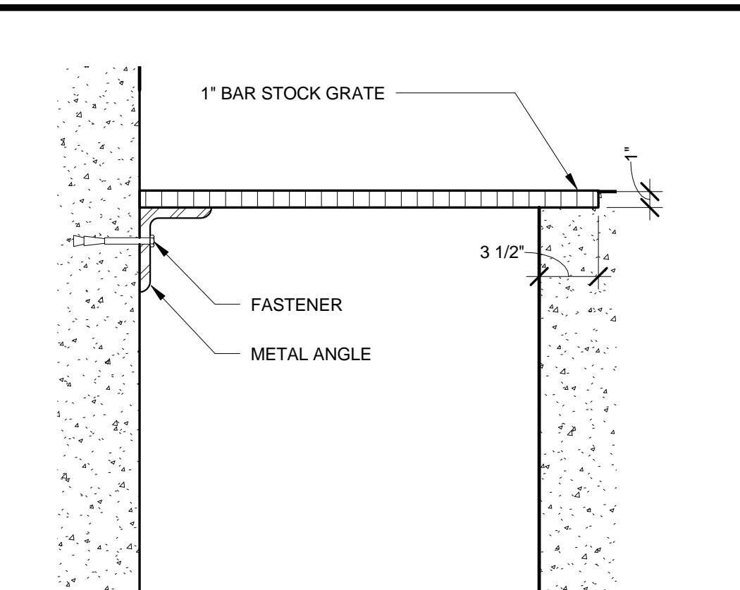
E1 ELEVATOR PIT GRATE SECTION 1 1/2" = 1'-0"
