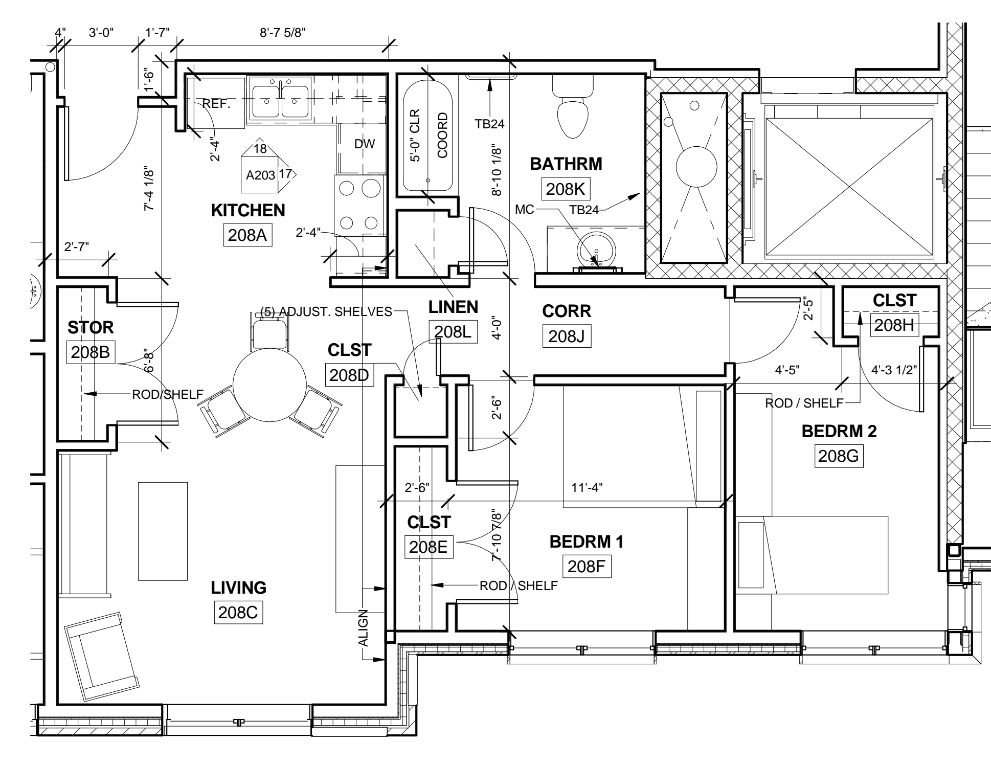
3A UNIT 208, 308, 408 (2-B-2) 1/4" = 1'-0"
