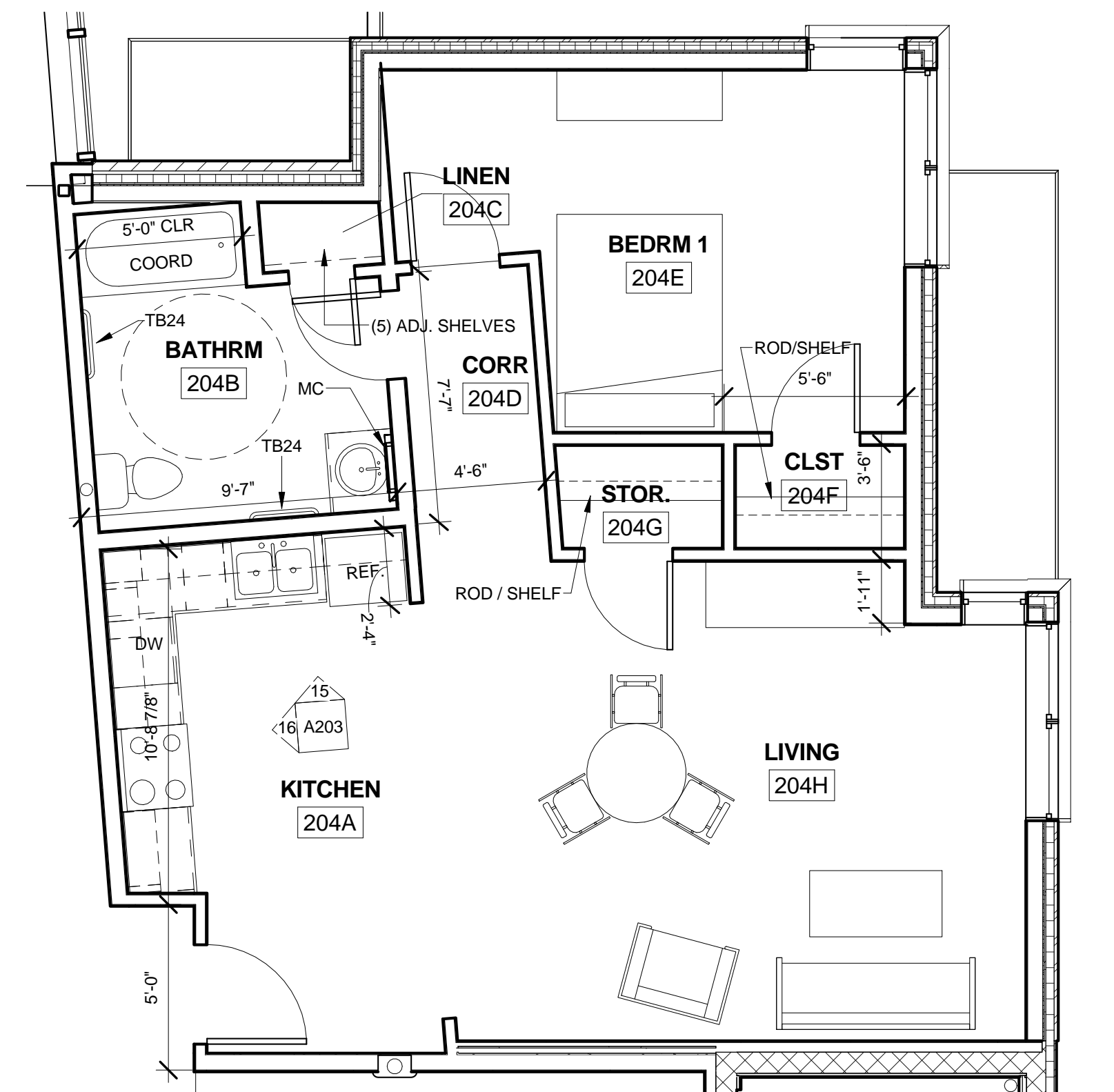
2A UNIT 204 (1-B-3) 1/4" = 1'-0"
