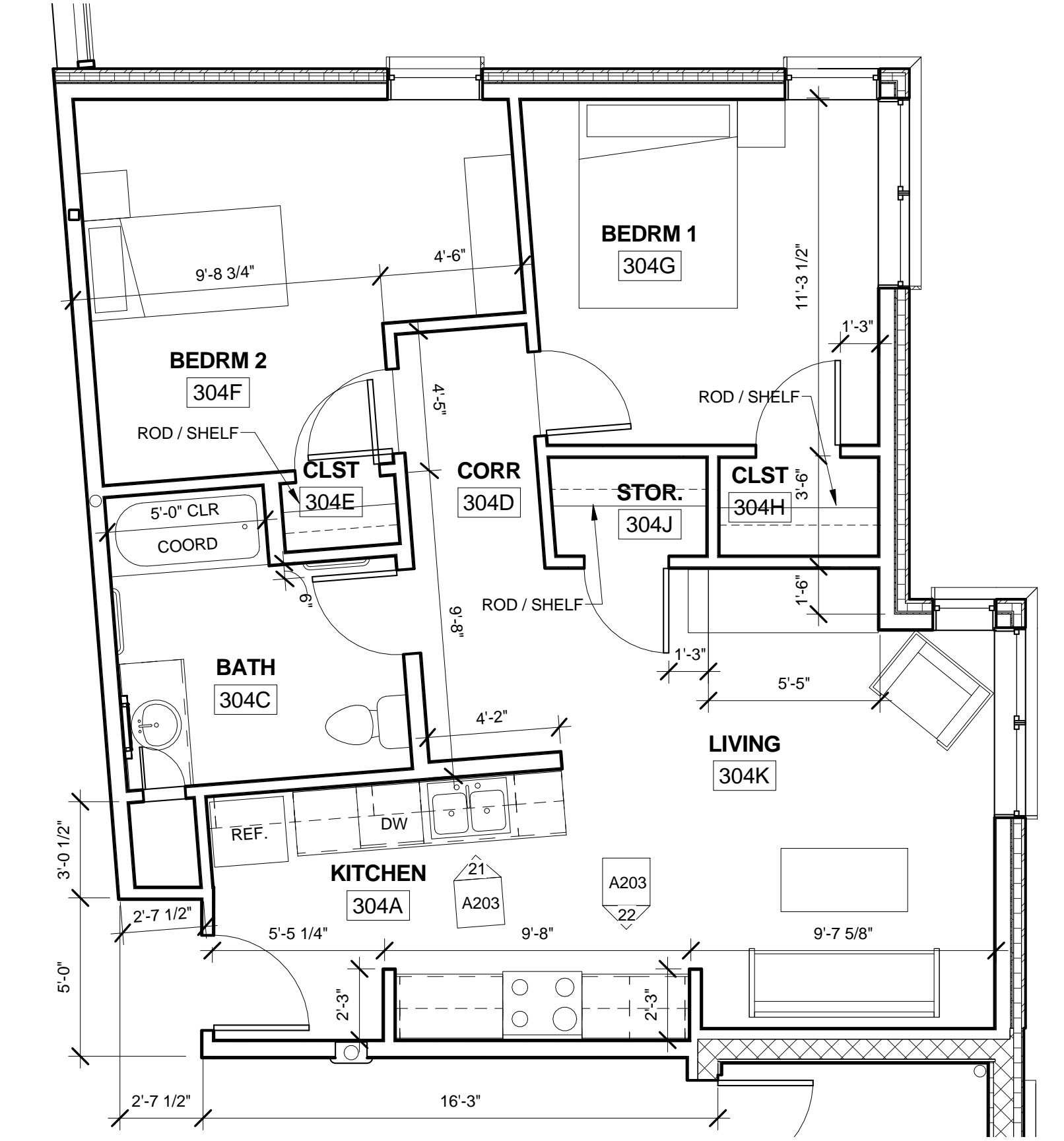
2D UNIT 304 (2-B-4) 1/4" = 1'-0"
