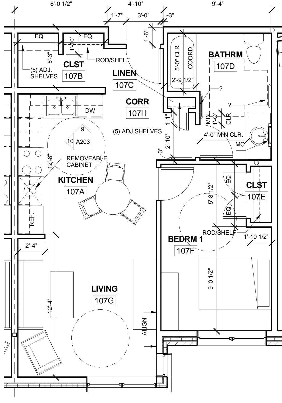
6A UNIT 107, 109, 209, 207, 309, 407, 409 (1-A-1) 1/4" = 1'-0"
