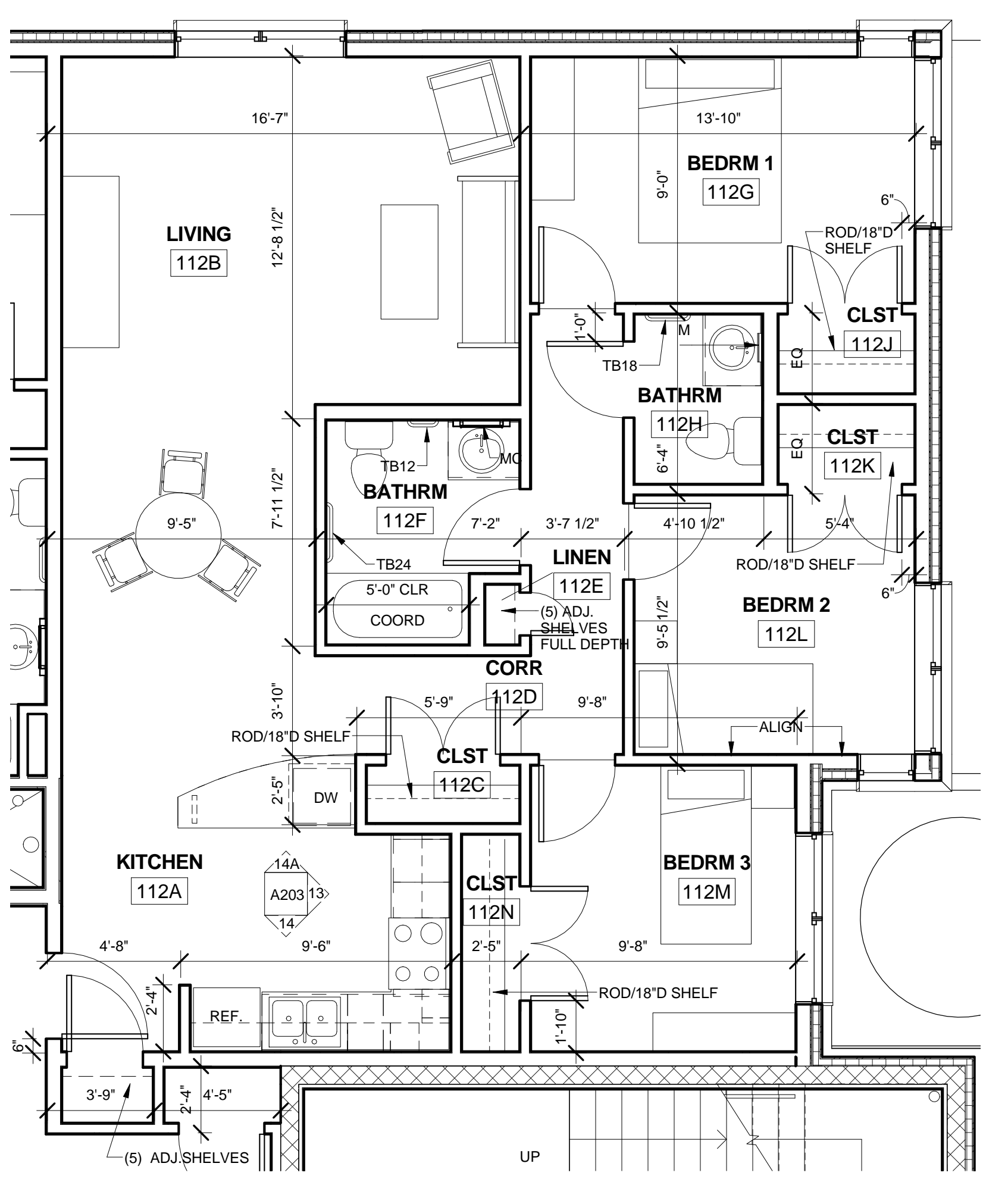
5D UNIT 112 (3-B-3) 1/4" = 1'-0"
