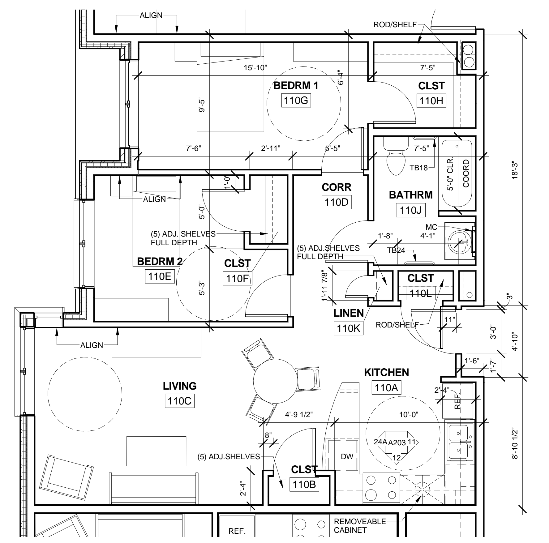
2D UNIT 110, 210, 310, 410 (2-A-3) 1/4" = 1'-0"
