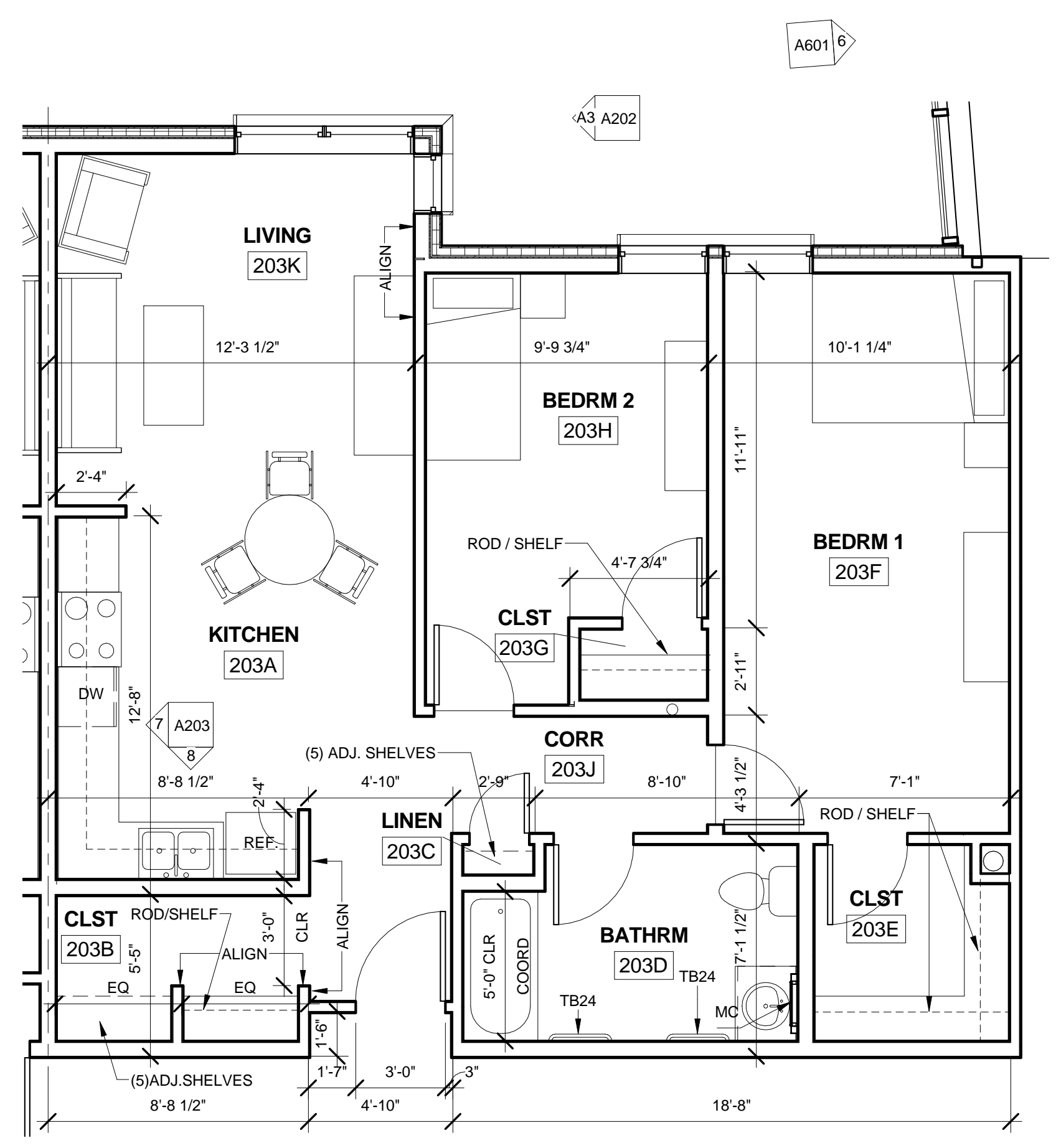
6D UNIT 203, 303, 403 (2-B-1) 1/4" = 1'-0"
