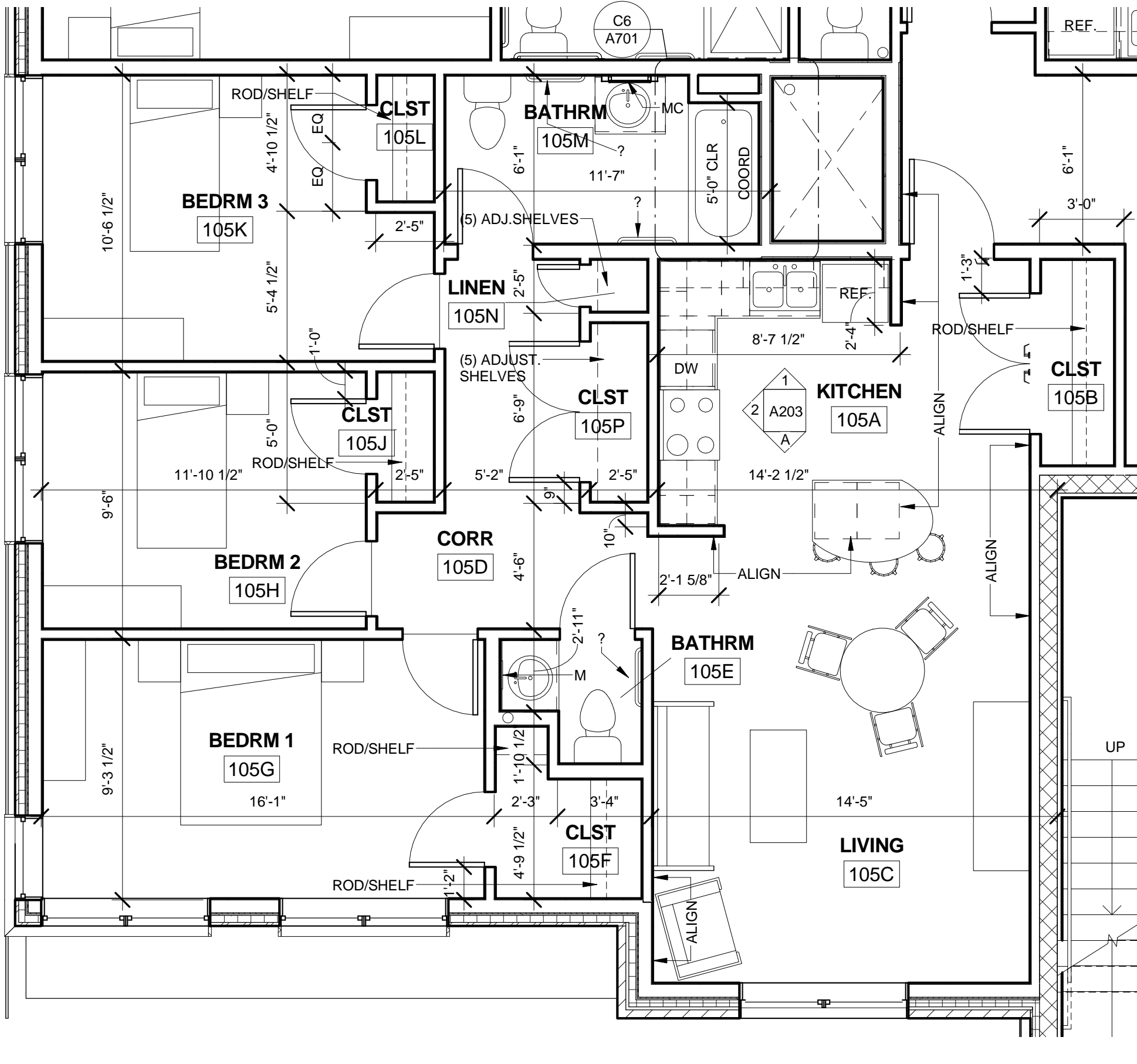
5A UNIT 105, 205, 305 (3-B-1) 1/4" = 1'-0"
