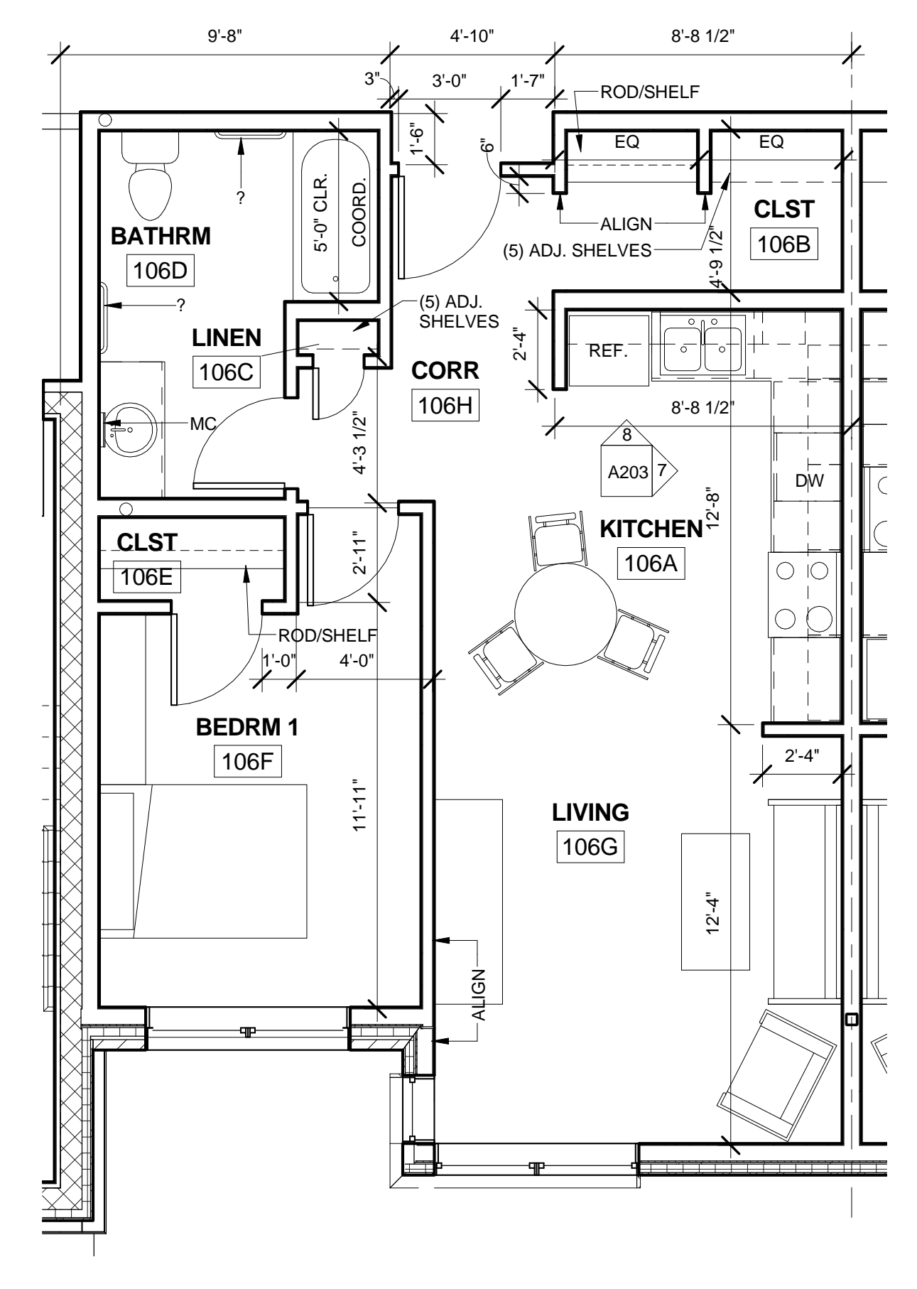
6A UNIT 103, 106, 113, 114, 206, 213, 214, 306, 313, 314, 406, 413, 414 (1-B-2) 1/4" = 1'-0"
