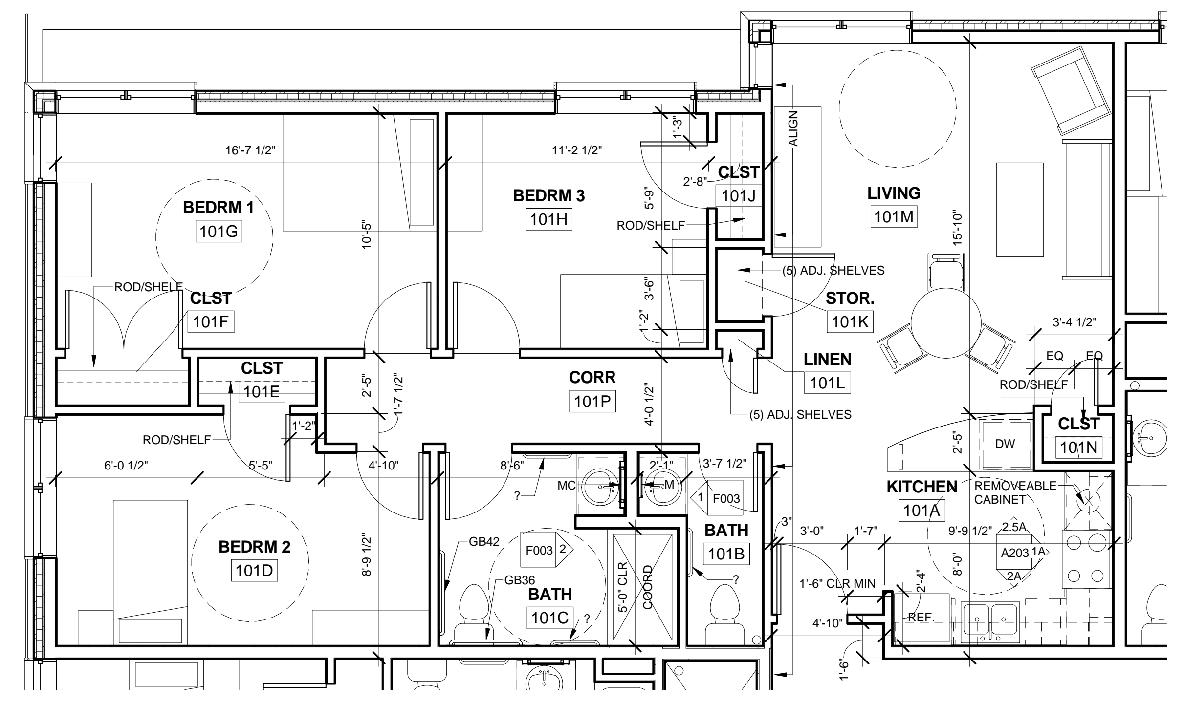
2A UNIT 101, 201, 301 (3-A-1) 1/4" = 1'-0"
