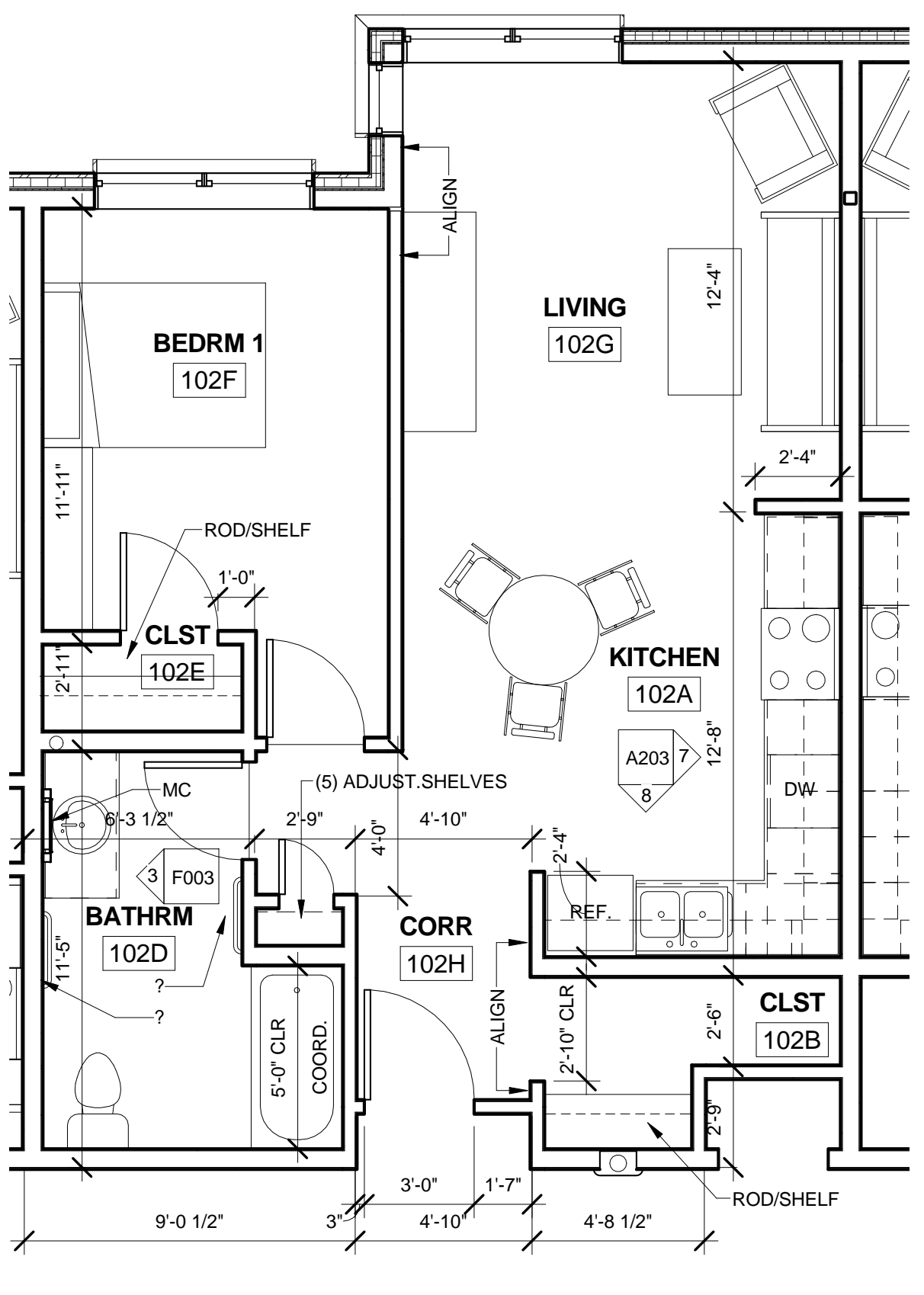
3A UNIT 102, 202, 302, 402 (1-B-1) 1/4" = 1'-0"
