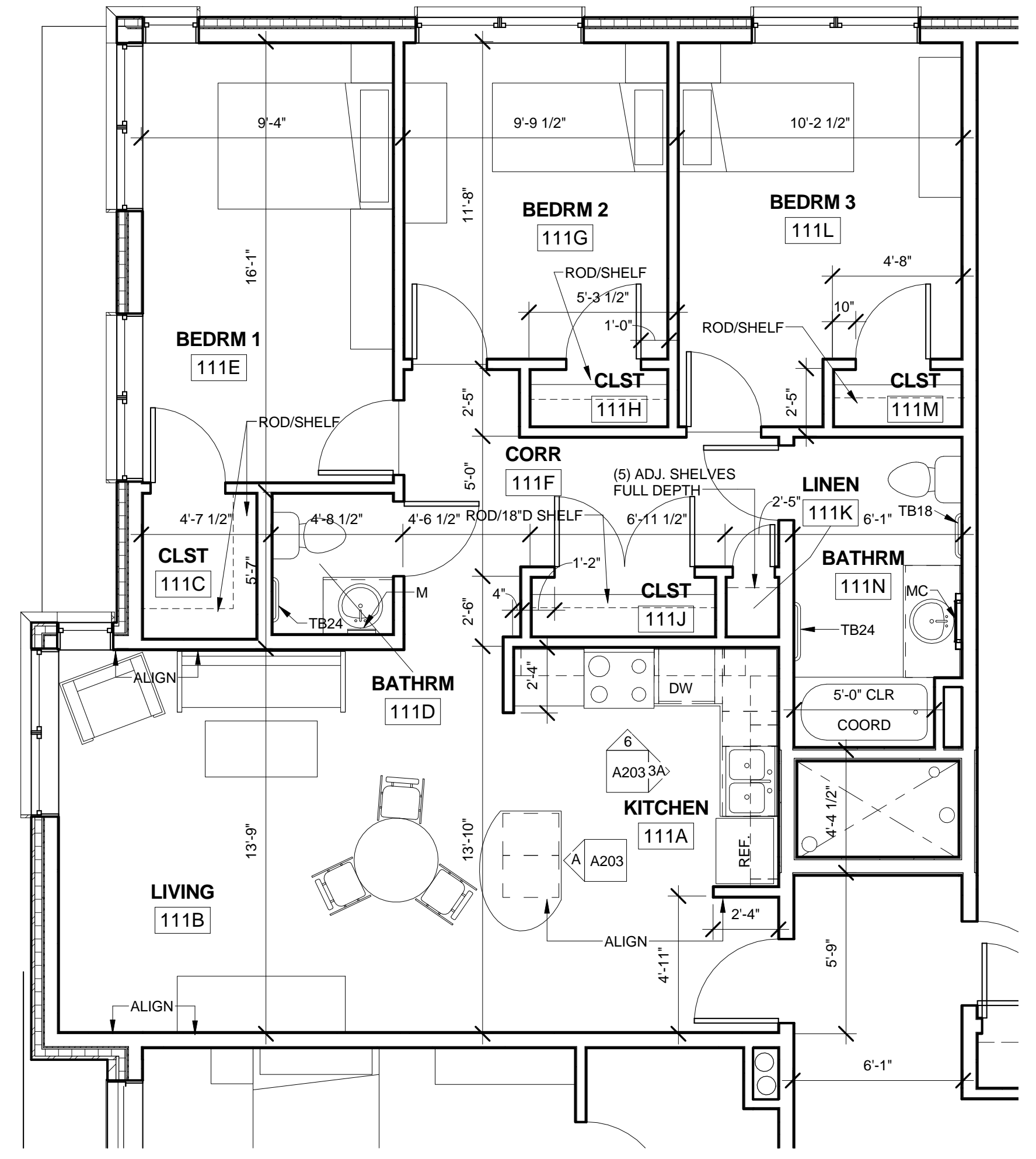
3D UNIT 111, 211, 311, 411 (3-B-2) 1/4" = 1'-0"
