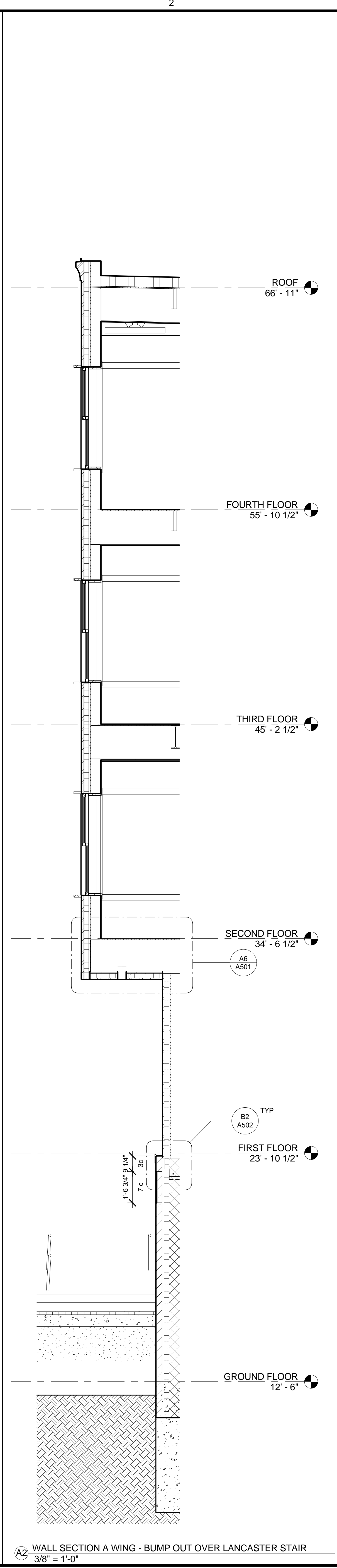
A3 WALL SECTION THROUGH BUMP OUT 3/8" = 1'-0"
