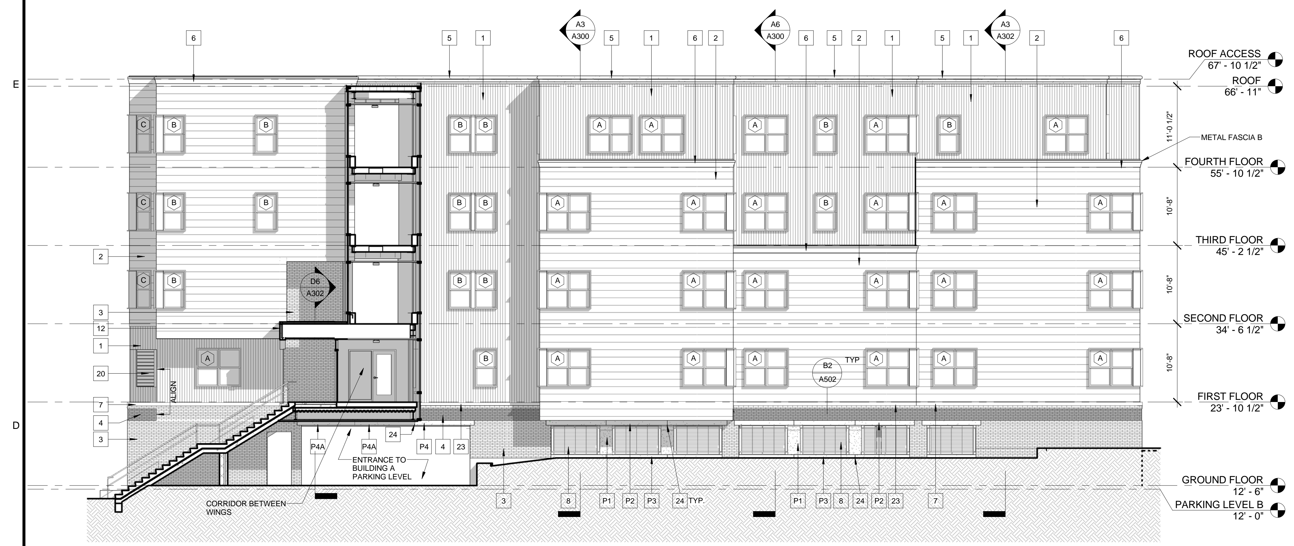
D6 EXTERIOR ELEVATION SOUTH A 1/8" = 1'-0"
