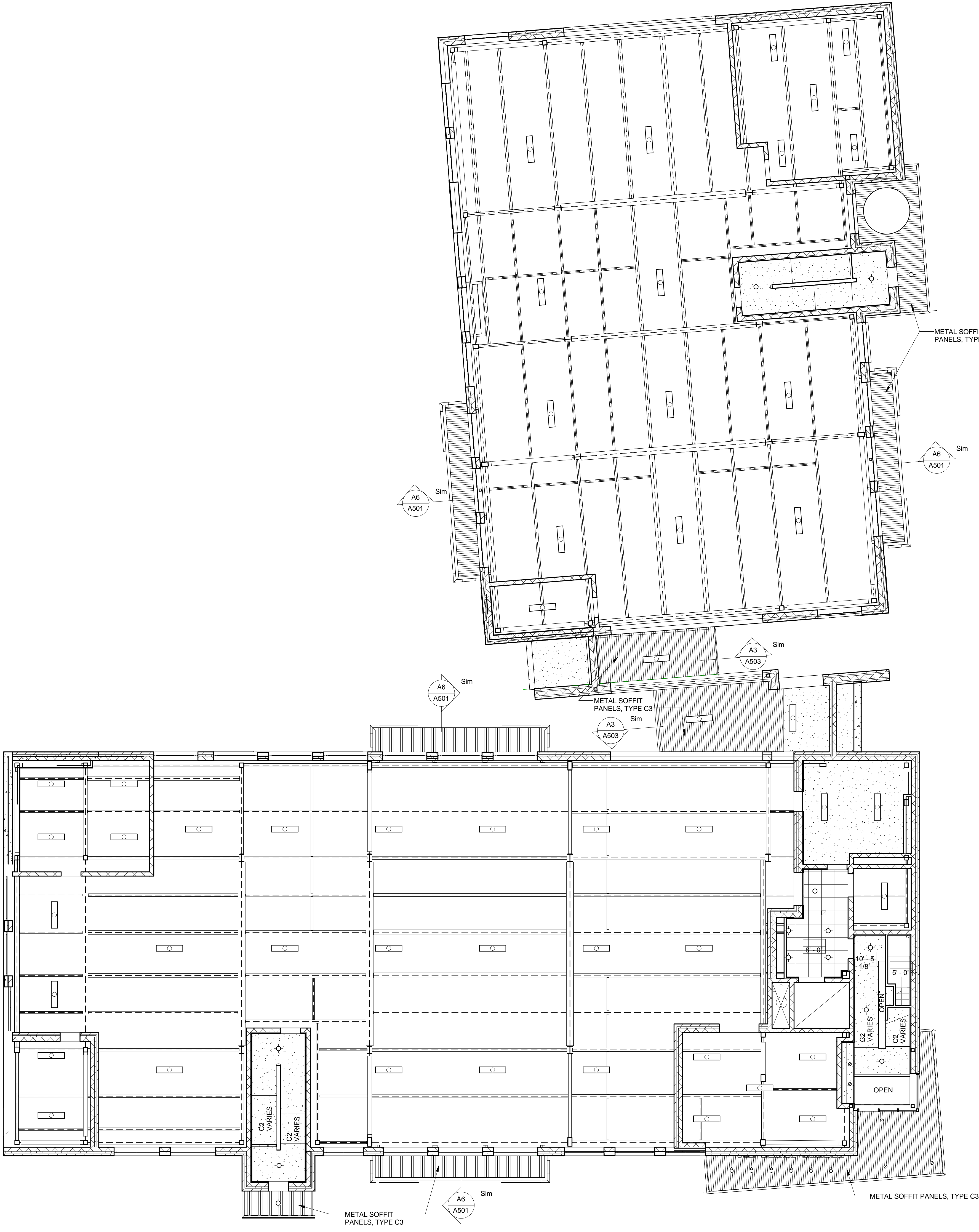
② PARKING CEILING PLAN 1/8" = 1'-0"
