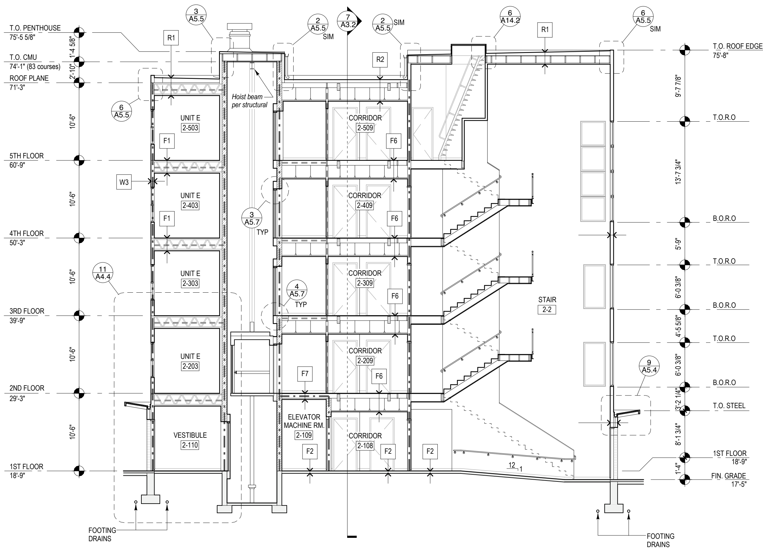
5 BUILDING SECTION 1/8" = 1'-0"
