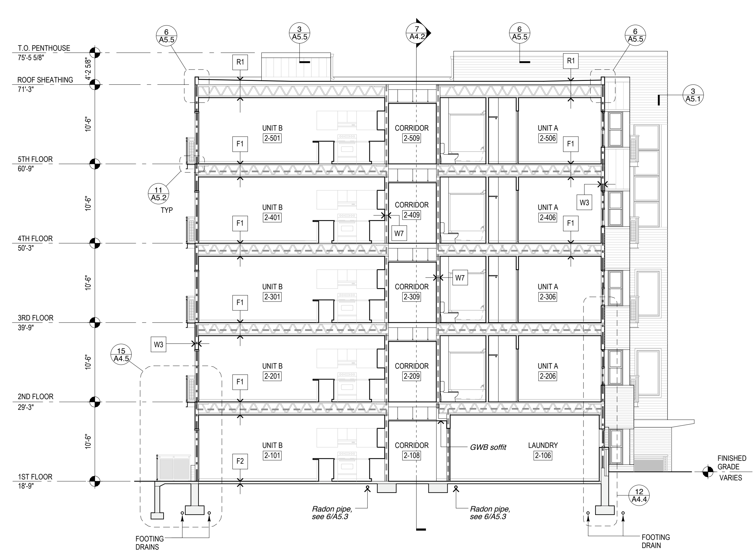
6 BUILDING SECTION 1/8" = 1'-0"
