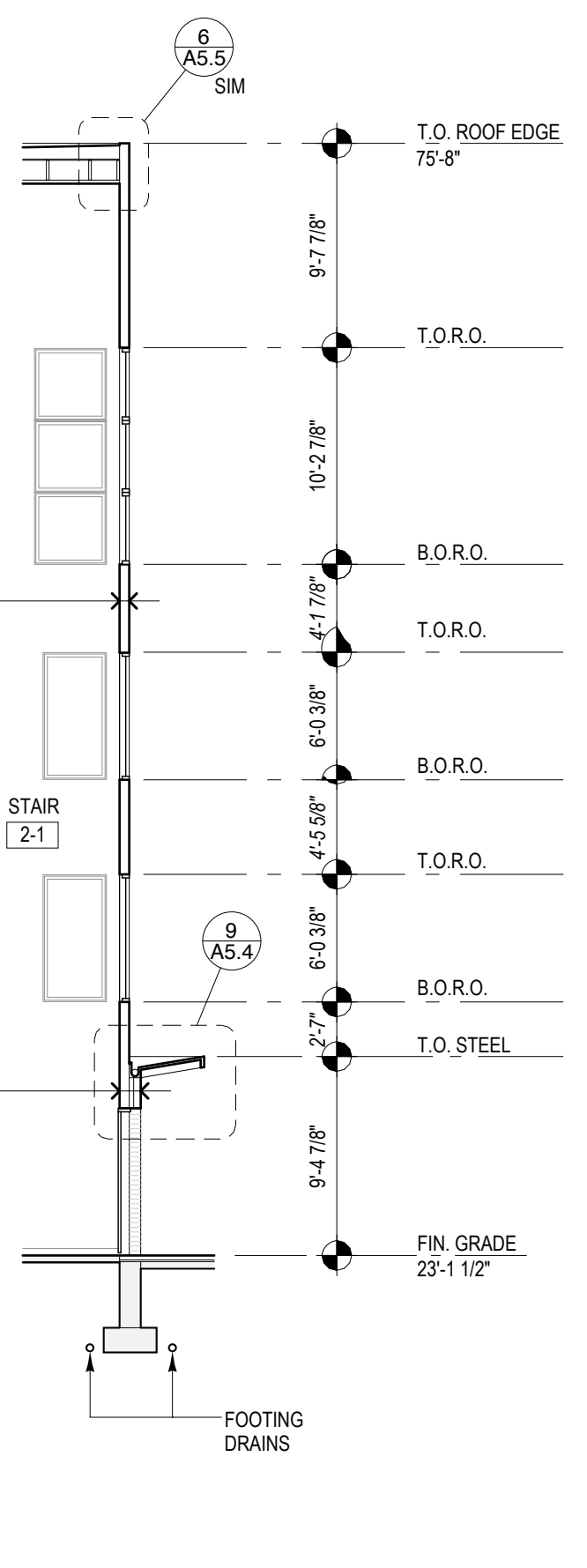
5A BUILDING SECTION 1/8" = 1'-0"
