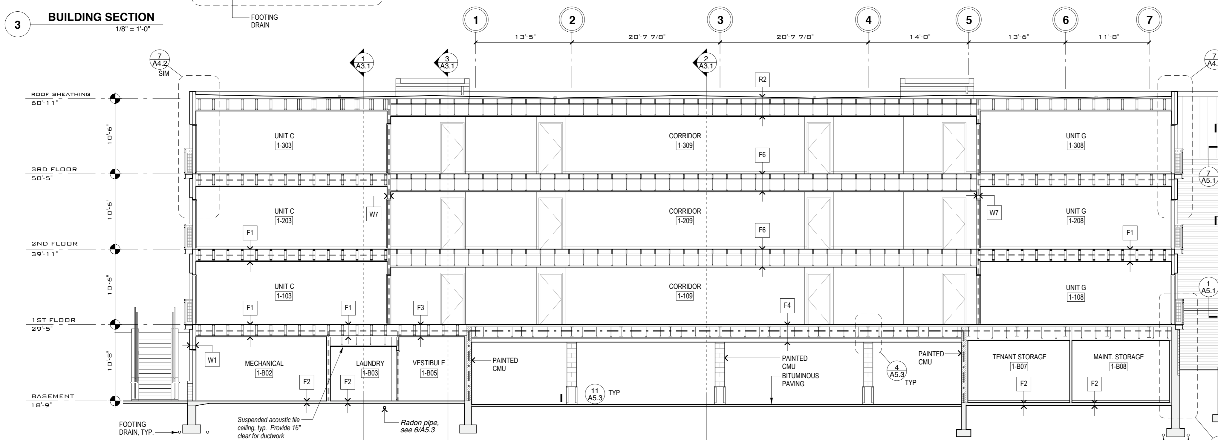
3 BUILDING SECTION 1/8" = 1'-0"
