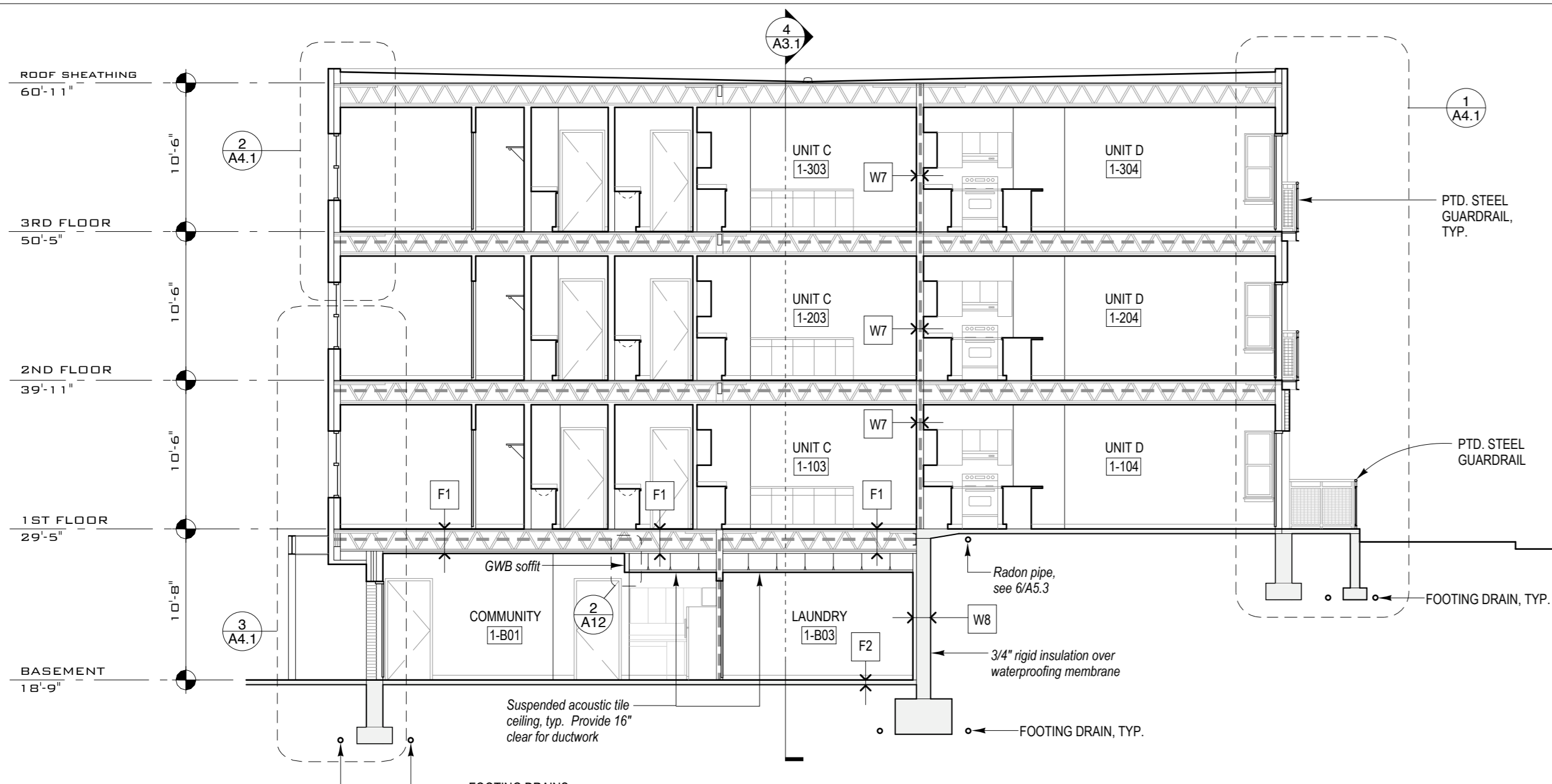
1 BUILDING SECTION 1/8" = 1'-0"
