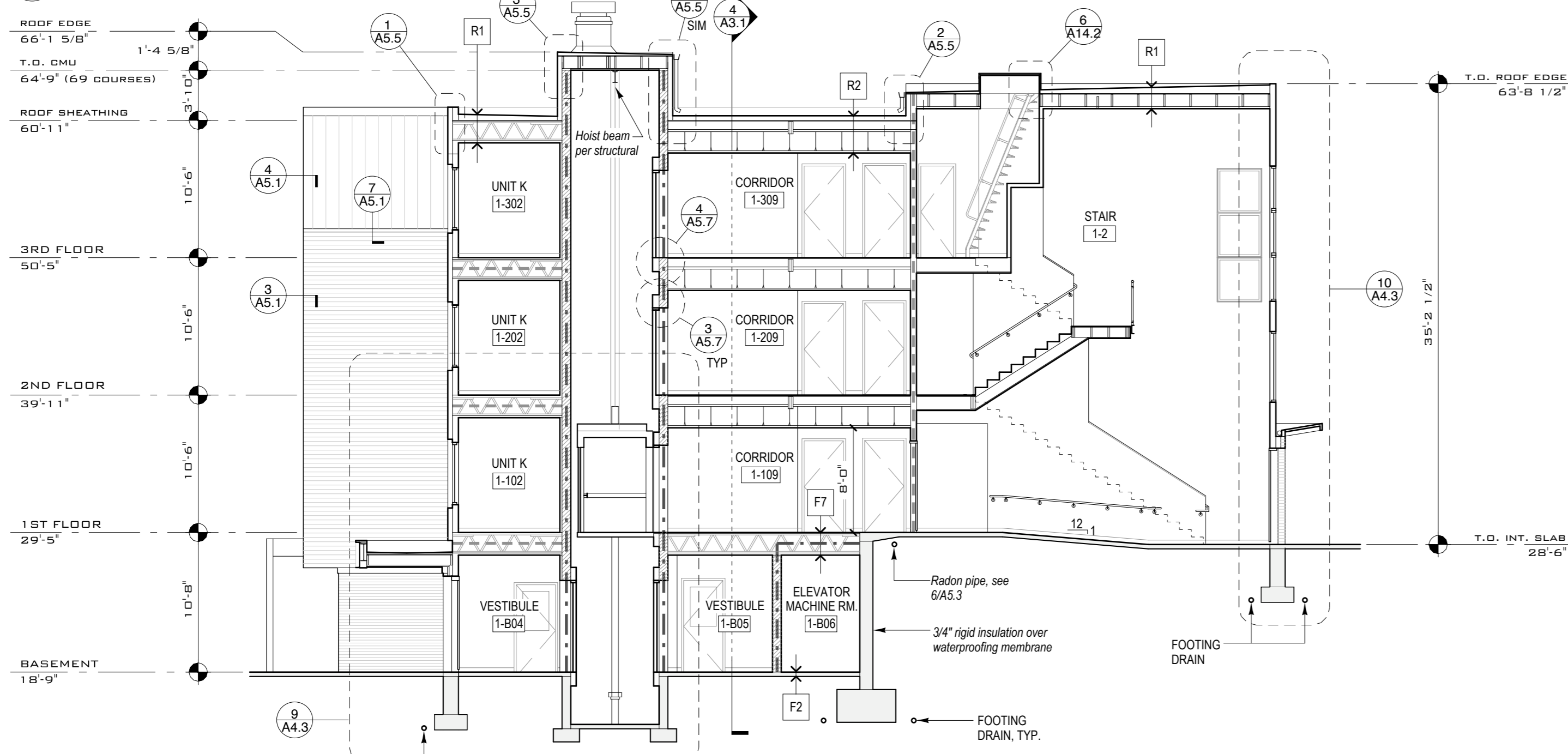
1 BUILDING SECTION 1/8" = 1'-0"
