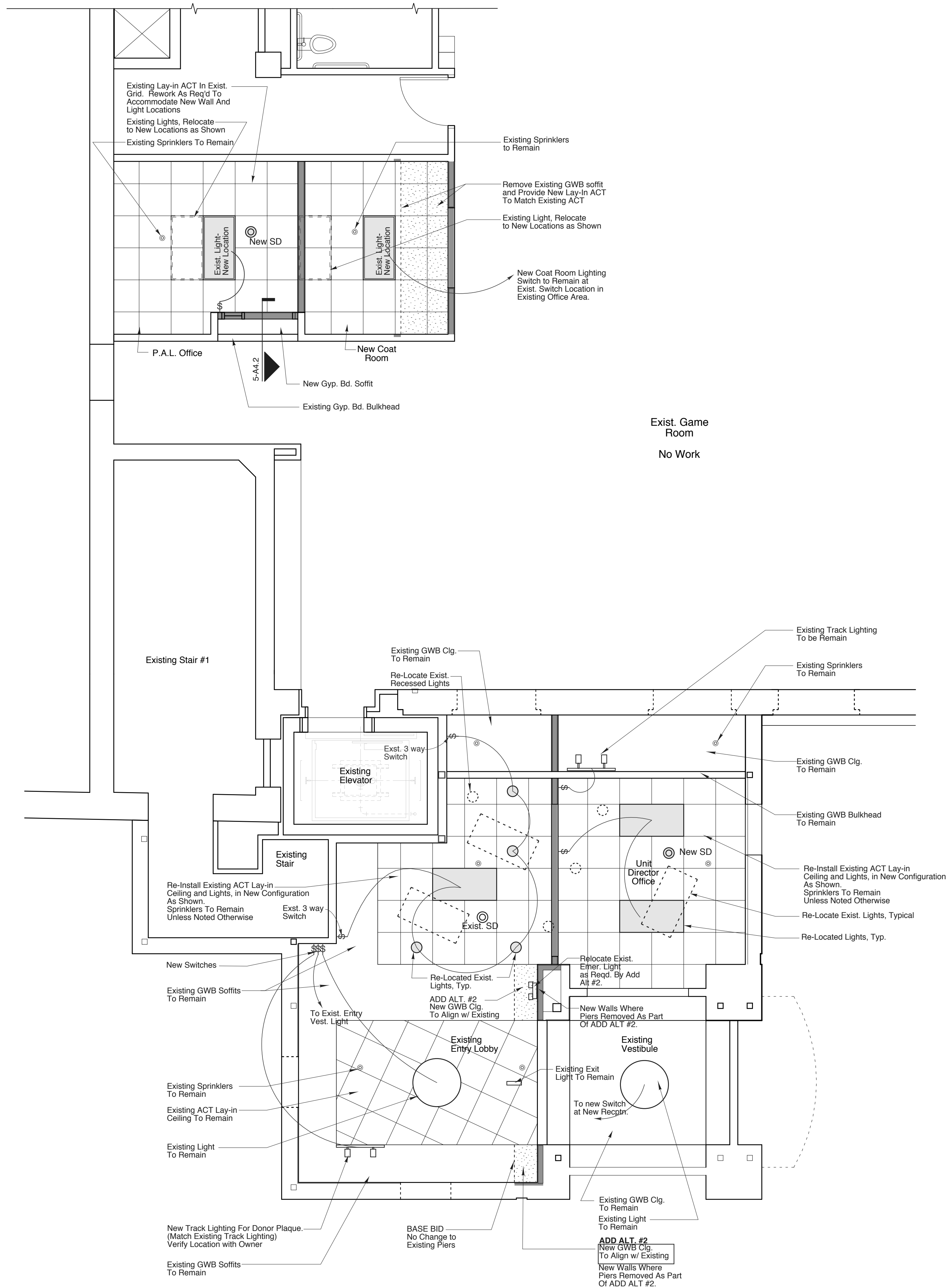
1 Proposed Reflected Ceiling Plan SCALE: 1/4" = 1'-0"
