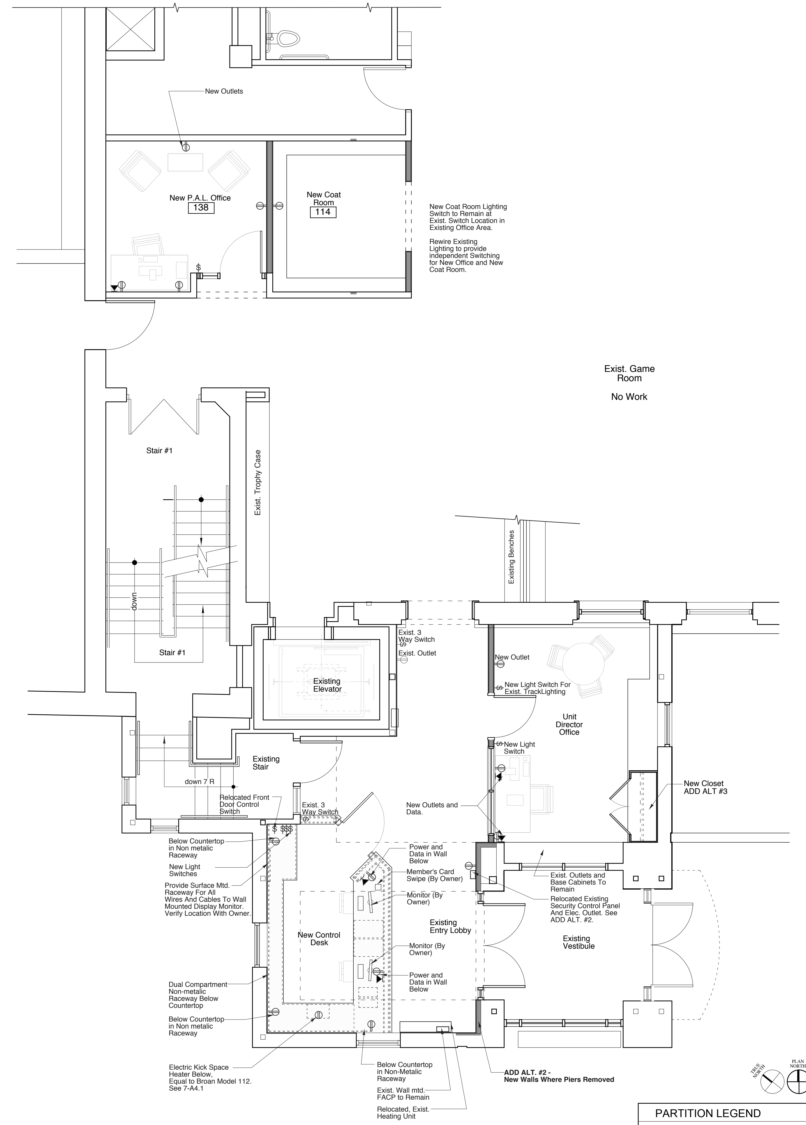
2 Proposed Electrical Plan SCALE: 1/4" = 1'-0"
