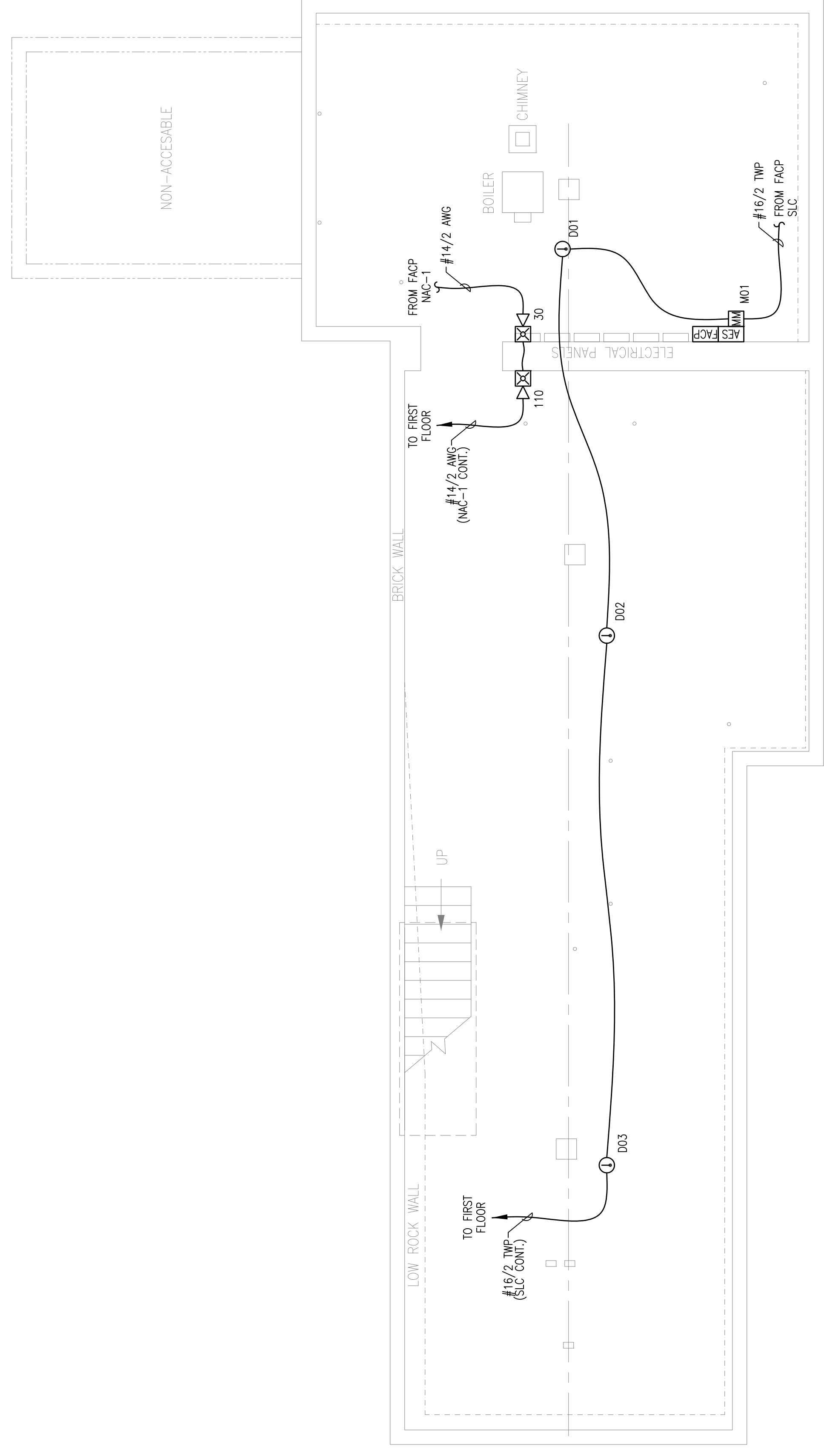
BASEMENT FIRE ALARM PLAN SCALE: 1/4"=1'-0"
