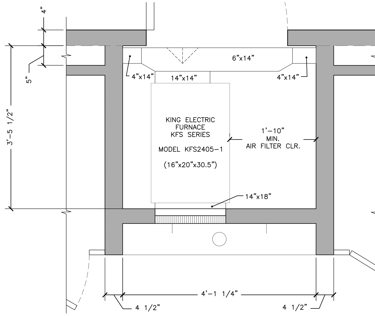
MECHANICAL ROOM (2) SCALE: 1" = 1'-0" (M1)
