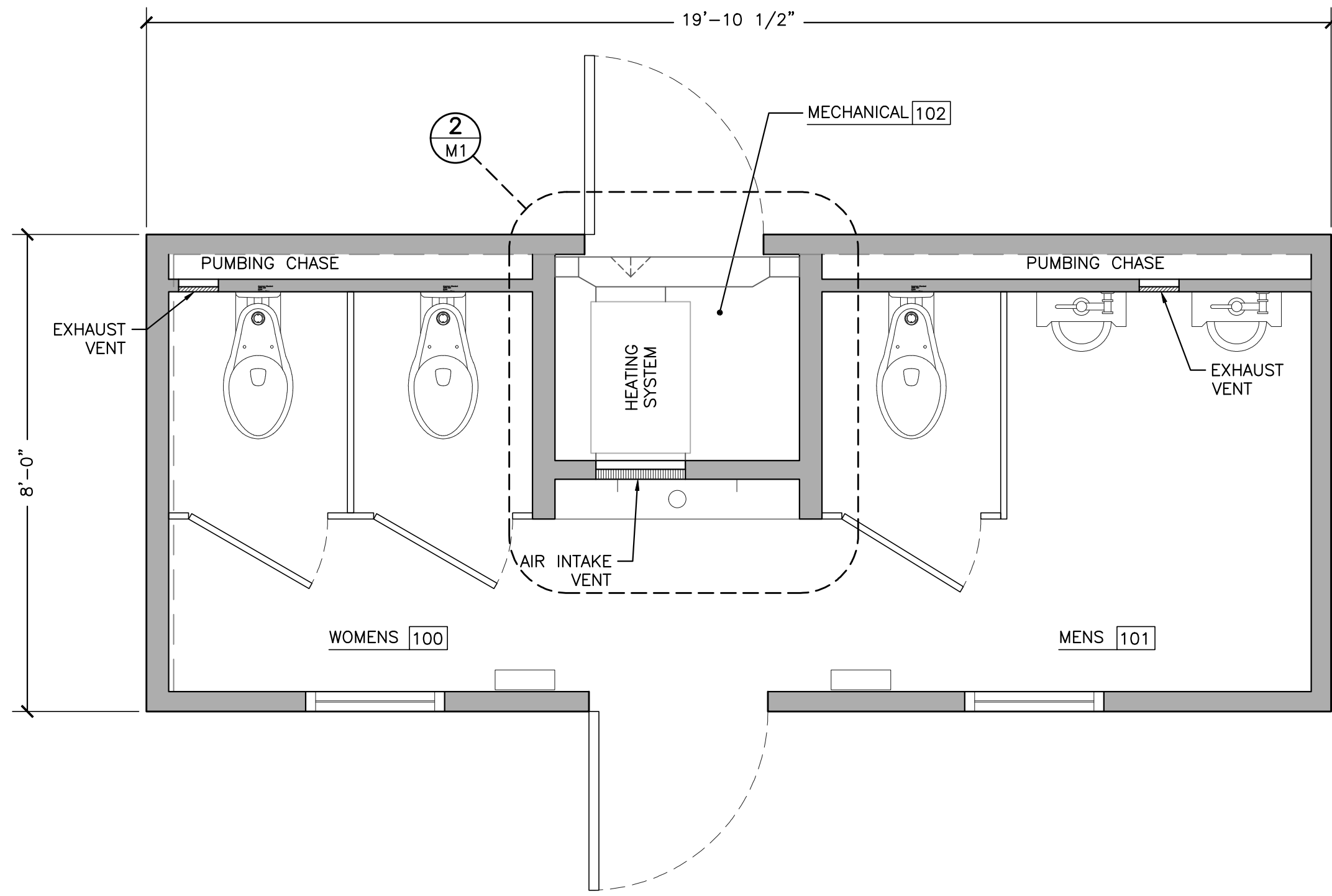
FLOOR PLAN (1) SCALE: 1/2" = 1'-0" (M1)
