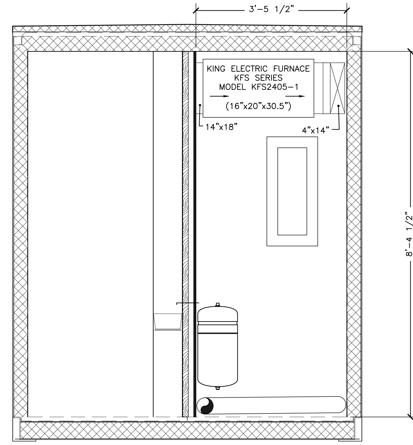
MECHANICAL ROOM (3) SCALE: 3/4" = 1'-0" (M1)
