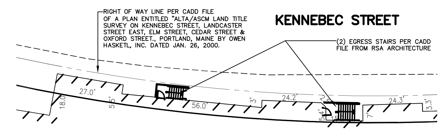
DETAIL AT KENNEBEC STREET SCALE: 1" = 20'
