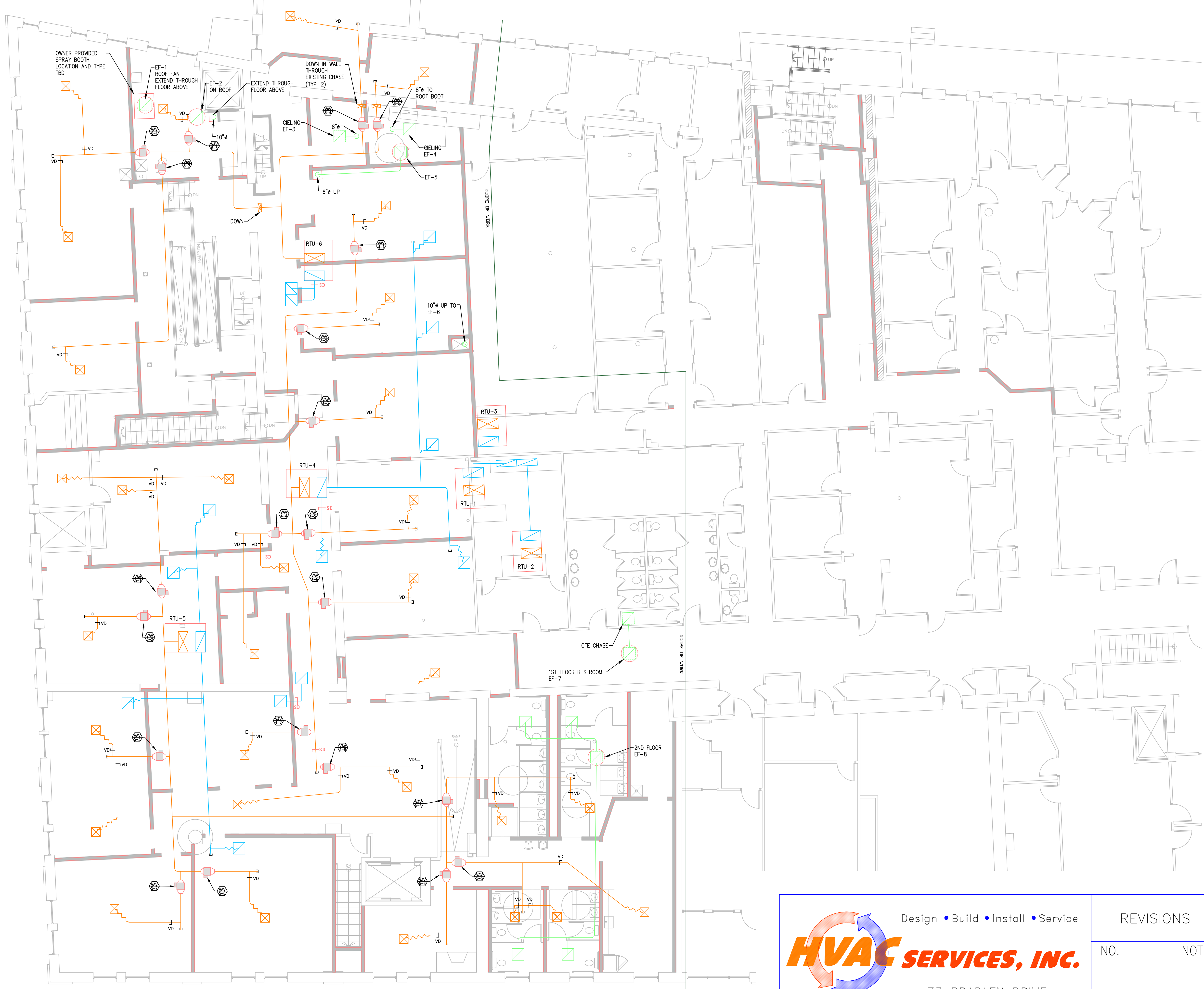
SECOND FLOOR - DUCTWORK SCALE: 1/8"=1'-0"
