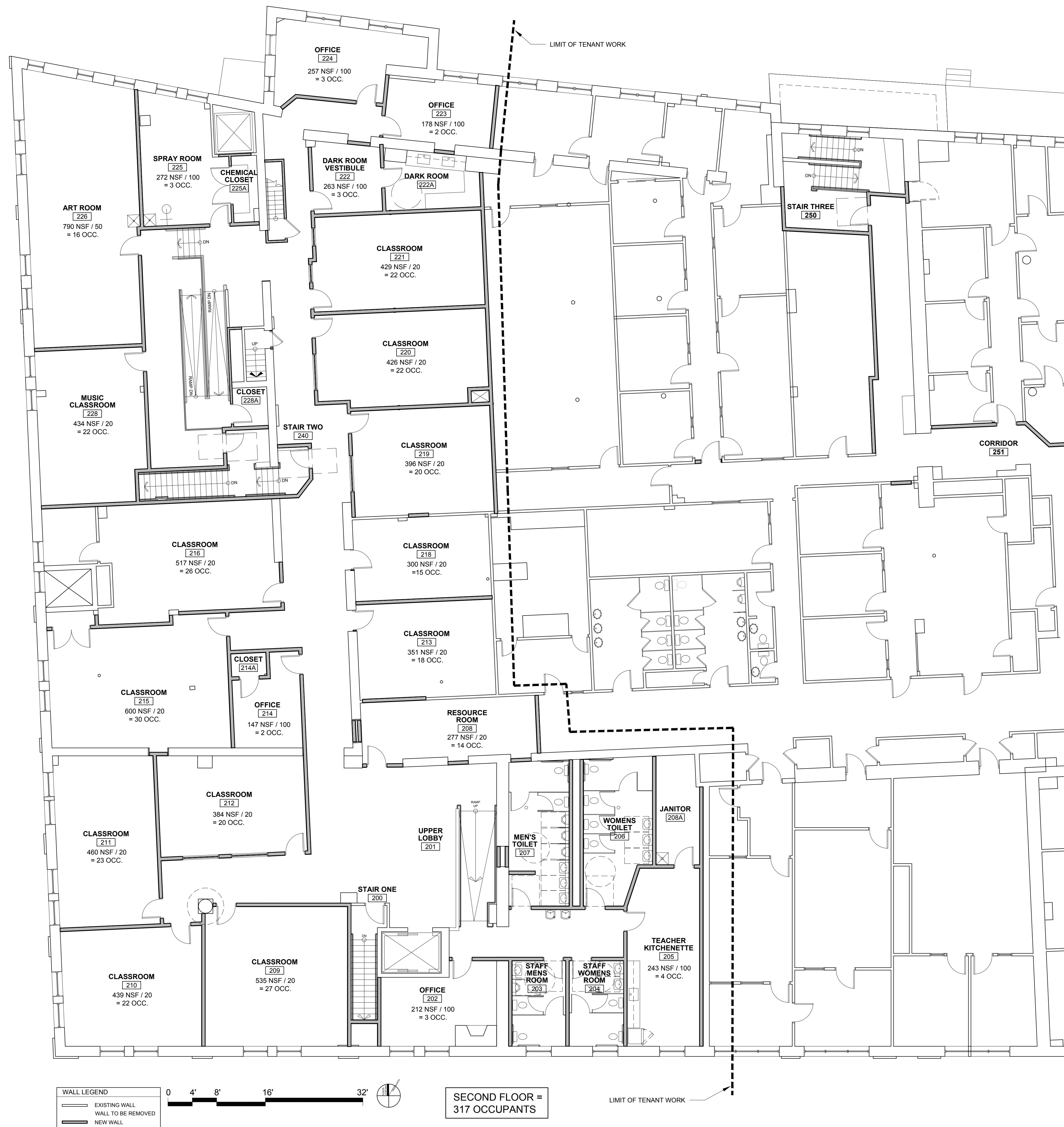
1 SECOND FLOOR OCCUPANT LOAD PLAN 1/8" = 1'-0"
