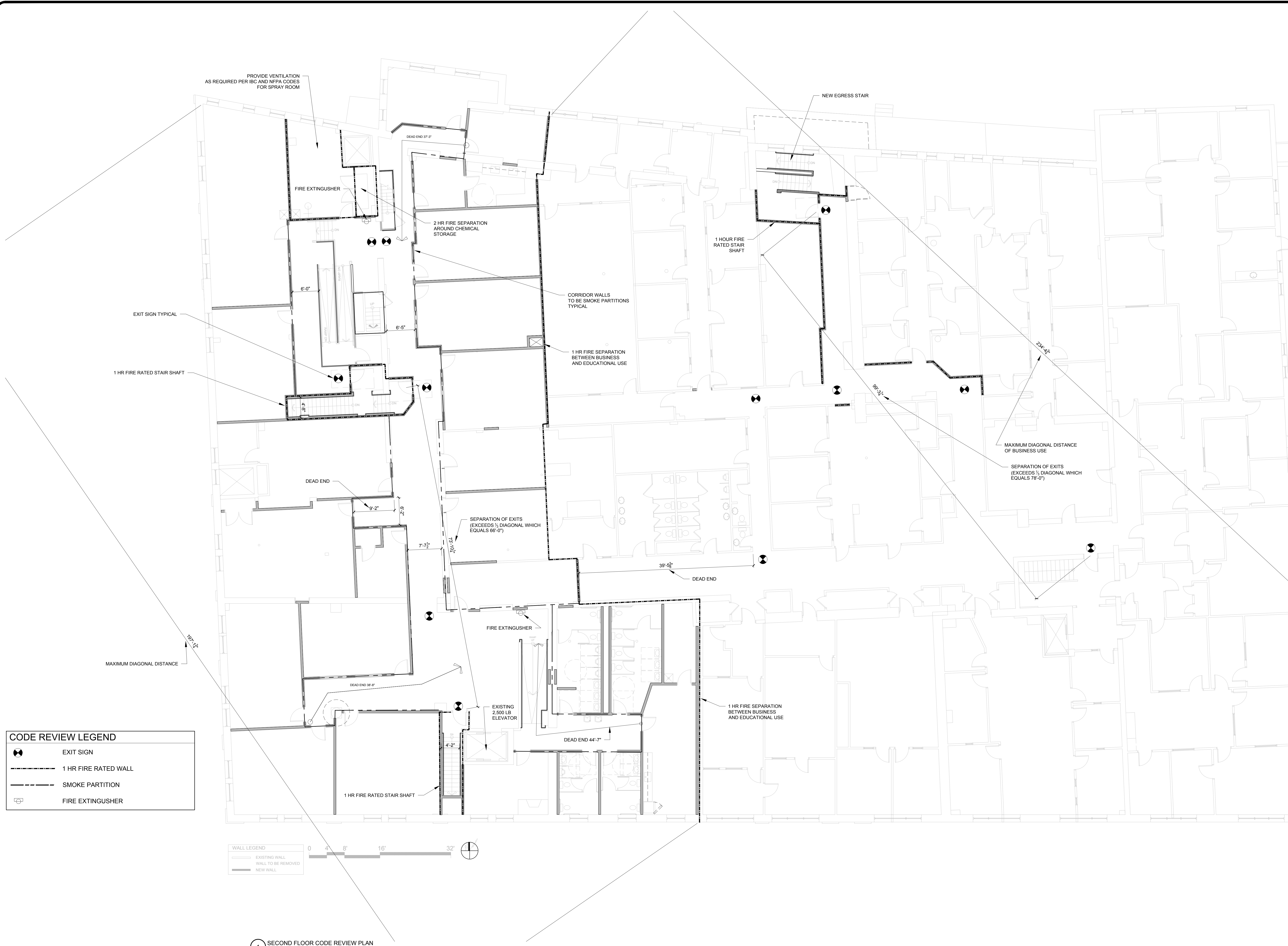
1 SECOND FLOOR CODE REVIEW PLAN
