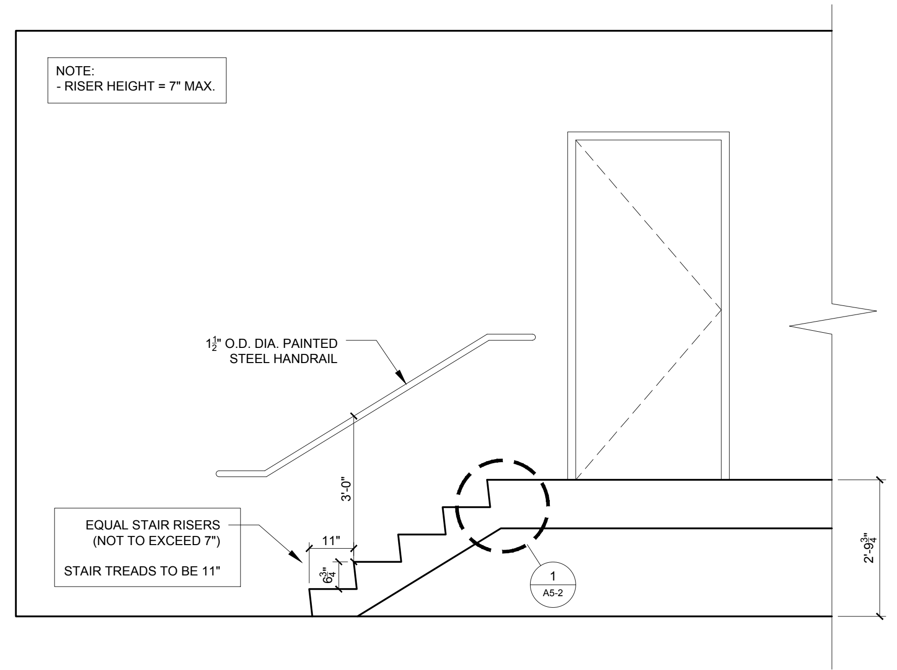
3 SECTION THROUGH STAIR AT END OF RAMP 1/2" = 1'-0"
