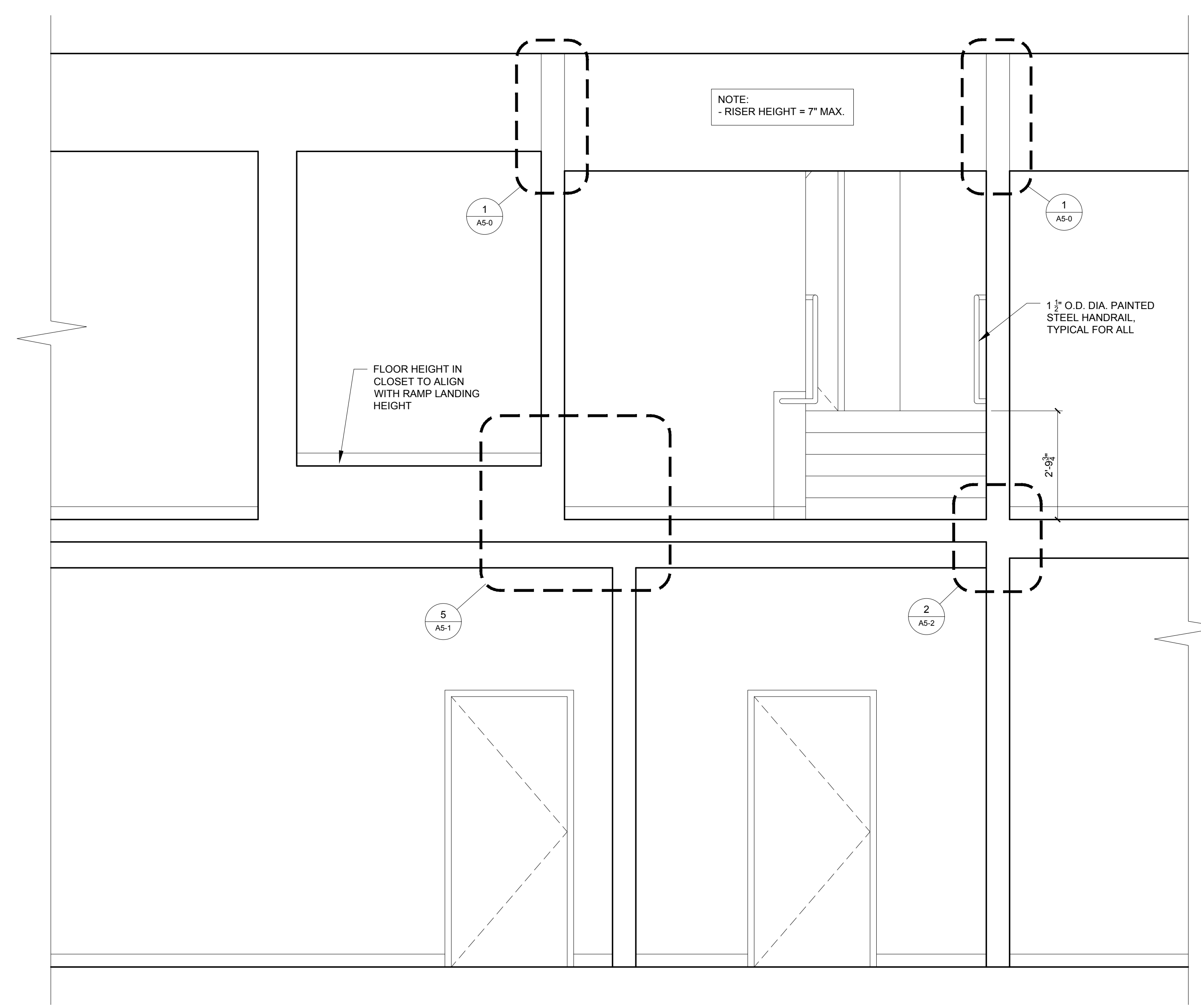
2 SECTION THROUGH STAIR 1/2" = 1'-0"
