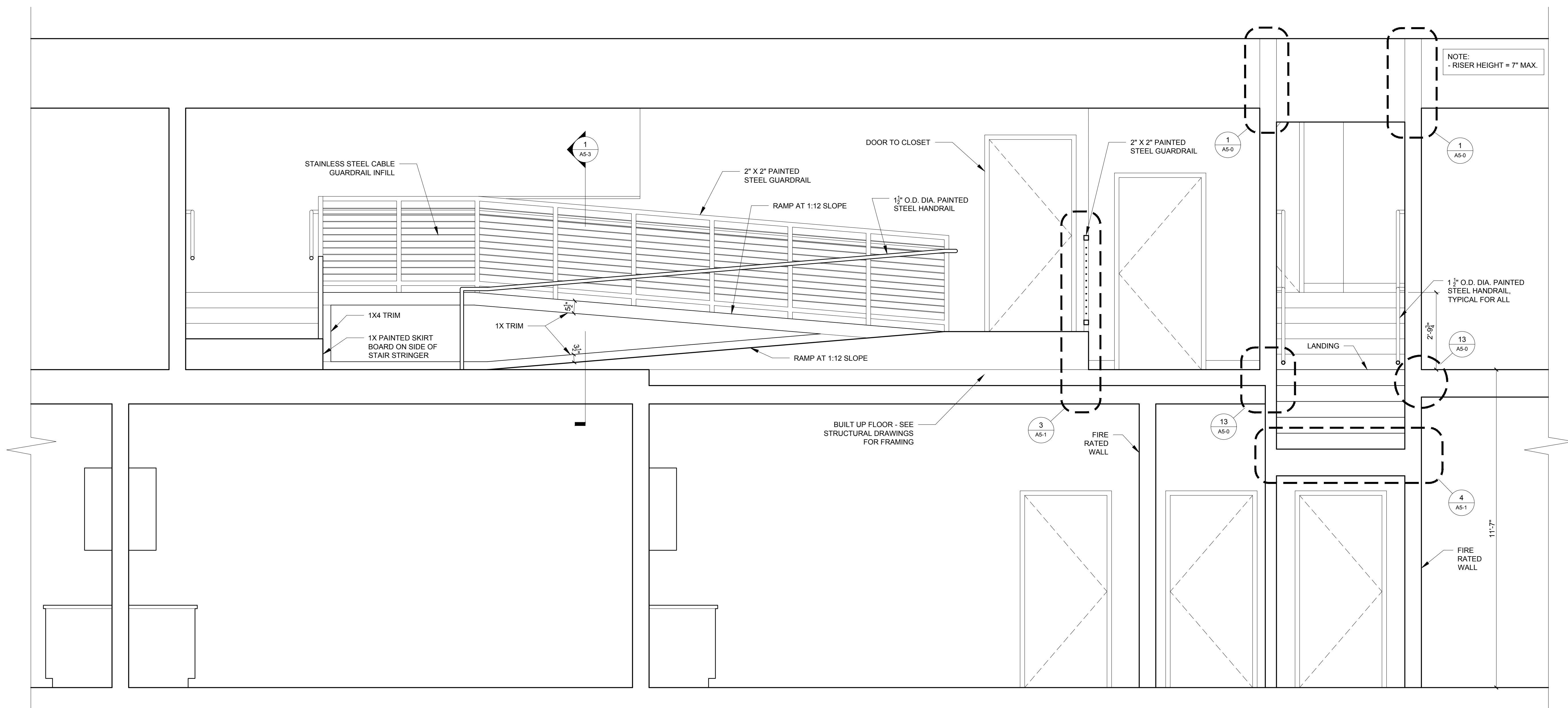
1 SECTION THROUGH STAIR 1/2" = 1'-0"
