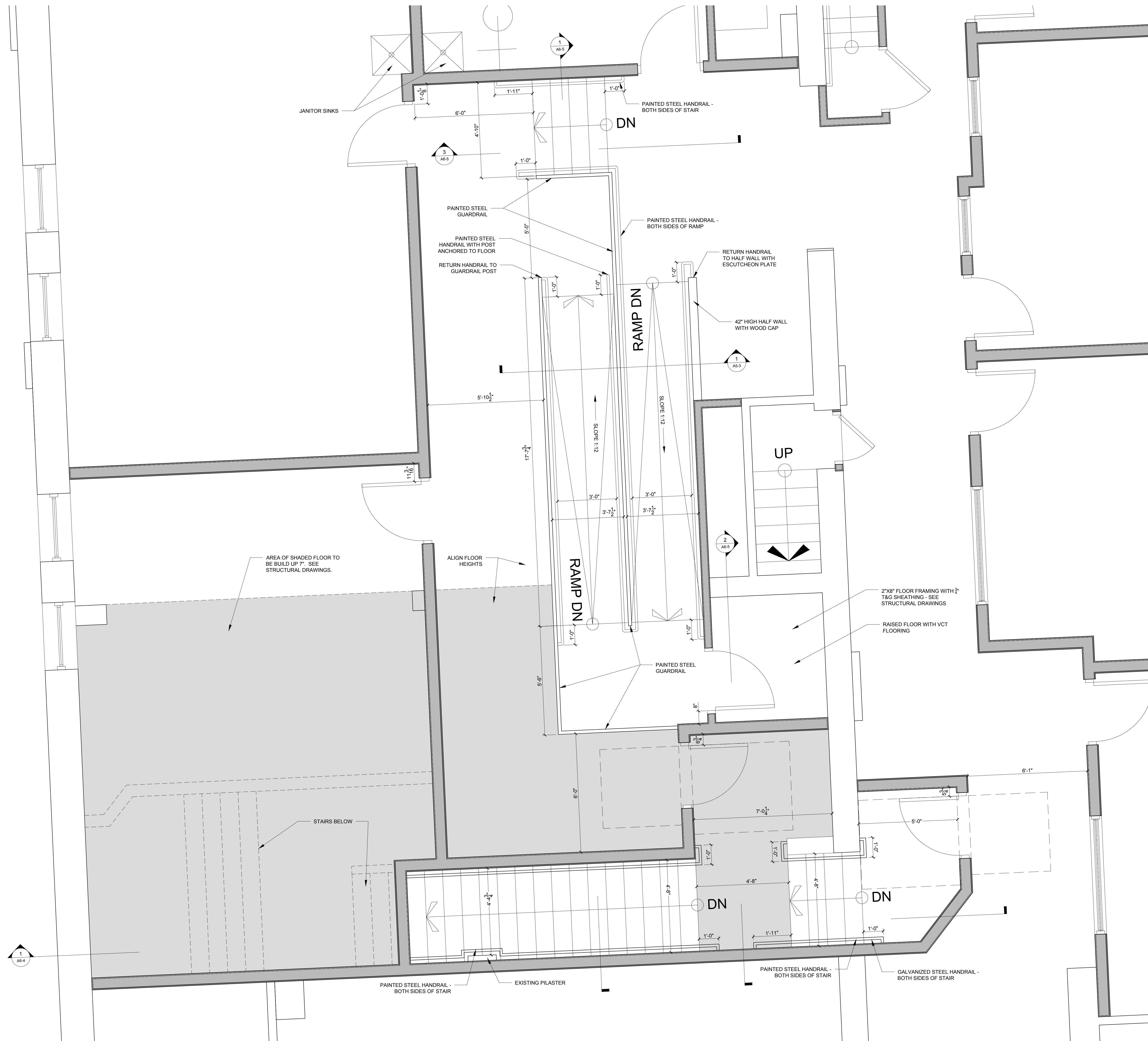
1 STAIR TWO 240 1/2" = 1'-0"
