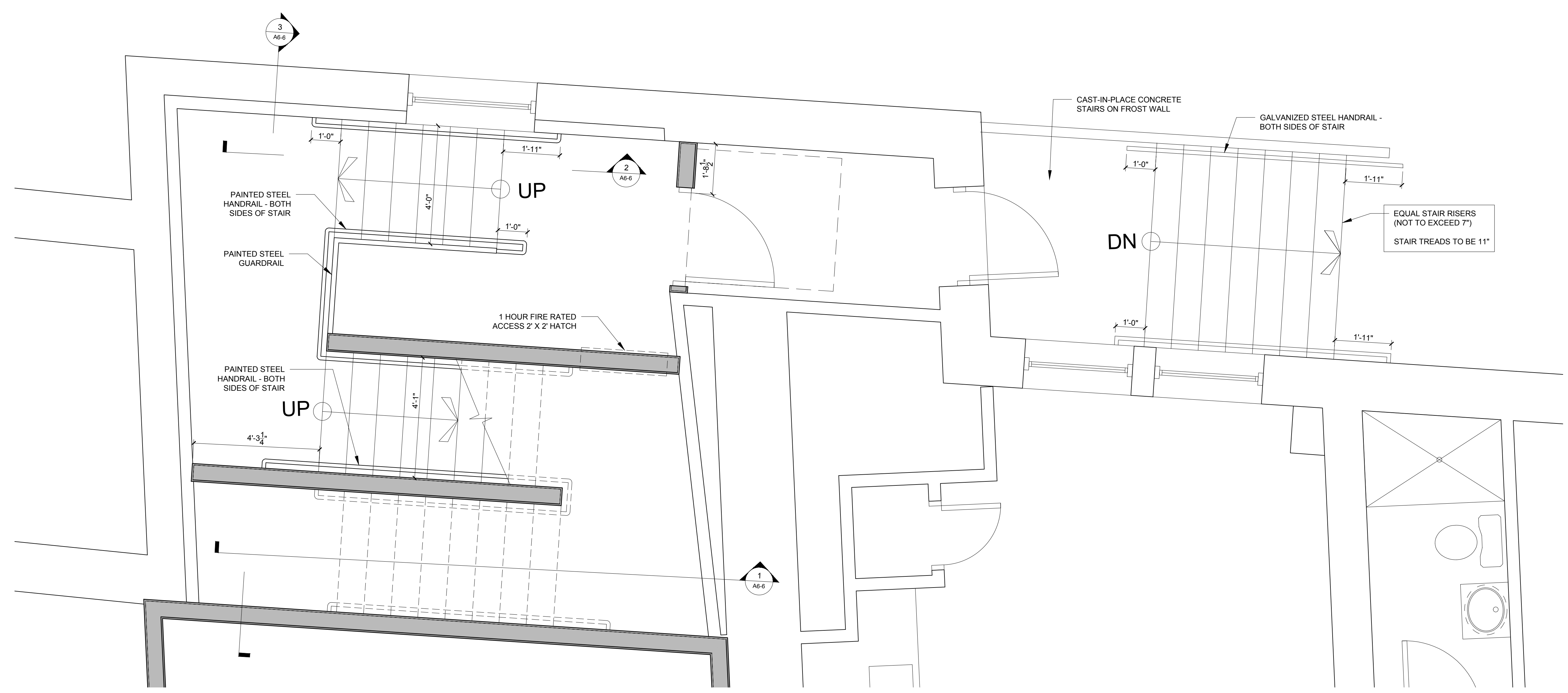
2 NORTH STAIR PLAN 1/2" = 1'-0"
