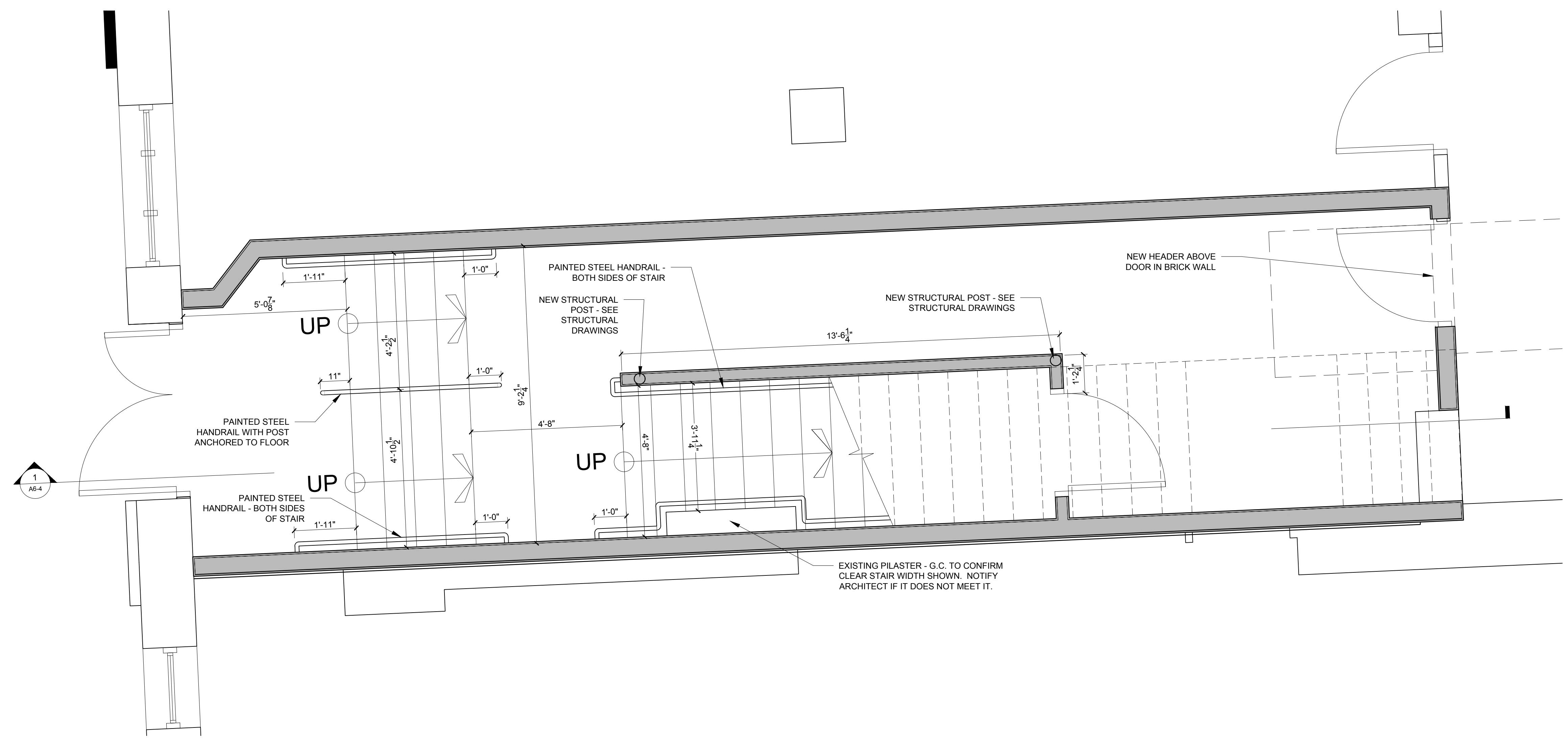
1 STAIR TWO (140) PLAN 1/2" = 1'-0"
