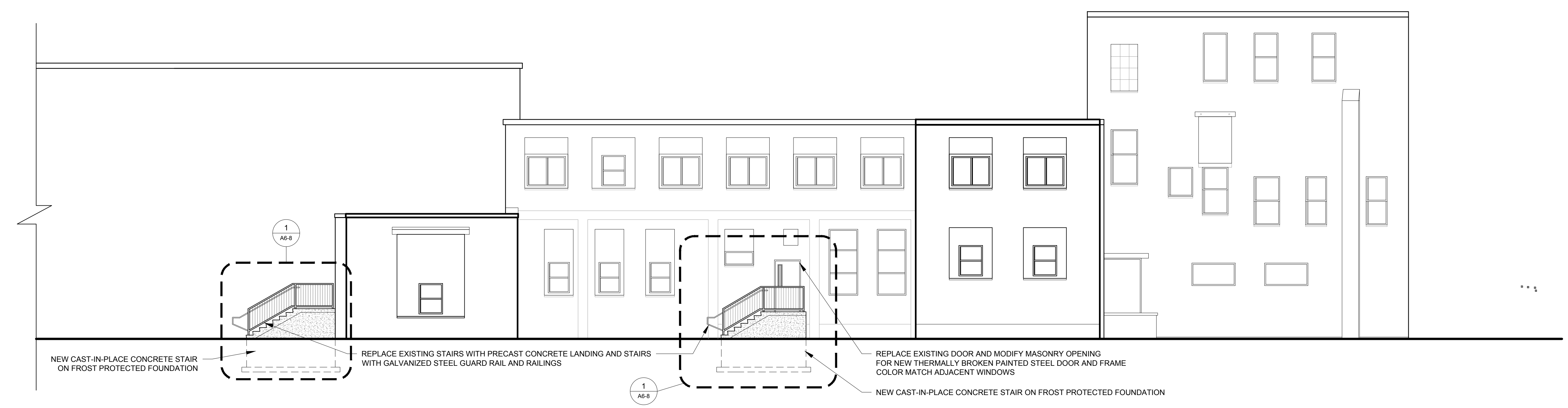
1 KENNEBEC STREET ELEVATION 1/8" = 1'-0"
