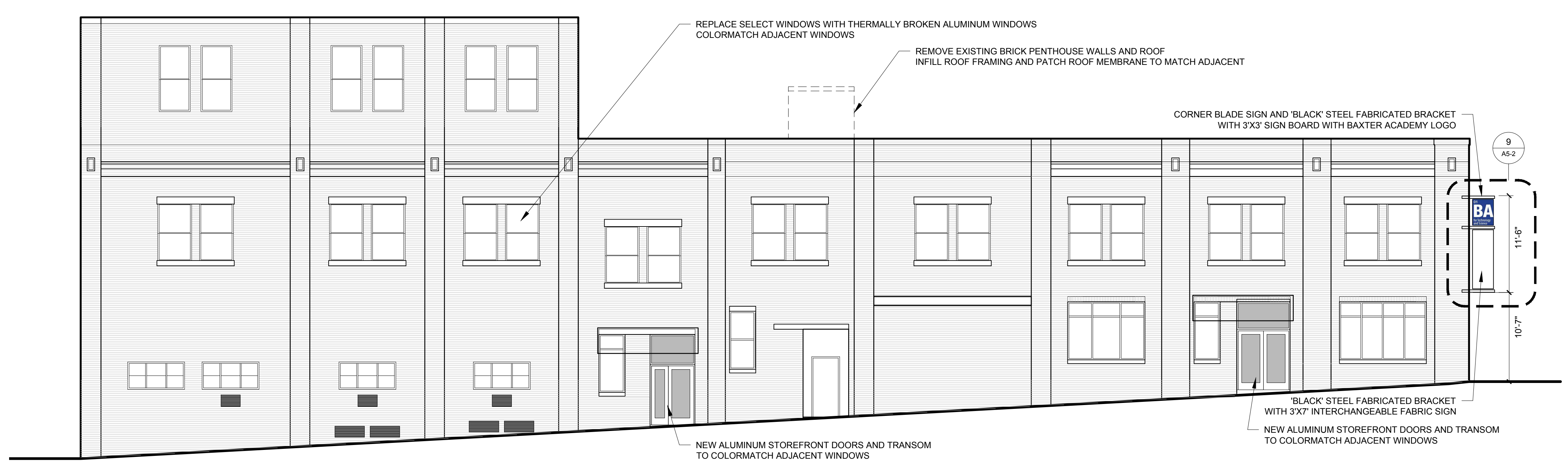
2 ELM STREET ELEVATION 1/8" = 1'-0"
