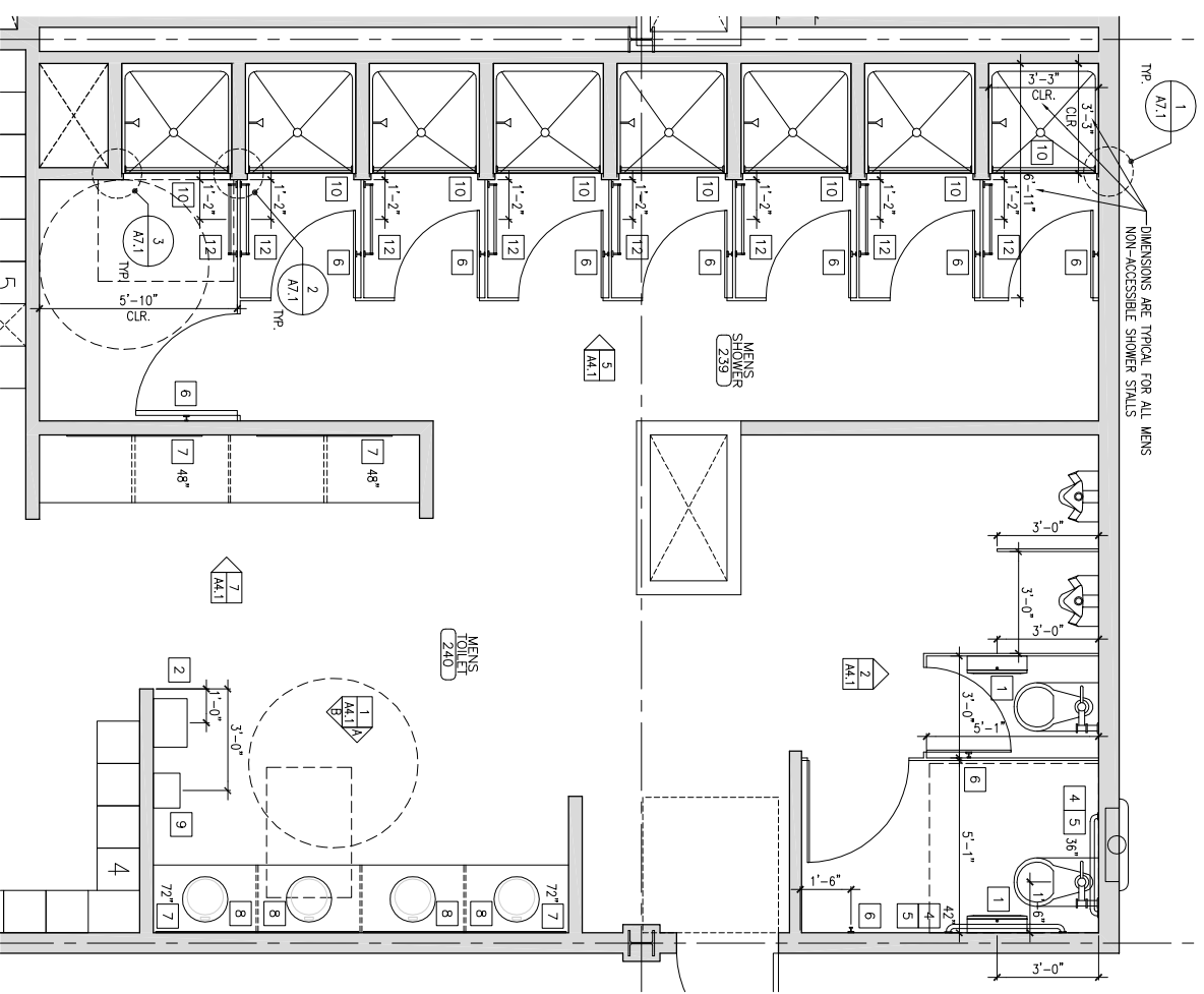
8 ENLARGED PLAN @ MENS SHOWER/TOILET ROOM
