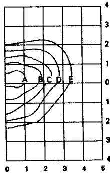
GM-6 GMA401292D 400-Watt MH Type II 40,000-Lumen Clear Lamp
