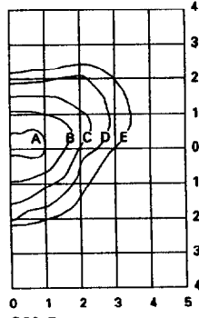
GM-7 GMA401293D 400-Watt MH Type III 40,000-Lumen Clear Lamp
