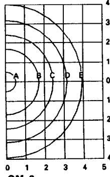
GM-8 GMA40129AR 400-Watt MH Area Round 40,000-Lumen Clear Lamp
