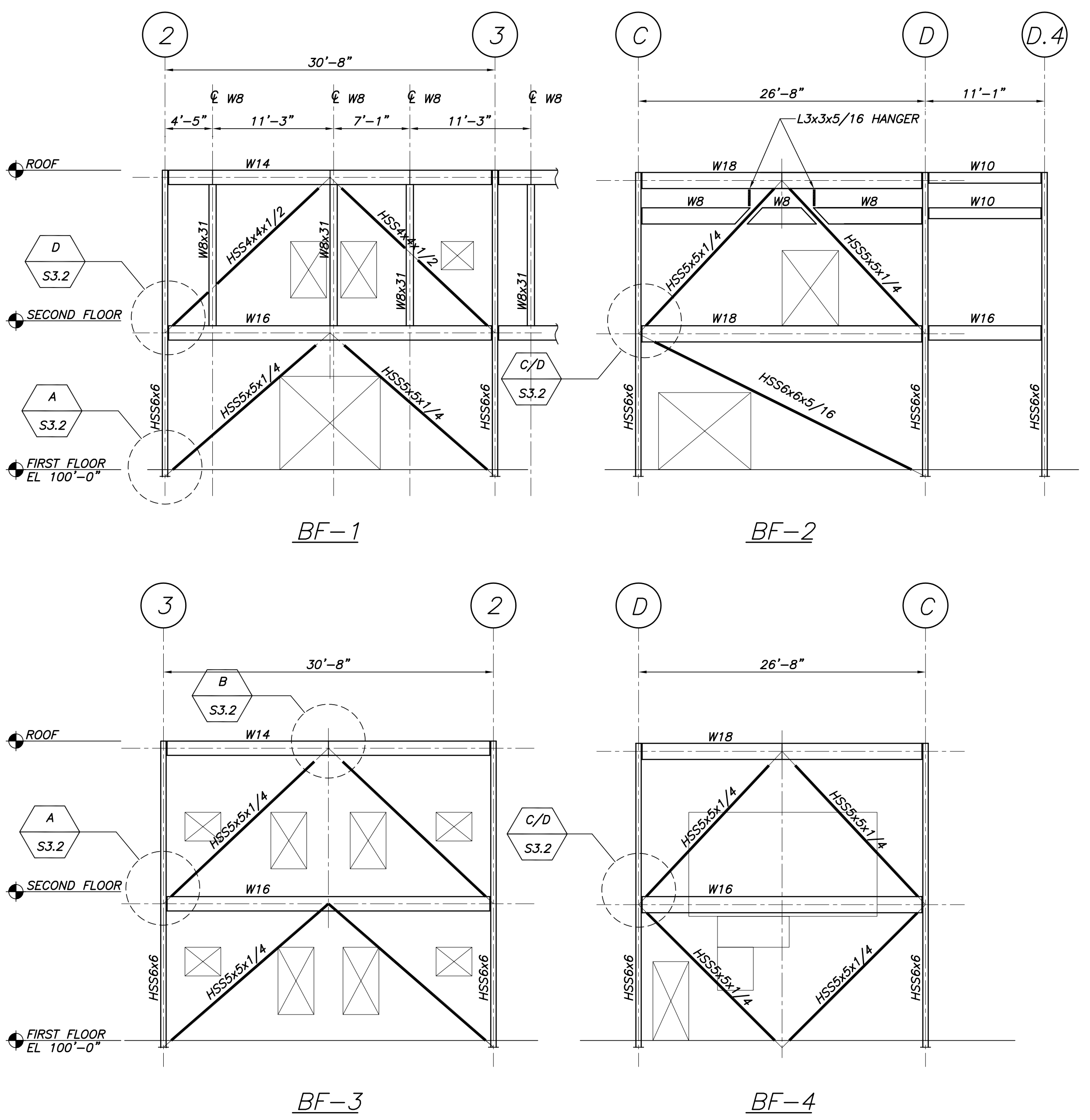
BRACING ELEVATIONS 1/8"=1'-0"
