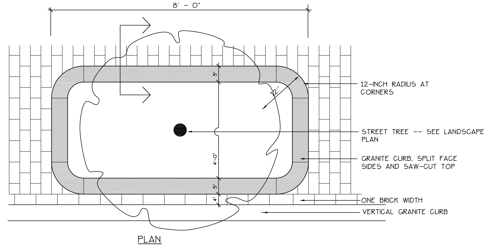
4 STREET TREE RAISED PLANTING BED L2.0 NOT TO SCALE
