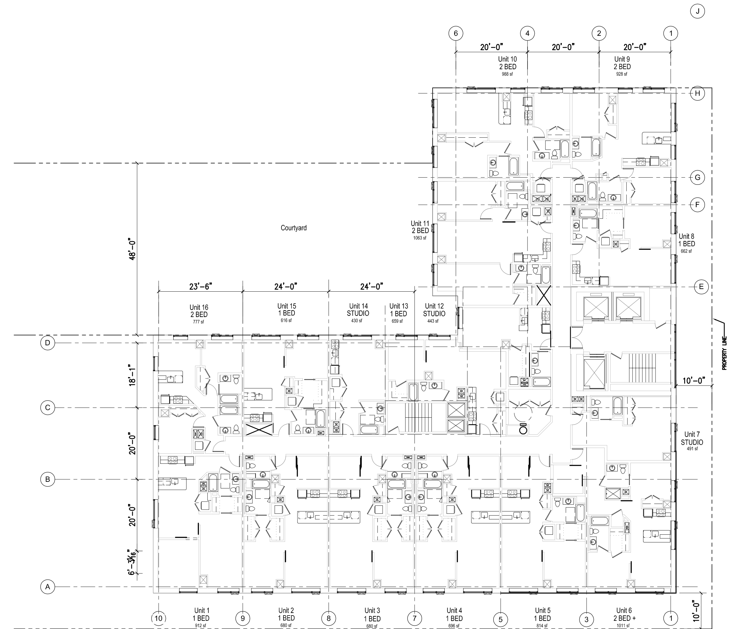
1 TYPICAL FLOOR PLAN SCALE: 1/16" = 1'-0"
