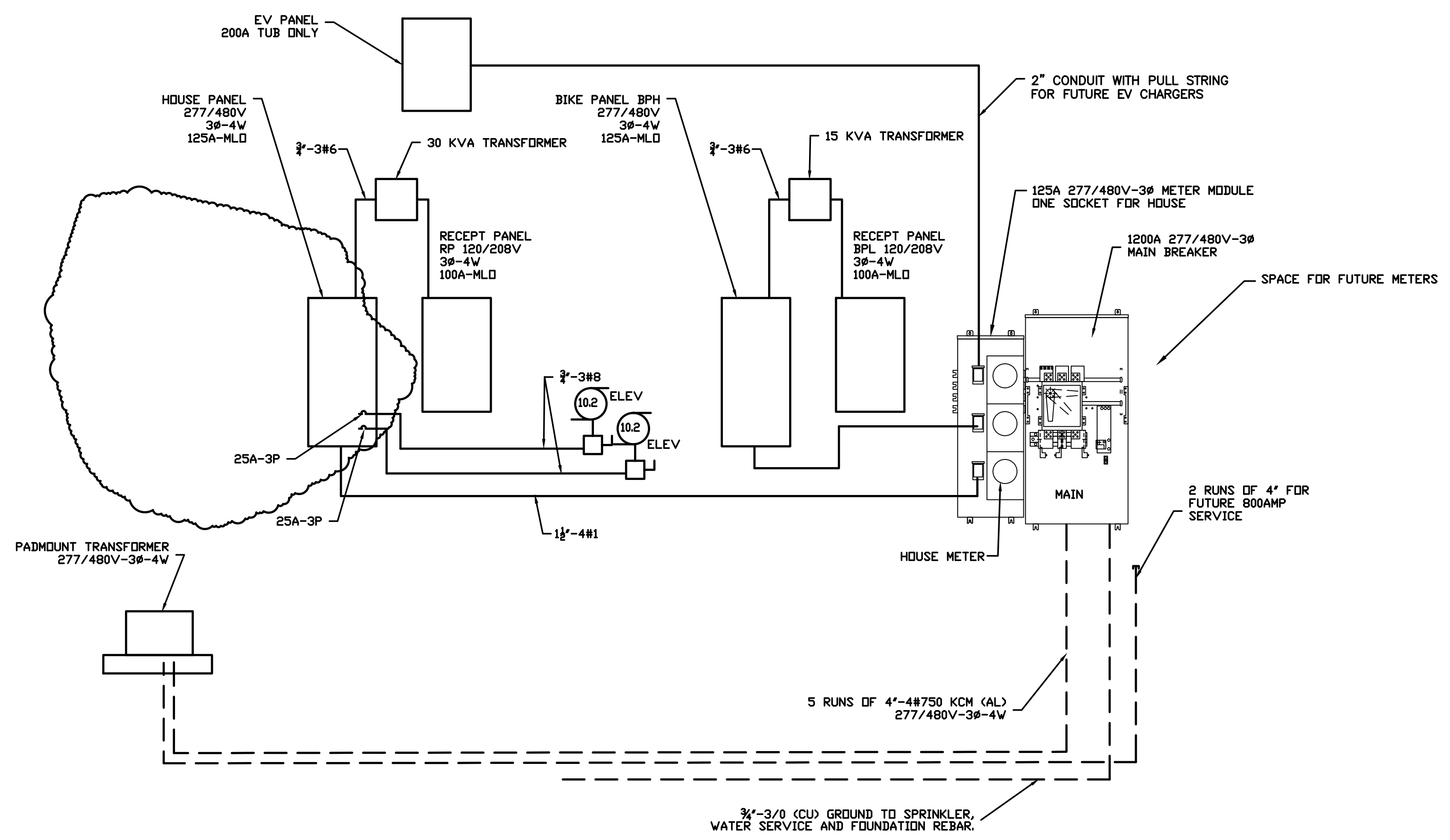
ONE LINE DIAGRAM
